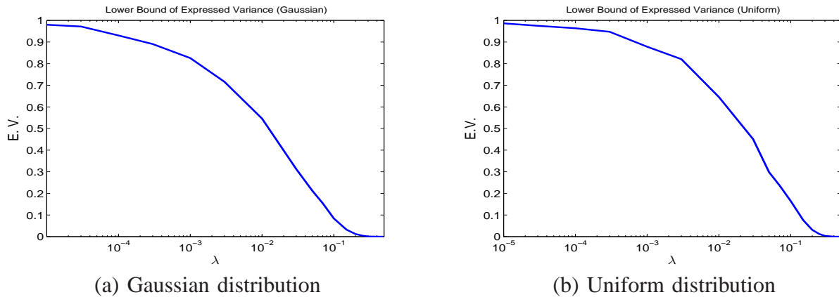
Fig. 1. This figure shows the lower bounds on the asymptotic performance of HR-PCA, under Gaussian and Uniform distribution for \mathbf{x} .
