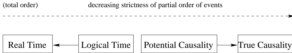
Figure 4.1: Spectrum of models
