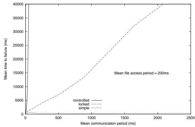
Figure 5.4: Plotting mttf against mean comm. period on a linear scale
