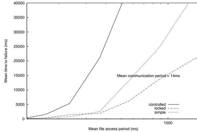
Figure 5.5: Plotting mttf against mean file access period
