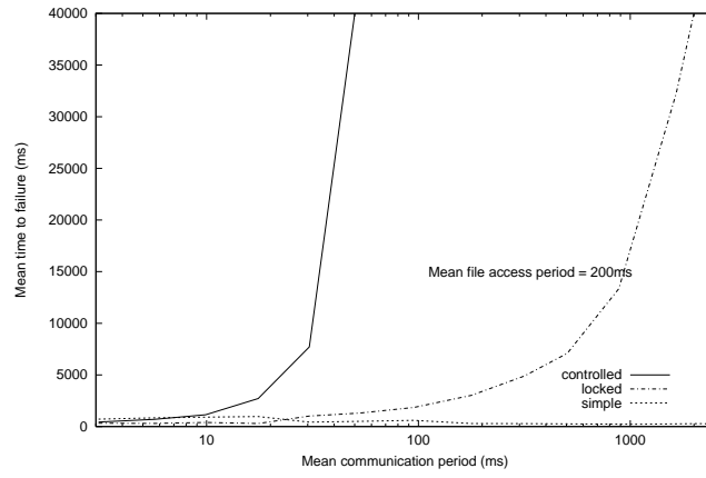
Figure 5.3: Plotting mttf against mean comm. period
