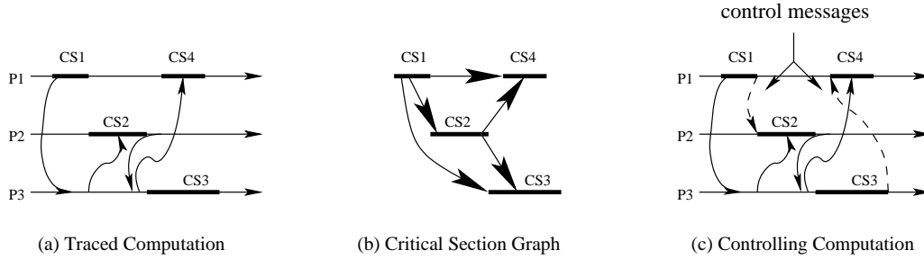
Figure 5.2: Controlled Re-execution
