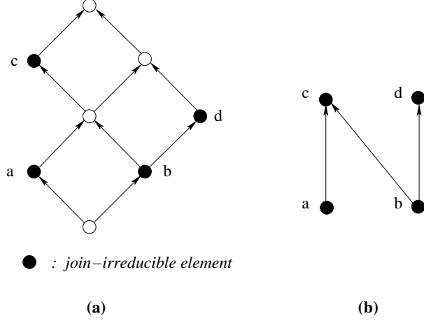
Figure 3: (a) An example of a distributive lattice (b) its partial order representation.
