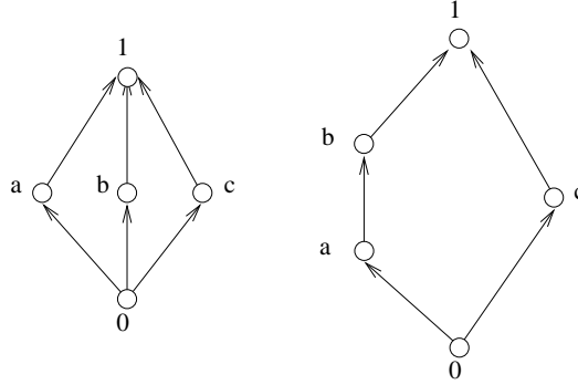
Figure 2: Examples of nondistributive lattices
