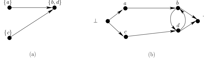
Figure 6: (a) A slice depicting the events that are to be executed atomically, and (b) the graph representation of the slice in (a).
