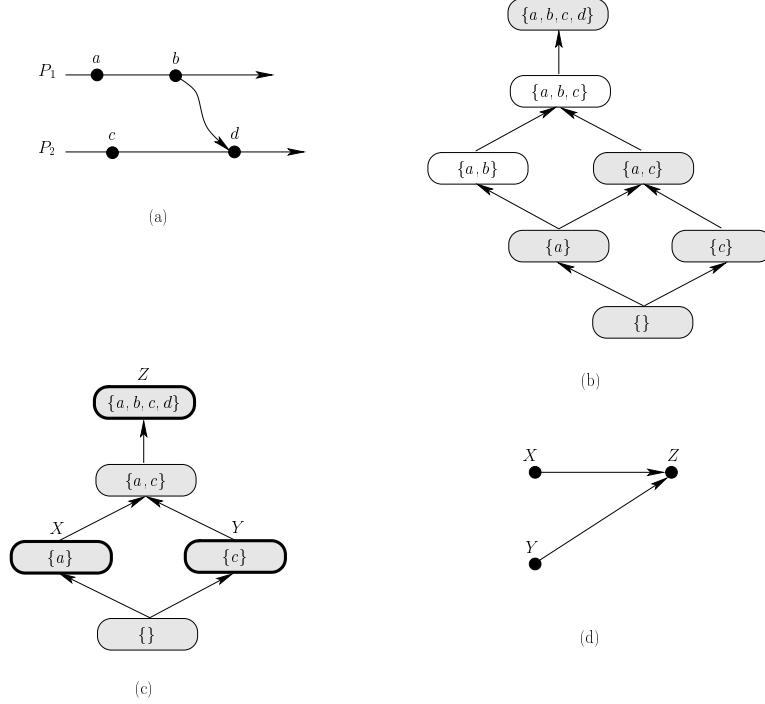
Figure 5: (a) A distributed computation, (b) the distributive lattice generated by its consistent cuts, (c) the sublattice containing all consistent cuts for which no messages are in transit, and (d) the poset induced on the set of join-irreducible elements of the sublattice.
