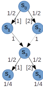
Figure 5: State-space graph that is not acyclic. JPF explores three paths: p_1 : \langle s_0, s_1, s_3, s_4 \rangle ; p_2 : \langle s_0, s_1, s_3, s_5 \rangle ; and p_3 : \langle s_0, s_2, s_3 \rangle . JPFBar calculates the following weights for them: p_1 : \frac{1}{4} ; p_2 : \frac{1}{4} ; and p_3 : \frac{1}{2} . The weights add up to 1 and represent 100% progress when JPF search terminates.
