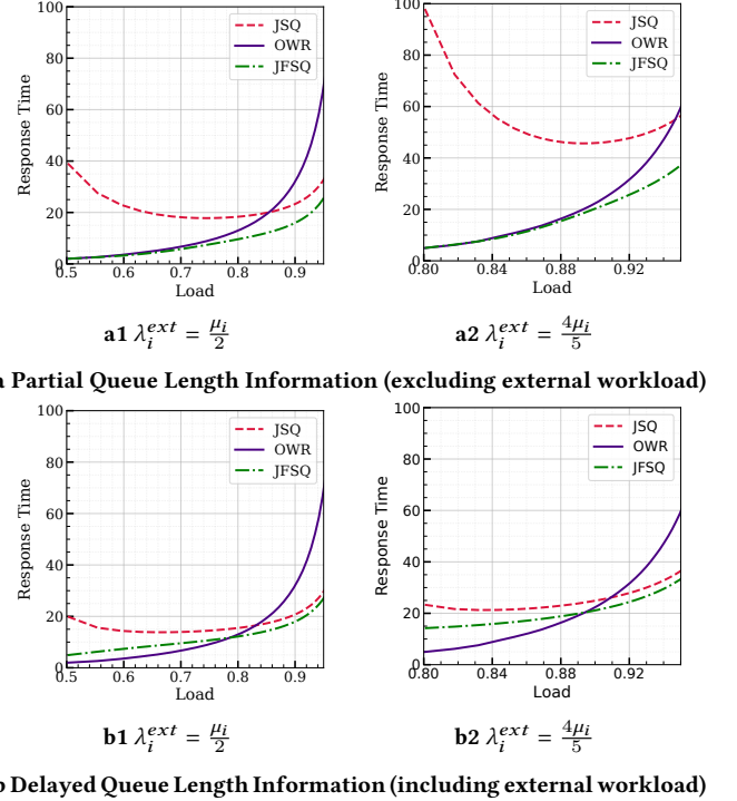
b Delayed Queue Length Information (including external workload)
