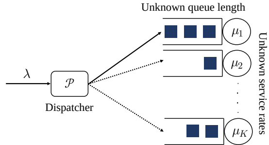
Figure 1: Our system model with job arrival rate \lambda and K servers with service rates \mu_1, \dots, \mu_K respectively. The dispatching policy \mathcal{P} assigns each job to one of K queues. The service rates and queue lengths are unknown to the dispatcher; it only observes the service times of departed jobs.
