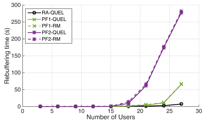
Fig. 10. Re-buffering comparison between RAQUEL and the conventional proportional fairness and rate matching methods for streamloading. The base layer limit is fixed at 50 seconds.
