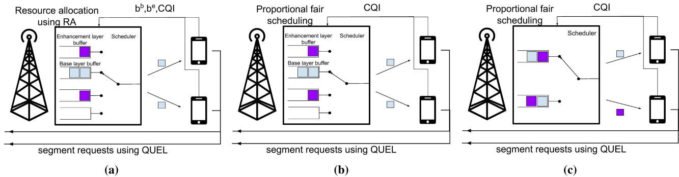
Fig. 4. Three different schemes for scheduling in terms of base station functionality. In all three cases, the quality request procedure is based on QUEL. From (a) to (c) complexity and signaling overhead decrease with the scheme presented in (c) not requiring any packet inspection at the base station. (a) RA-based scheduling with two buffers per user at base station. (b) Proportional fair scheduling with two buffers per user at base station (PF1). (c) Proportional fair scheduling with single buffer per user at base station (PF2).
