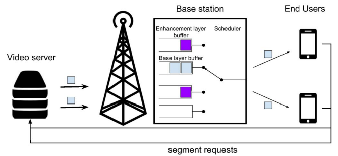
Fig. 3. The delivery procedure for streamloading with RAQUEL for two users. Each user is assigned two buffers at the base station for storing base and enhancement layer segments, respectively. Users request segments which the video server delivers to the base station and the base station schedules the segments for delivery.
