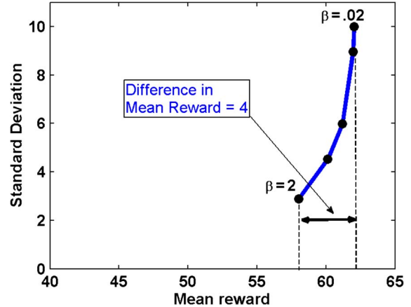
Fig. 1. Homogeneous setting: Mean-variability tradeoffs.
