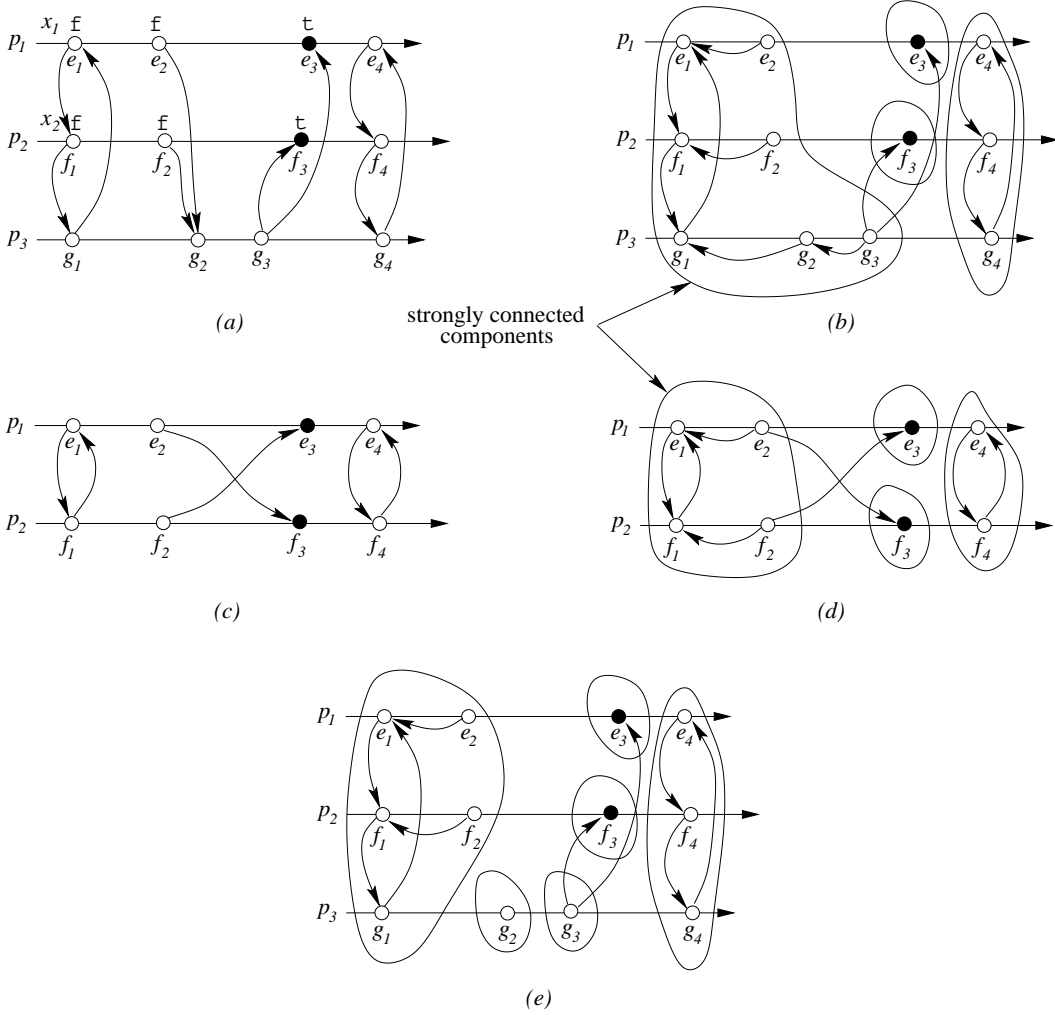
Fig. 8. (a) A computation, (b) its slice with respect to the predicate x_1 \vee x_2 , (c) its projection on processes p_1 and p_2 , (d) the slice of the projected computation with respect to the predicate x_1 \vee x_2 , and (e) the slice computed in (d) mapped to the original set of processes.
