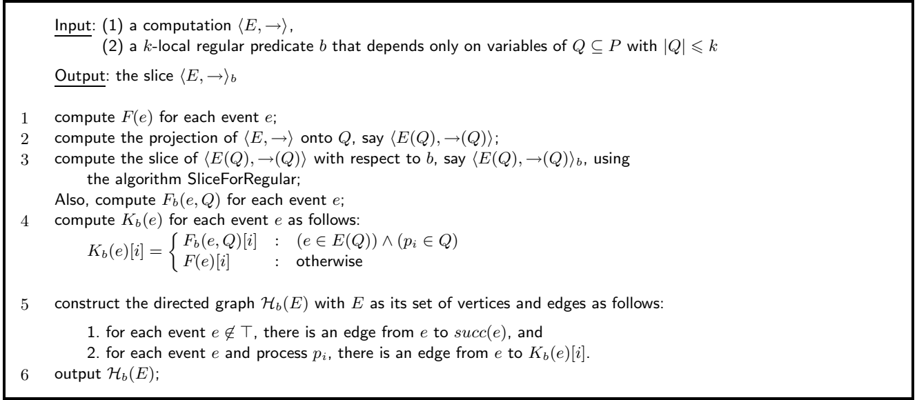
Fig. 7. The algorithm SliceForKLocalRegular to compute the slice for a k -local regular predicate.
