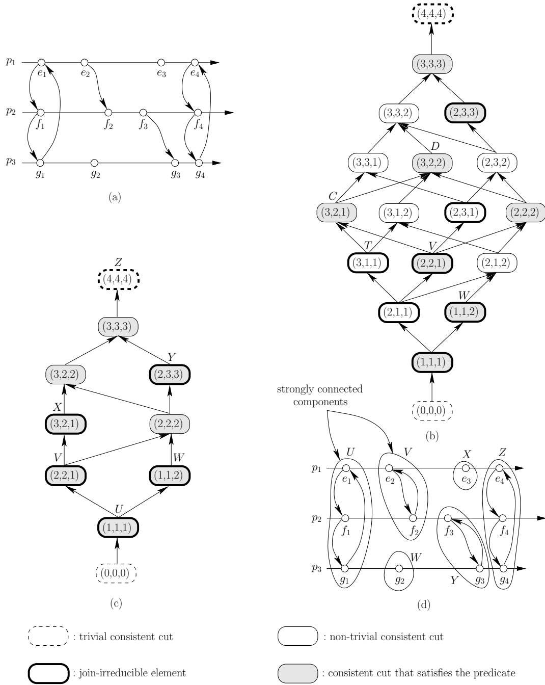
Fig. 2. (a) A computation, (b) the lattice of its consistent cuts, (c) the sublattice of the consistent cuts that satisfy the regular predicate “all channels are empty”, and (d) the poset induced on the set of join-irreducible elements of the sublattice.
