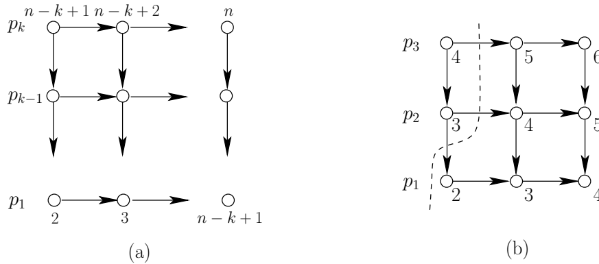
Fig. 13. (a) Computation for subsets of [n] of size k , and (b) example when n = 6 and k = 3 .
