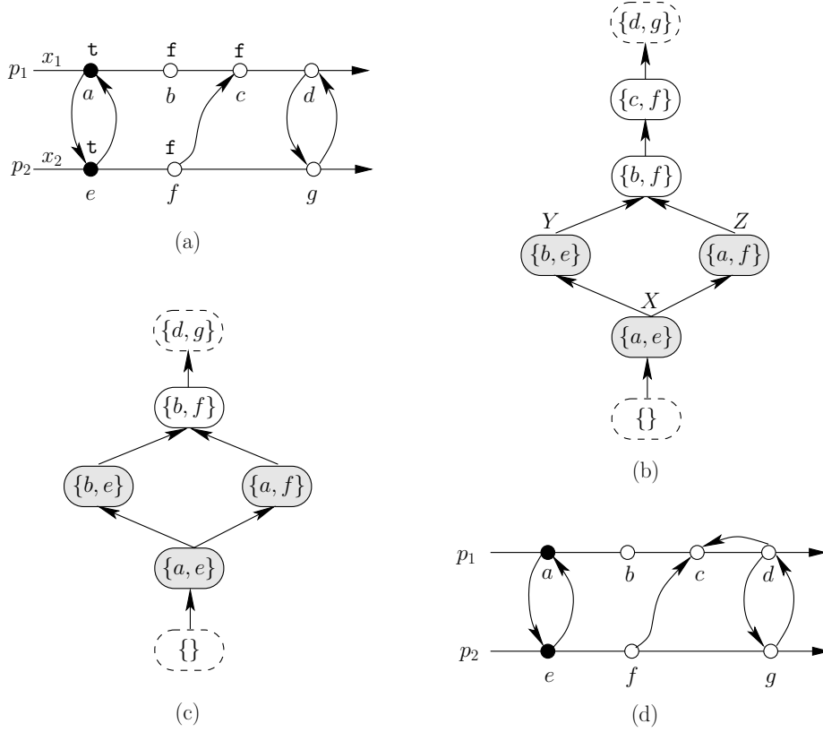
Fig. 3. (a) A computation, (b) the lattice of its consistent cuts, (c) the sublattice of its consistent cuts that satisfy reg(x_1 \vee x_2) , and (d) its slice with respect to reg(x_1 \vee x_2) (and therefore also with respect to x_1 \vee x_2 ).
