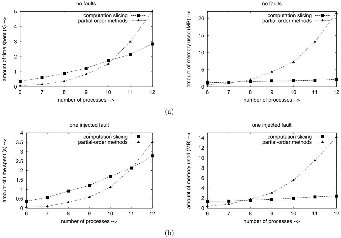
Fig. 11. Primary-Secondary example with the number of events on a process bounded by 90 for (a) no faults and (b) one injected fault.
