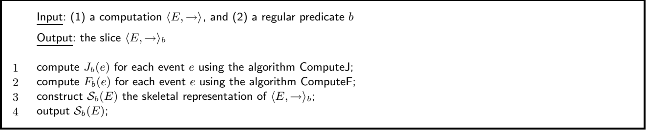
Fig. 6. The algorithm SliceForRegular to compute the slice for a regular predicate.
