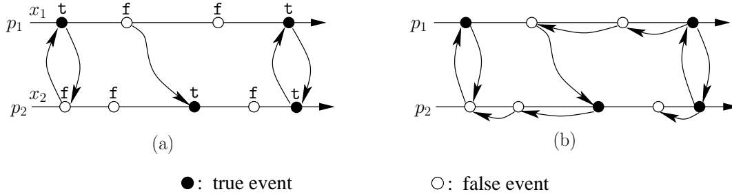
Fig. 10. (a) A computation, and (b) its slice with respect to the conjunctive predicate x_1 \wedge x_2 .
