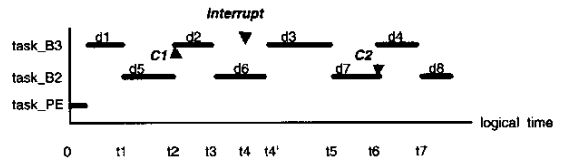
(b) scheduled model
