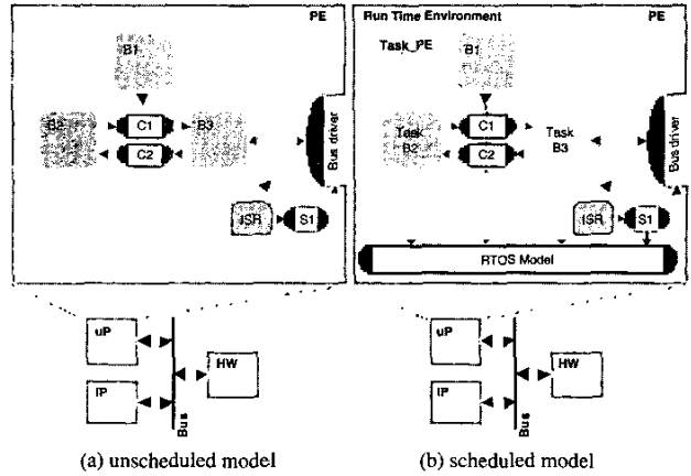
Figure 4: Refinement example
