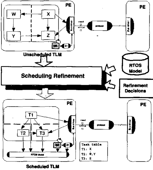
Figure 2: Scheduling refinement tool
