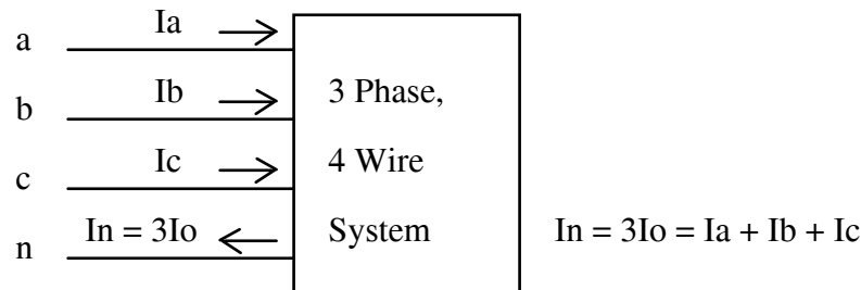
Figure 2.1: Relationship Between Zero Sequence Currents and Neutral Current
