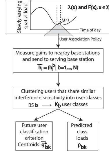
Fig. 2: Traffic abstractions to enable efficient coordination.
