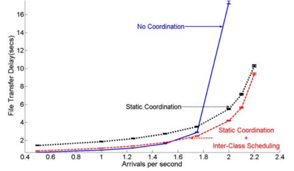
Fig. 9: Delay performance with inter-class scheduling.
