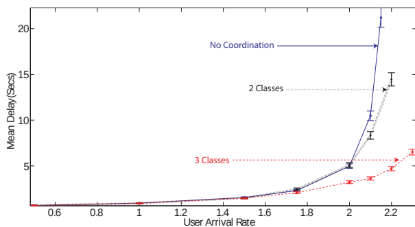
Fig. 17: Uplink delay performance under schedules factoring inter-base station coupling.
