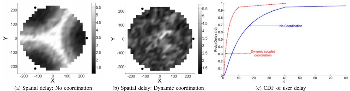
Fig. 13: Distribution of user-perceived delay
