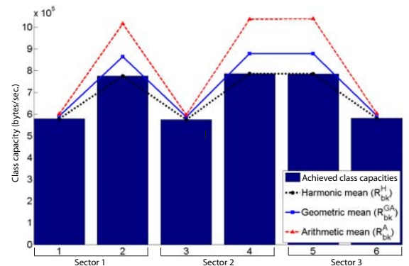
Fig. 6: Comparing the different estimates for class capacity
