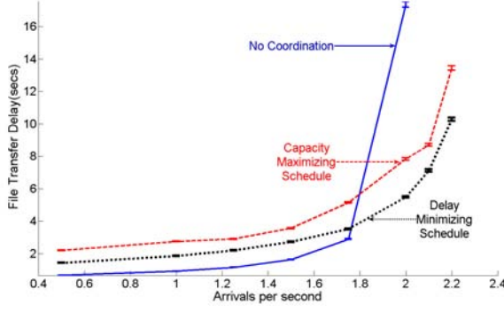
Fig. 8: Performance of capacity maximizing vs. delay optimal static, decoupled schedules with 2 classes per sector.
