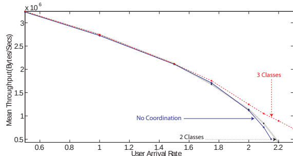
Fig. 18: Average throughput under schedules factoring inter-base station coupling.
