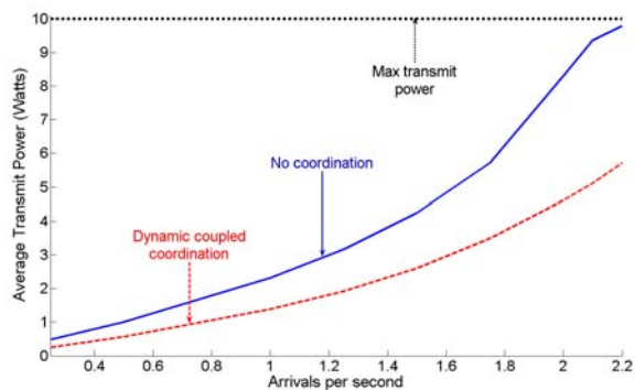
Fig. 14: Average power consumed at the base stations.
