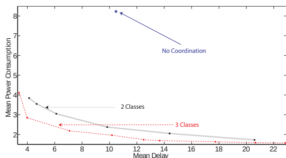
Fig. 19: Power-Delay tradeoffs on the uplink.
