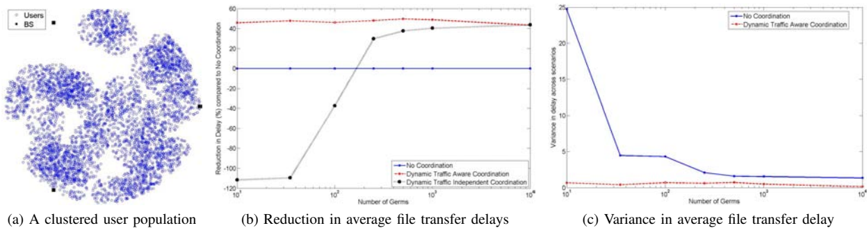
Fig. 15: A scenario with non-homogeneous spatial load
