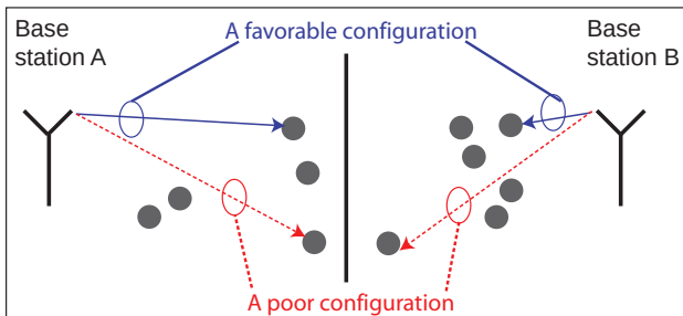
Fig. 1: Traffic abstractions to enable efficient coordination.
