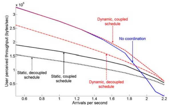
Fig. 12: Average user throughput under schedules factoring inter-base station coupling, with 2 classes per sector.
