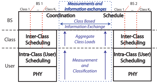
(a) System architecture for coordination.
