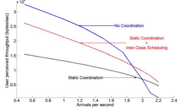
Fig. 10: User throughput with inter-class scheduling.
