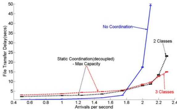
Fig. 7: Average file transfer delays under capacity maximizing static schedules.
