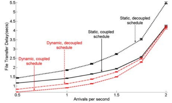
Fig. 11: Average file transfer delays under schedules factoring inter-base station coupling, with 2 classes per sector.
