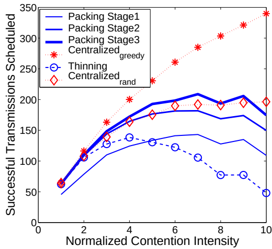
Figure 8: Performance of Packing is robust when contention intensity at each stage is not optimally chosen.
