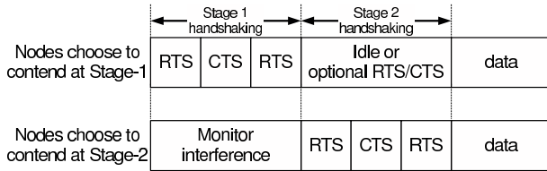
Figure 4: Timing diagrams of a two-stage contention MAC with the top for Stage 1 transmitter/receiver and the bottom for Stage 2 transmitter/receiver.
