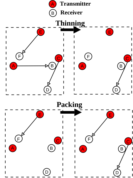
Figure 2: On the top, an example of thinning contenders with only one surviving transmission. On the bottom, an example of a packing of contenders with two surviving transmissions.
