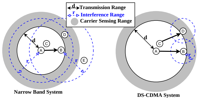
Figure 1: The transmission range, interference range and carrier sensing ranges for an idealized narrow-band and spread spectrum system. Since A \rightarrow B requires no concurrent transmission in the critical interference range r around a B , C \rightarrow D is not allowed in a narrow-band system, but may be allowed in a CDMA system.
