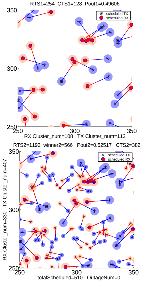
Figure 6: On the top, the resulting transmitter-receiver pairs of a multistage multi-class contention protocol's Stage 1 contention among nodes using longer relay distances and high transmission powers. At the bottom, the resulting transmitter-receiver pairs for Stage 1 and 2 for a multi-class multistage contention protocol.
