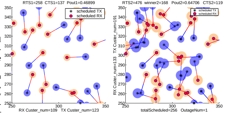
Figure 5: On the left, contention result of successful transmitter-receiver pairs of Stage 1. On the right the contention result after Stage 2.
