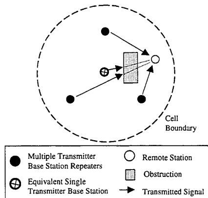
Figure 4. Reduced shadowing with a multiple transmitter cell
