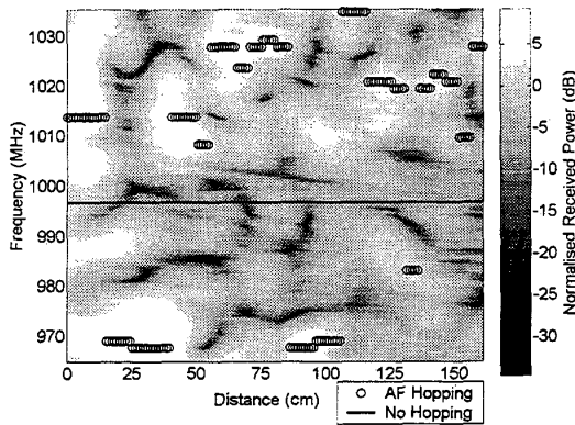
Figure 1. Single user Adaptive Frequency Hopping
