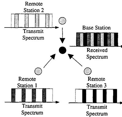
Figure 3. Reverse link of a multiuser OFDM system
