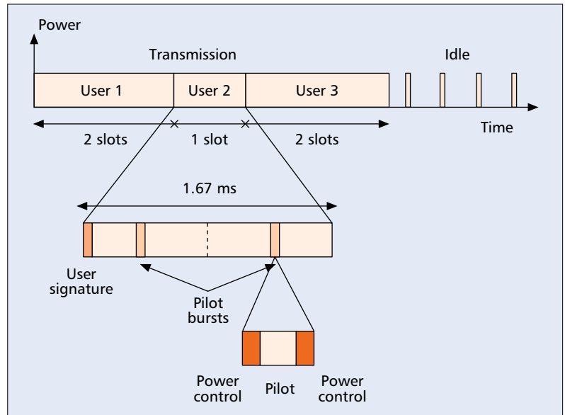
■ Figure 1. An access point transmission diagram.
