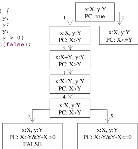
Figure 3. Code that swaps two integers and the corresponding symbolic execution tree
