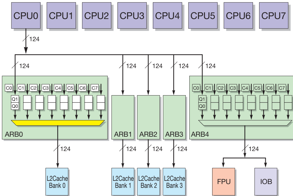
FIGURE 3-9 Data Flow in PCX Arbiter
