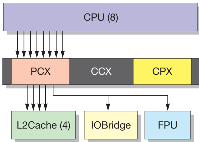
FIGURE 3-2 Processor Cache-Crossbar (PCX) Interface
