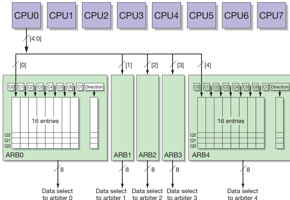
FIGURE 3-10 Control Flow in PCX Arbiter
