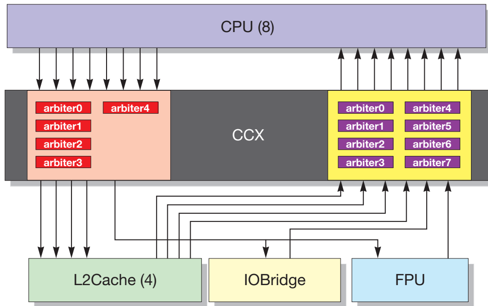
FIGURE 3-8 PCX and CPX Internal Blocks
