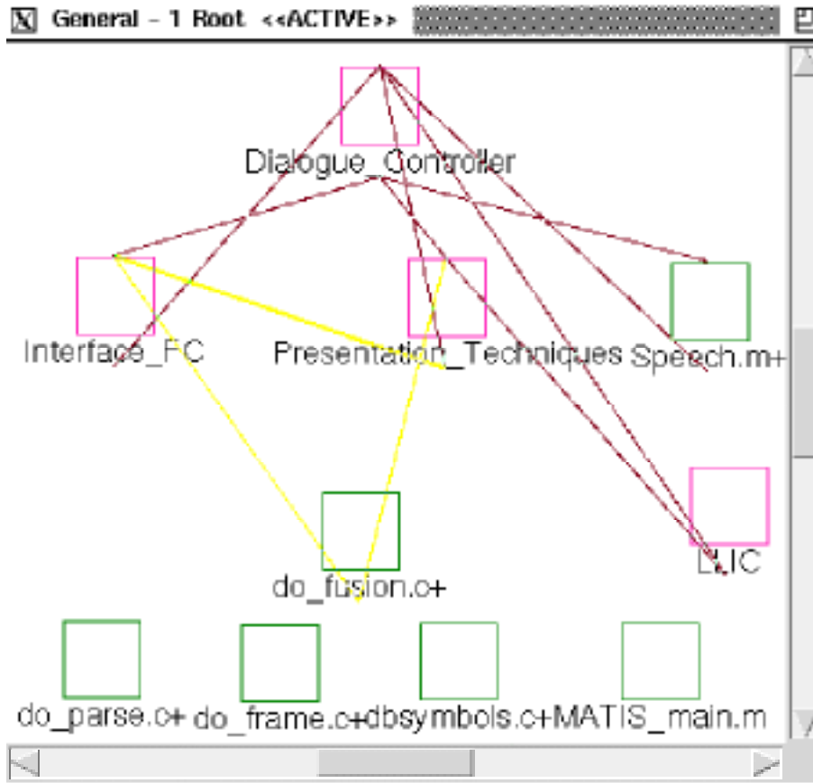
Figure 7: Recognized PAC-Amodeus Pattern in MATIS. Solid lines represent calls relations and shaded lines represent variable access relations
