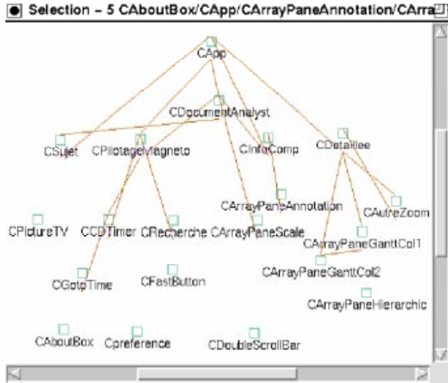
Figure 5: As-implemented Architecture of SupraAnalyse Using PAC Patterns
