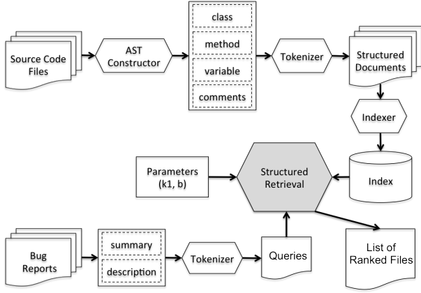
Fig. 2. BLUiR Architecture
