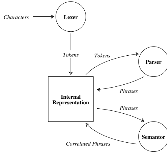
Figure 4: Partial Functional View of Parallel Process, Shared Data Structure Compiler Architecture.
