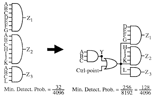
Figure 5. Example of Cube Extraction with Control Point (same form applies if Y is a kernel)
