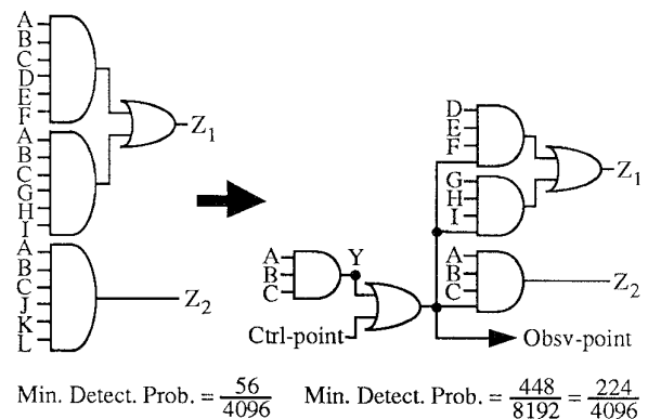
Figure 6. Example of Cube Extraction with Control and Observation Point (same form applies if Y is a kernel)
