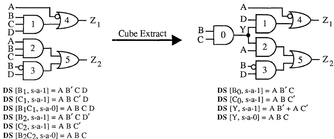
Figure 2. Example of Effect of Extracting a Common Cube on Detecting Sets
