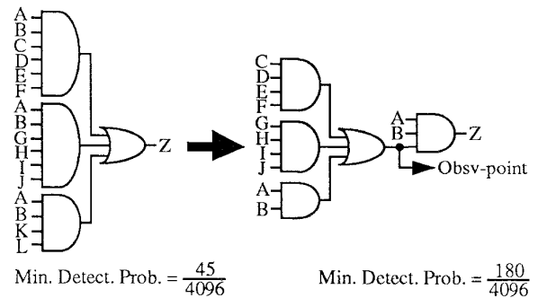
Figure 4. Example of Kernel Extraction with Observation Point
