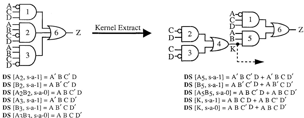
Figure 3. Example of Effect of Extracting a Kernel on Detecting Sets
