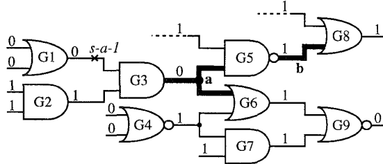
Figure 4. Example: Observation Point at Node a or b is a Solution
