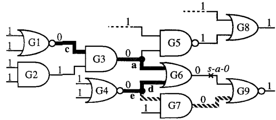
Figure 5. Example: Control-1 Point at Node a , c , or d is a Solution, but Node e is Not a Solution Because It Blocks Propagation to a Primary Output
