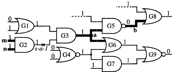
Figure 7. Example: A Control-0 Point at Node m or n Provokes the Fault, and an Observation Point at Node a or b Propagates the Fault to a Primary Output.
