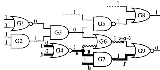
Figure 6. Example: Control-0 Point at Node f , g , or h are Solutions, but Nodes e , i , and j are Not Solutions Because They Don't Provoke the Fault
