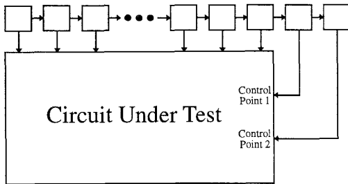
Figure 9 . Control Points Driven by Extra Scan Elements
