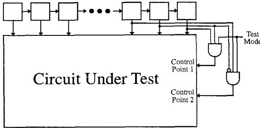
Figure 10 . Control Points Driven by Pattern Decoding Logic
