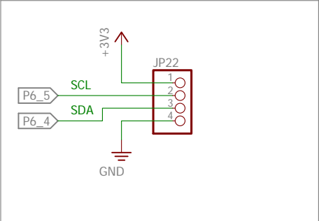
Optional I2C Sensor Interface
