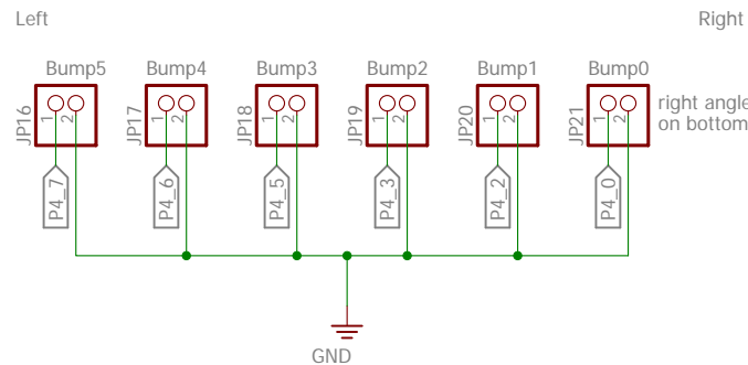
Ground for Bump Switches
