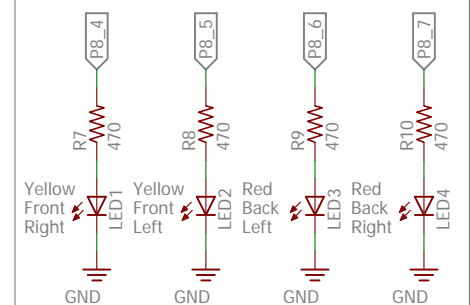
Optional LED Lights
