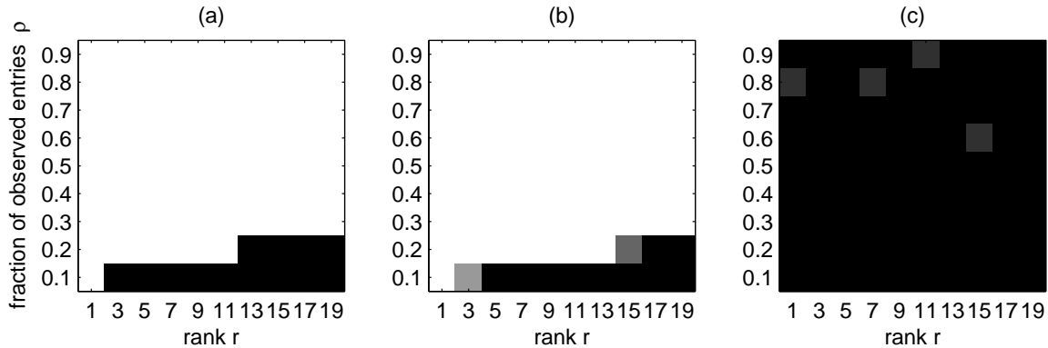
Fig. 1. Experiment results for 400 \times 400 matrix with one corrupted column. We plot the probability of successful recovery of the low rank matrix. Panes (a) and (b) show the results of our approach with and without the corrupted column, respectively. Pane (c) shows the essentially complete failure of standard matrix completion, due to the corrupted column.
