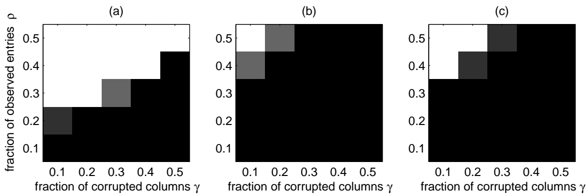
Fig. 2. Experiment results for 400 \times 400 rank-10 matrix with different fraction of observed entries \rho and fraction of corrupted columns \gamma . Corrupted columns are generated neutrally random. Panes (a) and (c) show the results of our approach and standard matrix completion, respectively. Pane (b) shows the results of minimizing a convex combination of the nuclear norm and the matrix \ell_1 norm.
