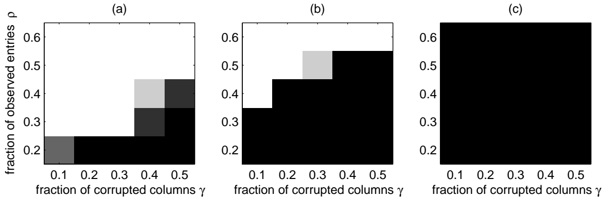
Fig. 3. Experiment results for adversarial corruptions. Other settings are the same as in Fig. 2.
