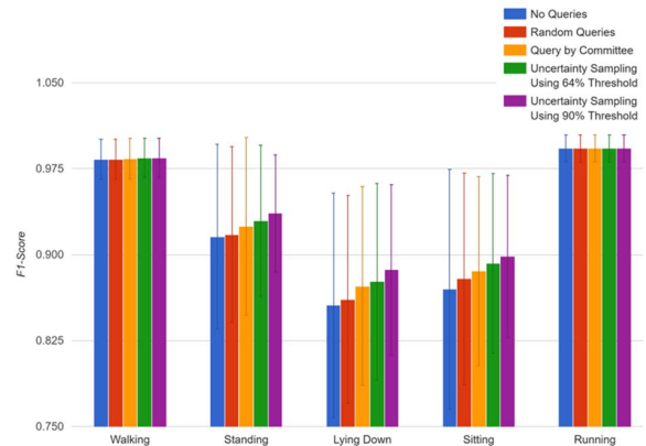
Fig. 8. Model certainty based on the number of visited samples for the different activities.
