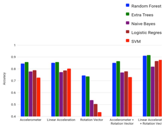
Fig. 4. Accuracy of the classifier tested for each sensor combination.
