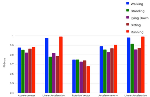
Fig. 5. F1 score of activities obtained by the Extra Trees classifier for each sensor combination.
