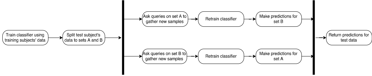
Fig. 3. Workflow of the active learning model evaluation.
