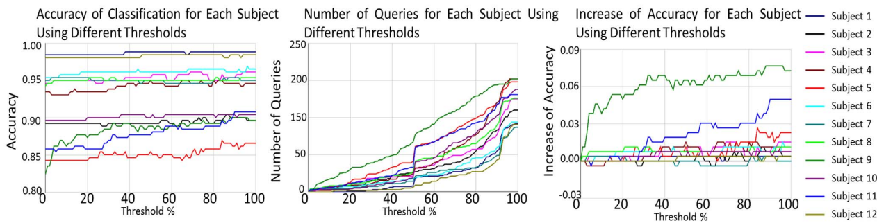
Fig. 7. Simulation results after performing Uncertainty Sampling. Accuracy, number of queries, and increase in accuracy for each subject is shown based on the uncertainty threshold.
