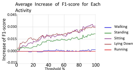
Fig. 9. Average increase of F1-score for each activity using the active learning model.
