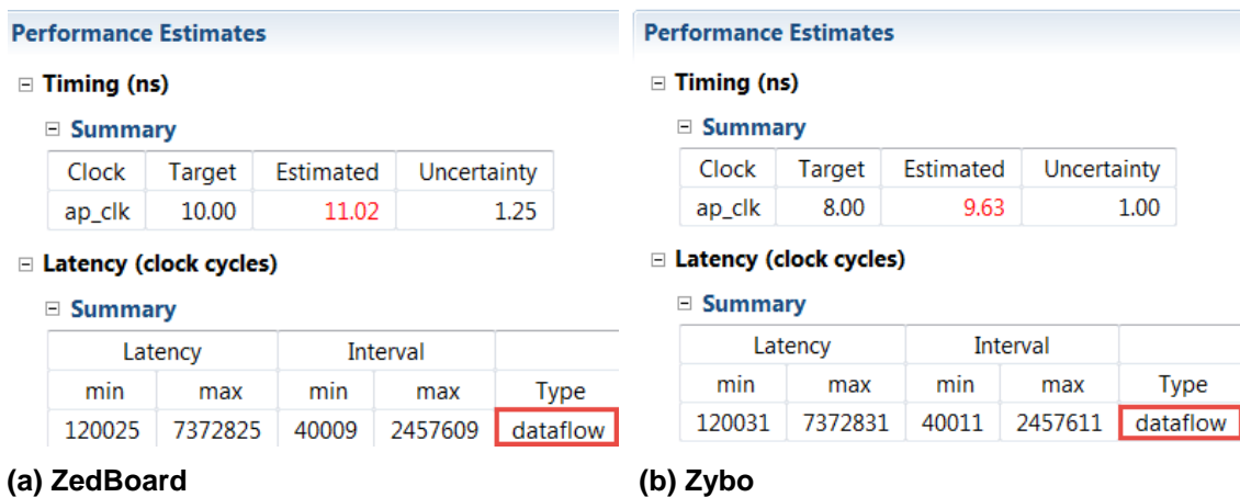
Figure 15. Performance estimate after DATAFLOW directive applied
