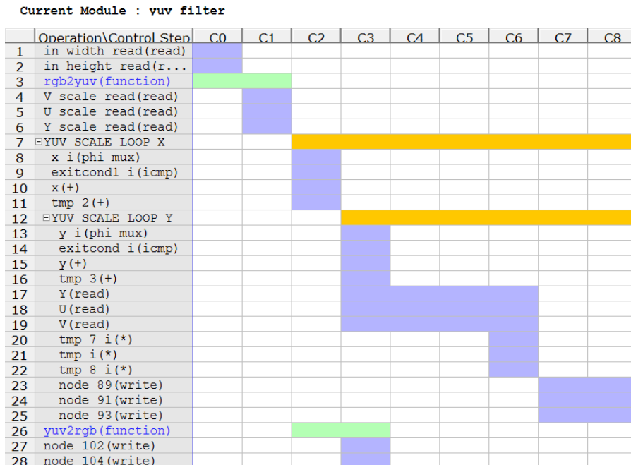
Figure 9. Design analysis view of the YUV_SCALE_LOOP_Y loop
