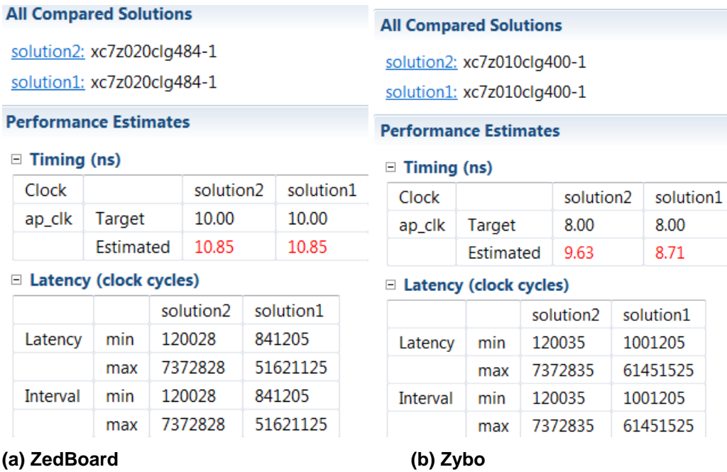
Figure 13. Performance comparison after pipelining
