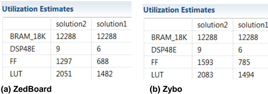
Figure 14. Resources utilization after pipelining
