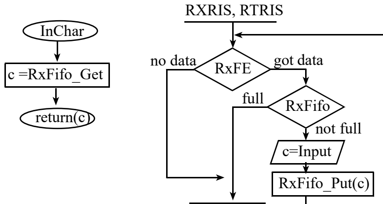
Figure 2.8. One possible interrupt synchronization for the serial input.
