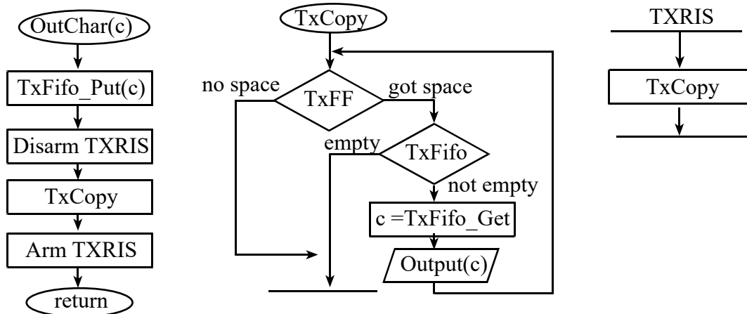
Figure 2.9. One possible interrupt synchronization for the serial output.
