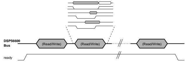
Figure 14: Application layer synchronization protocol.
