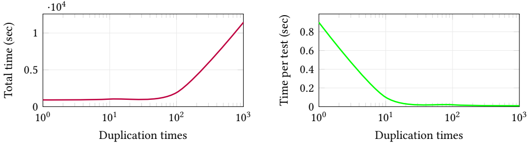
Fig. 14. Duplication times vs. total time (left) and average time (right).
