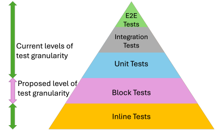
Fig. 2. Testing pyramid.
