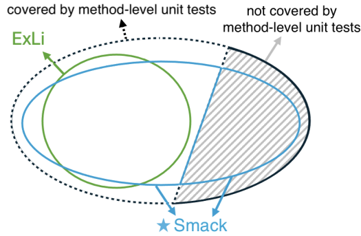
■ Figure 3 The gap in inline-test generation that SMACK fills (not drawn to scale).
