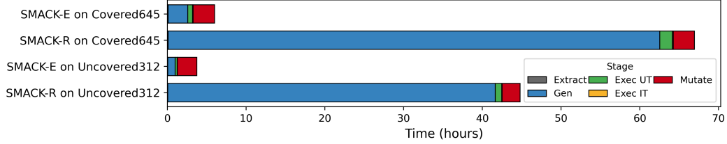
■ Figure 20 Time breakdown of SMACK on UNCOVERED312 and COVERED645.
