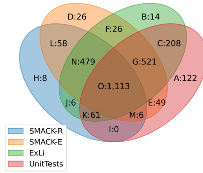
■ Figure 14 Mutants killed by SMACK (using Randoop and EvoSuite) and ExLi on COVERED645.
