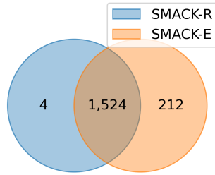
■ Figure 13 Mutants killed by SMACK-generated inline tests using Randoop (SMACK-R) or EvoSuite (SMACK-E).
