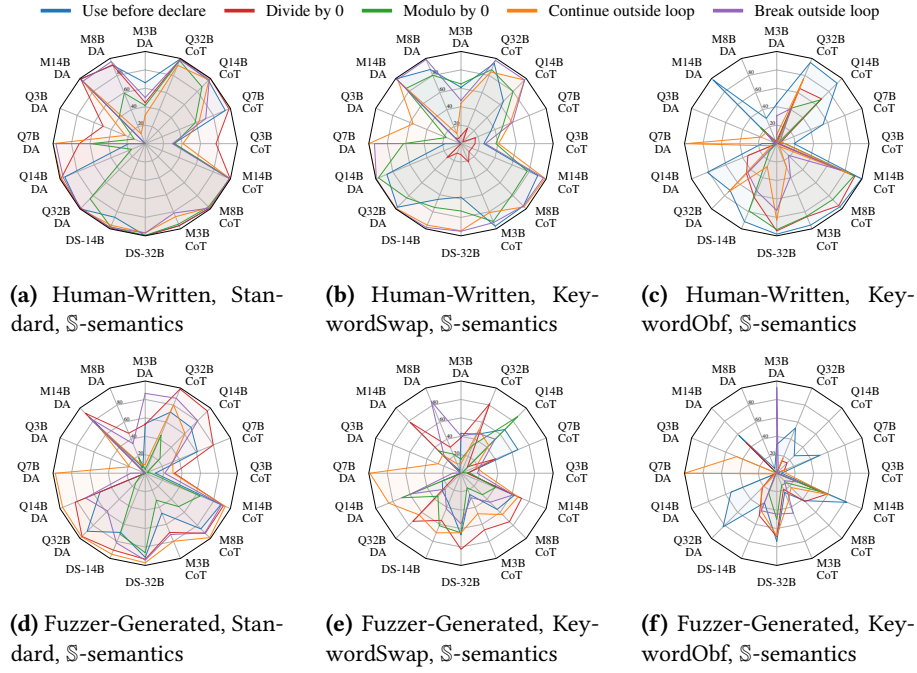
Figure 5. Per-error-type accuracy on invalid C* programs across all evaluated models under §-semantics. The top row shows Human-Written programs and the bottom row shows Fuzzer-Generated programs (Standard, KeywordSwap, and KeywordObf configurations). Radar axes are models and each colored polygon is a semantic error type. Radial grid lines mark accuracy percentages, using the same rule-level criterion as Tables 6 and 8.
