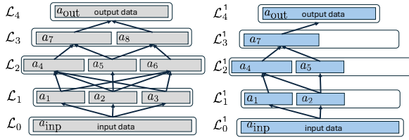
Fig. 1. Left: an example of parent DNN architecture highlighting the input data atom, the computational atoms (including the output data atom), the layers they belong to, and their connectivity. Right: an example of a task-specific DNN architecture derived for a given task.
