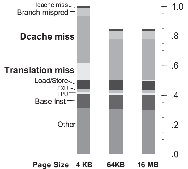
Figure 1. 471.omnetpp Normalized CPI
