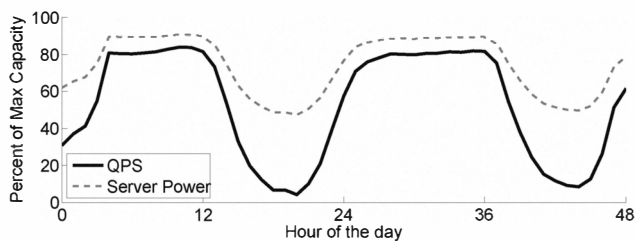
Figure 1: Example diurnal pattern in queries per second (QPS) for a Web Search cluster: Non-peak periods provide significant opportunity for energy-proportional servers. For a perfectly energy proportional server, the percentage of peak power consumed and peak QPS would be the same. Server power is estimated for systems with 45% idle power.
