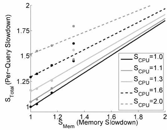
(b) Average query slowdown as a function of memory slowdown (holding CPU slowdown constant). Data points at S_{mem} = 1.3 exhibit test-harness-specific memory bandwidth effects and are excluded from the regression.
