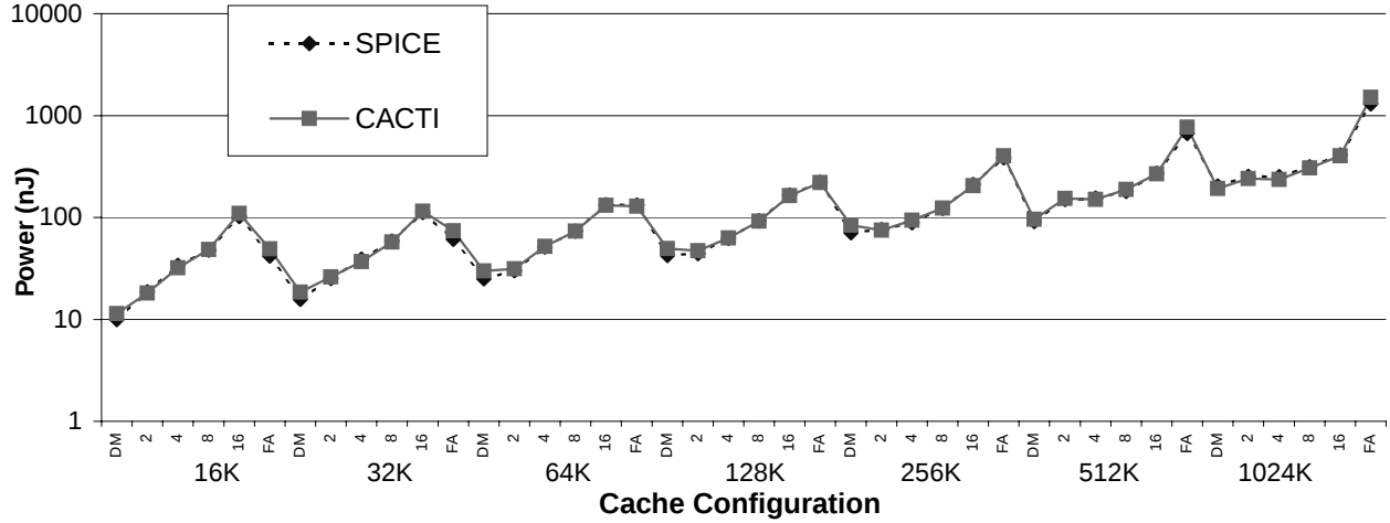
Figure 8: Comparison of power consumption for a variety of cache configurations in both CACTI and SPICE. The y-axis is on a logarithmic scale, and shows the cache power consumption in nanojoules. The x-axis ranges over a variety of cache configurations - all with 32 byte block sizes. Caches sizes of 16K, 32K, 64K, 128K, 256K, 512K, and 1024K are all shown, each broken down into six associativity configurations (direct mapped, 2-way, 4-way, 8-way, 16-way, and fully associative).
