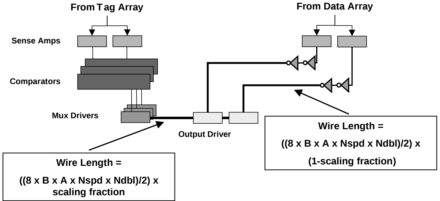
Figure 2: Balancing the tag and data paths. CACTI will determine the scaling factor for the wire length between the mux drivers and output drivers that will result in the lowest overall cache delay.
