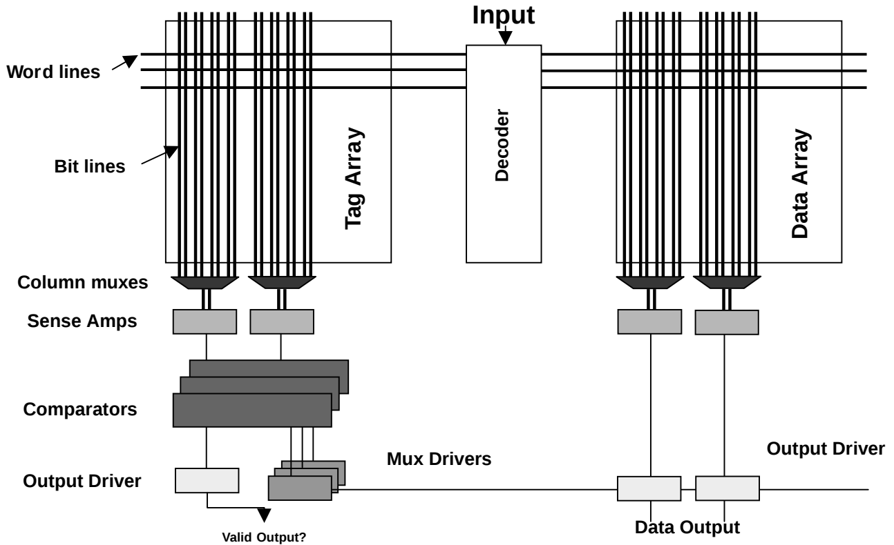
Figure 1: Cache model used in CACTI [6].
