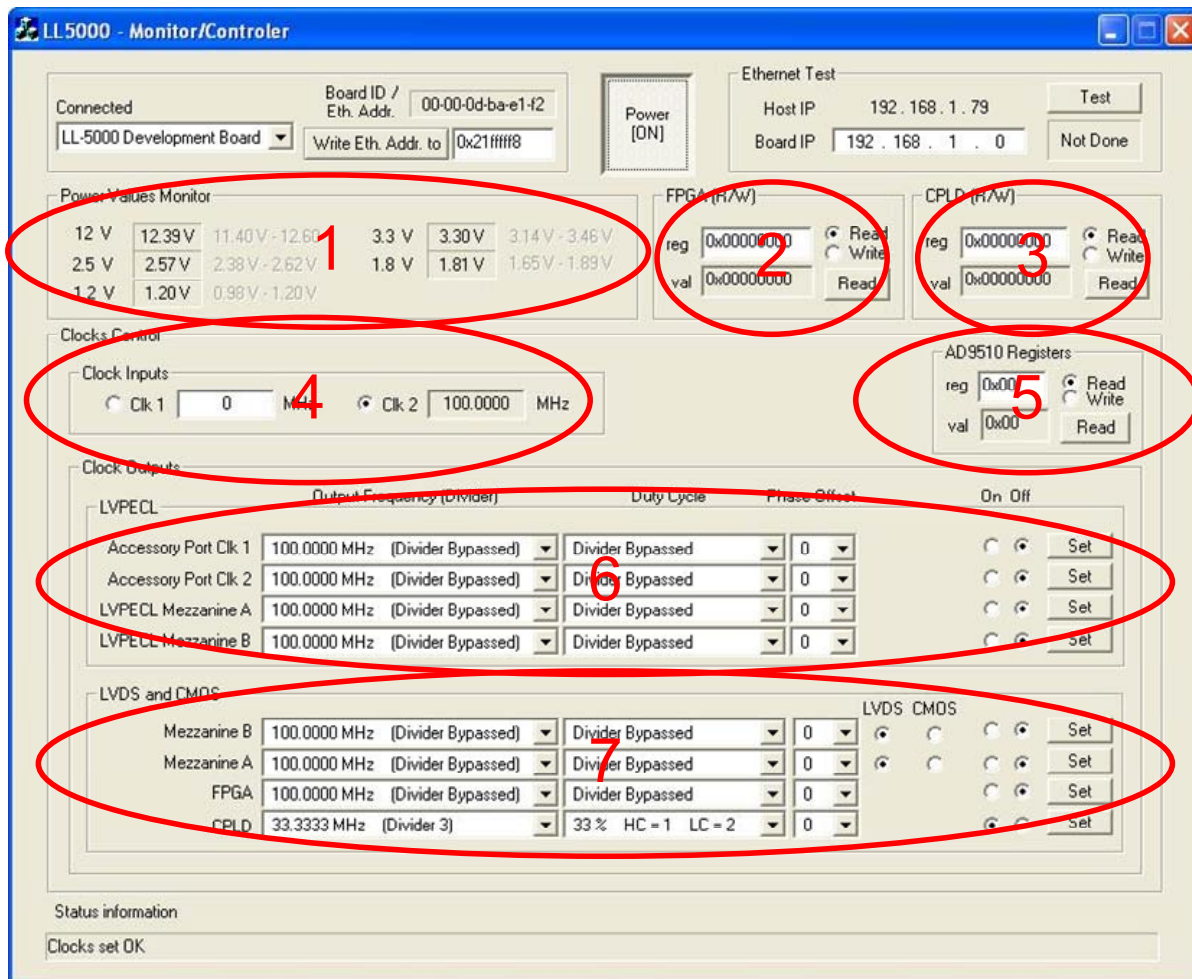
Figure 0.2: TLL5000 Monitor/Controller Power On Screen
