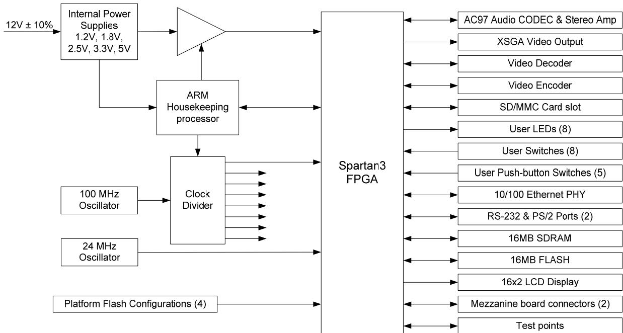
Figure 0.1: TLL5000 Development System Block Diagram
