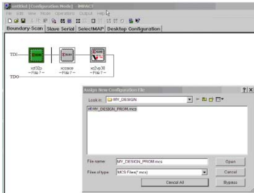
Figure 0.9: Selecting configuration file for XCF32P
