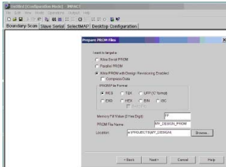
Figure 0.5: Selecting a PROM with Design Revisioning Enabled
