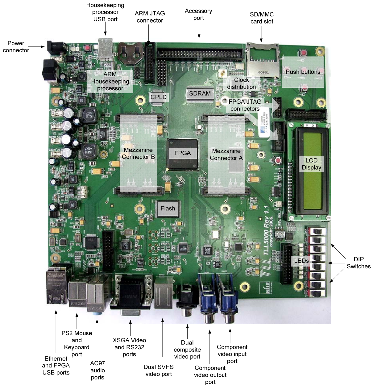
Figure 0.2: TLL5000 Development System Board Photo
