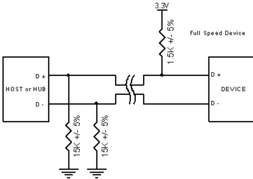
Full Speed Device with pull up resistor connected to D+
