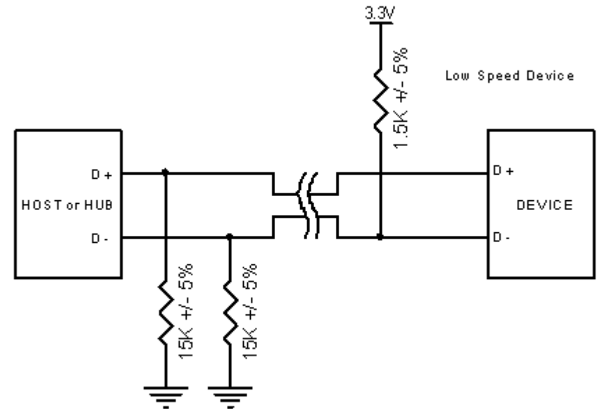
Low Speed Device with pull up resistor connected to D-
