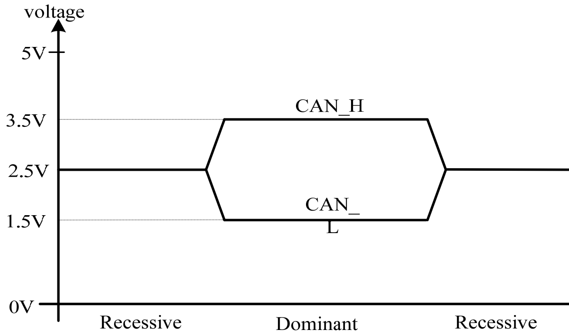
Nominal CAN bus levels
