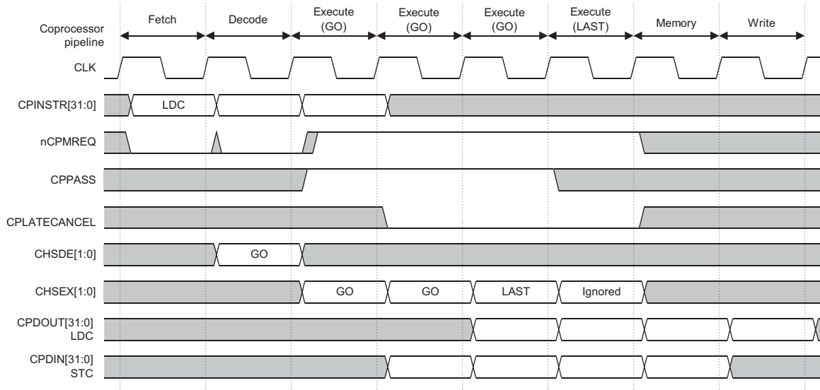
Figure 8-3 LDC/STC cycle timing
