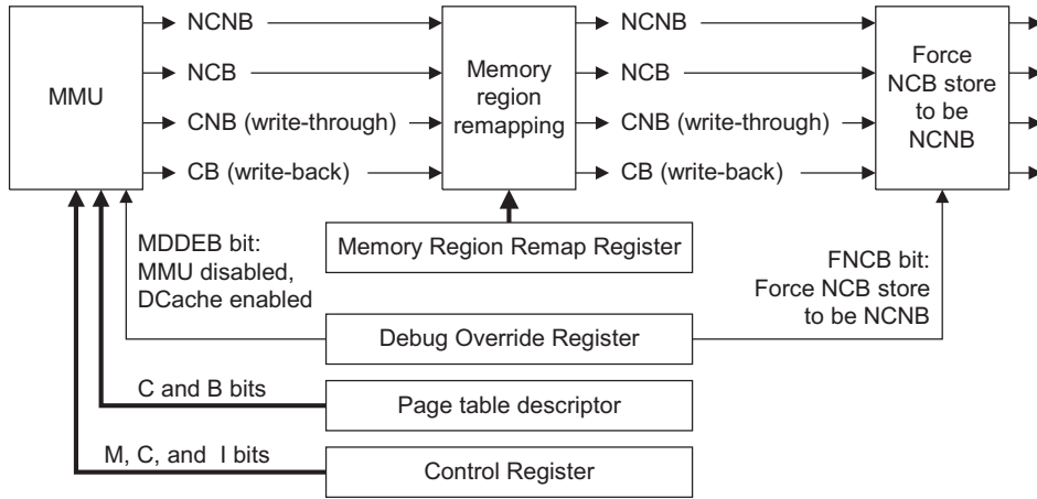
Figure B-10 Memory region attribute resolution
