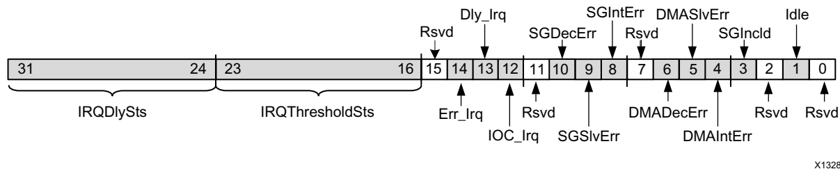
Figure 2-3: CDMASR Register
