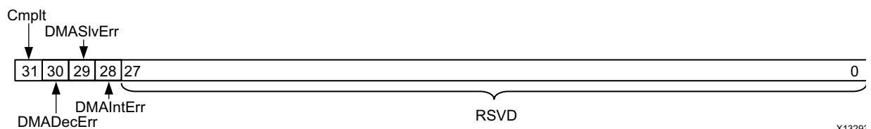
Figure 3-9: Transfer Descriptor Status Word
