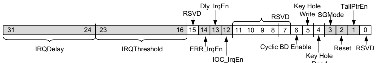
Figure 2-2: CDMACR Register
