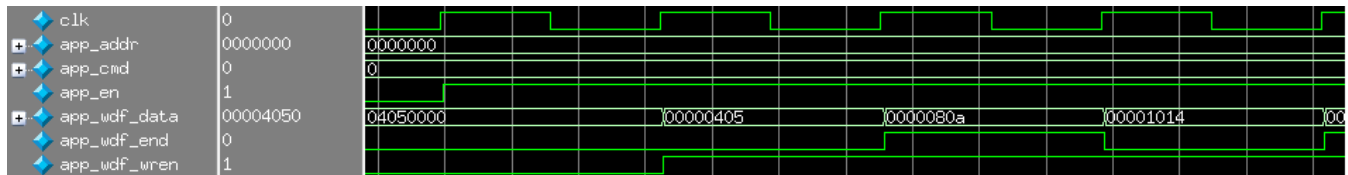
Figure 1-79: Data at the Application Interface for 2:1 Mode
