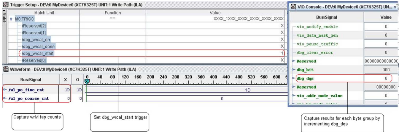
Figure 1-99: Trigger = dbg_wrcal_start
