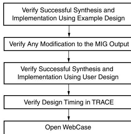
Figure 2-63: Synthesis and Implementation Debug Flowchart
