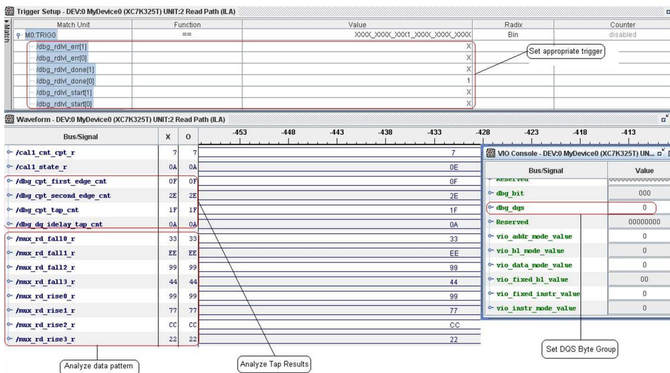
Figure 1-104: Trigger = dbg_rdlvl_done[0]
