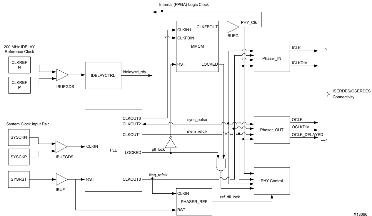
Figure 2-41: Clocking Architecture
