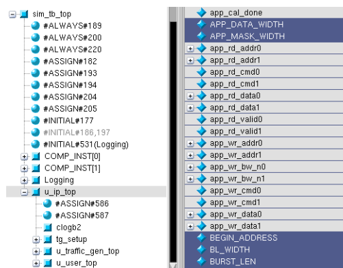
Figure 2-60: QuestaSim Instance Window
