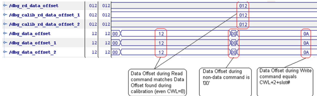
Figure 1-97: Expected Vivado Logic Analyzer Tool Results
