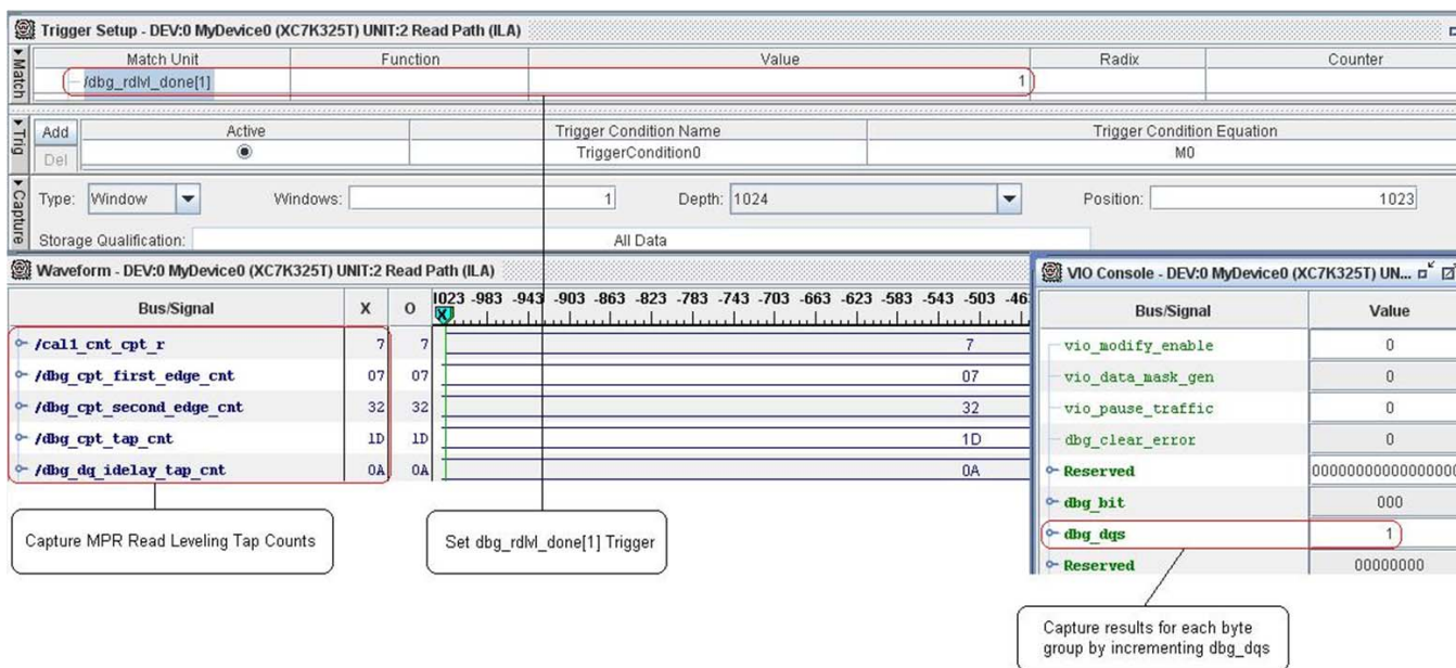
Figure 1-101: Trigger = dbg_rdlvl_done[1]
