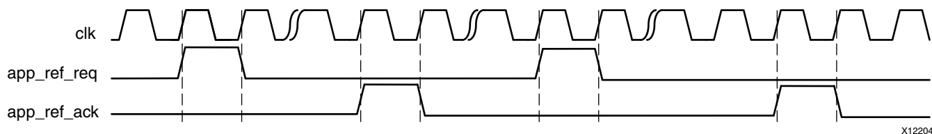
Figure 1-83: User-Refresh Interface
