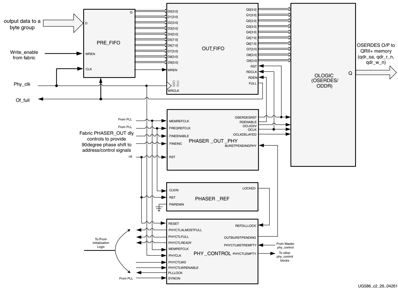
Figure 2-45: Address Path
