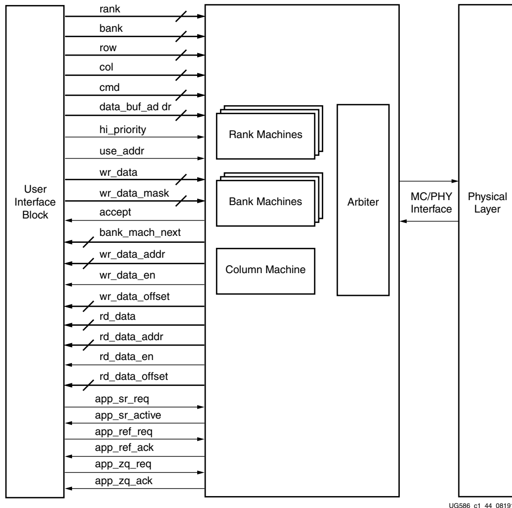
Figure 1-53: Memory Controller
