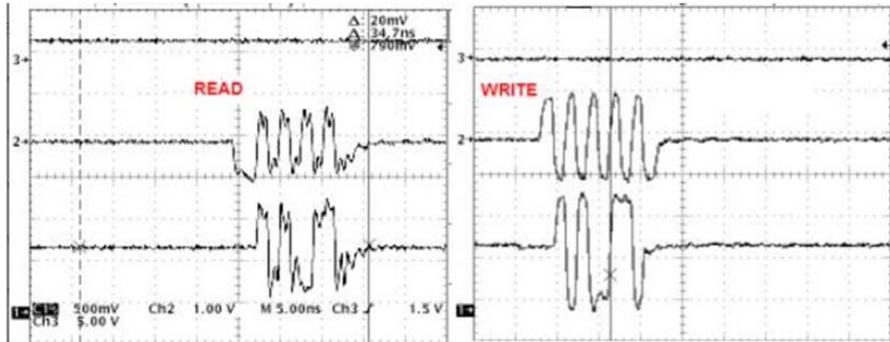
Figure 1-105: Read and Write
