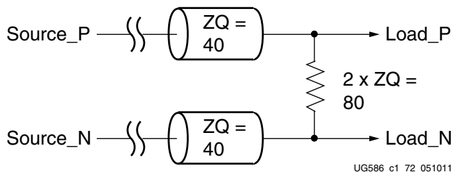
Figure 1-93: 80Ω Differential Termination
