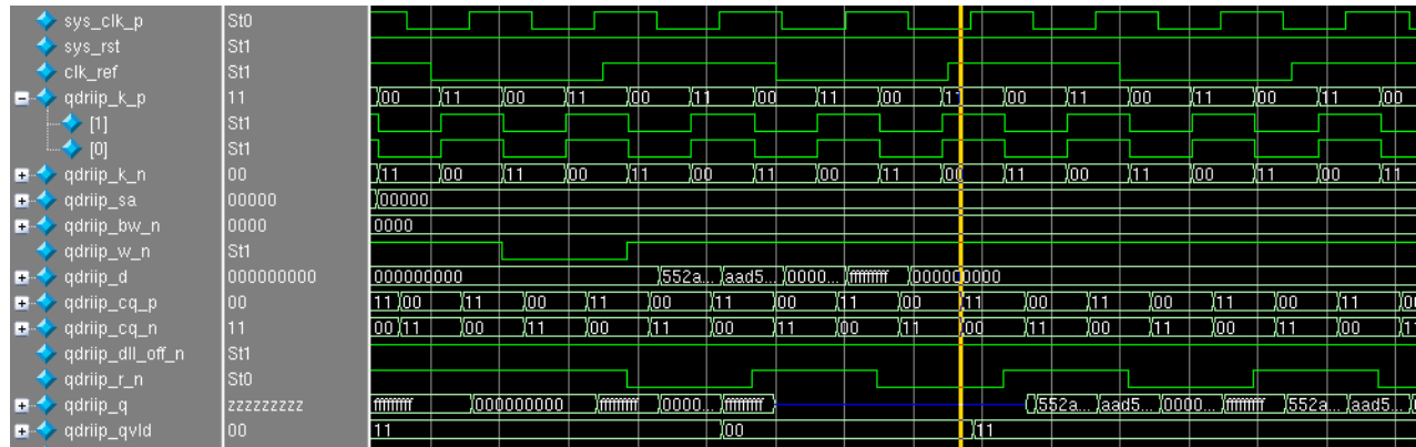
Figure 2-58: Write and Read for Second Stage Read Calibration
