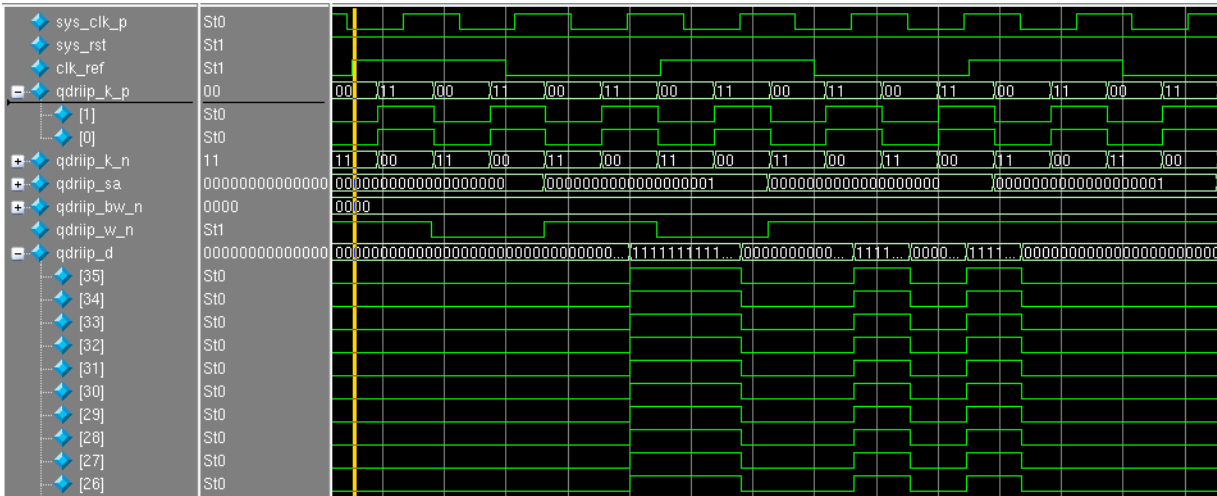
Figure 2-56: Writes for First Stage Read Calibration
