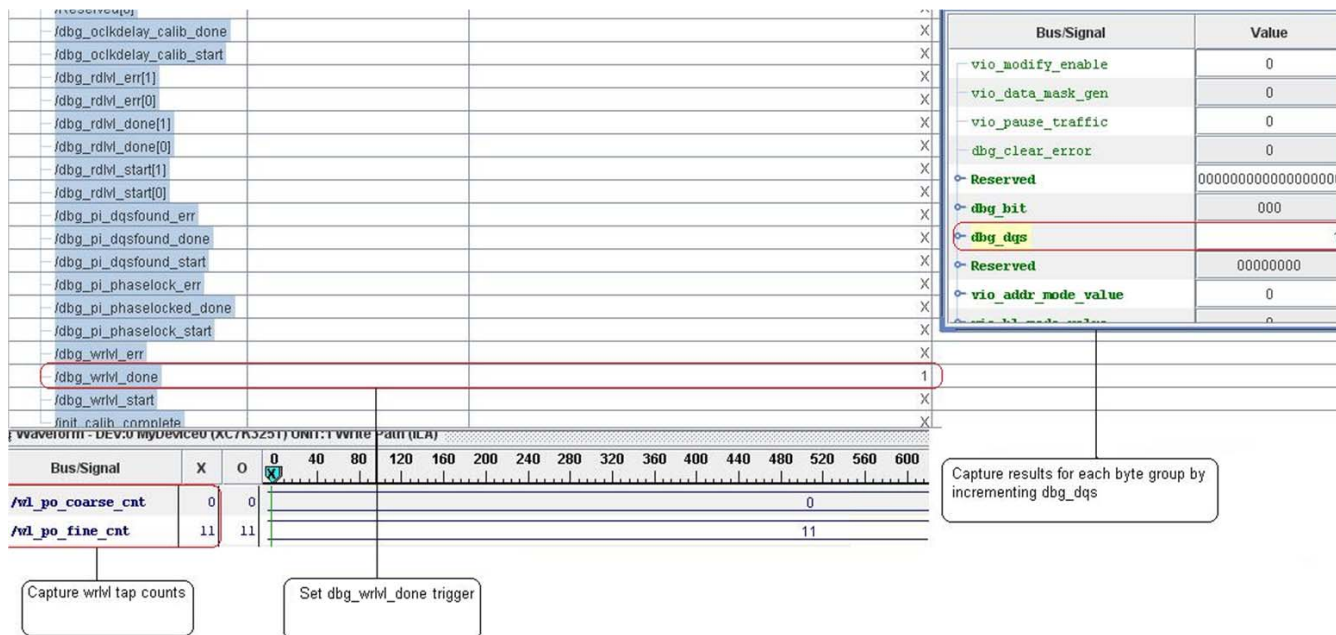
Figure 1-98: Trigger = dbg_wrlvl_done
