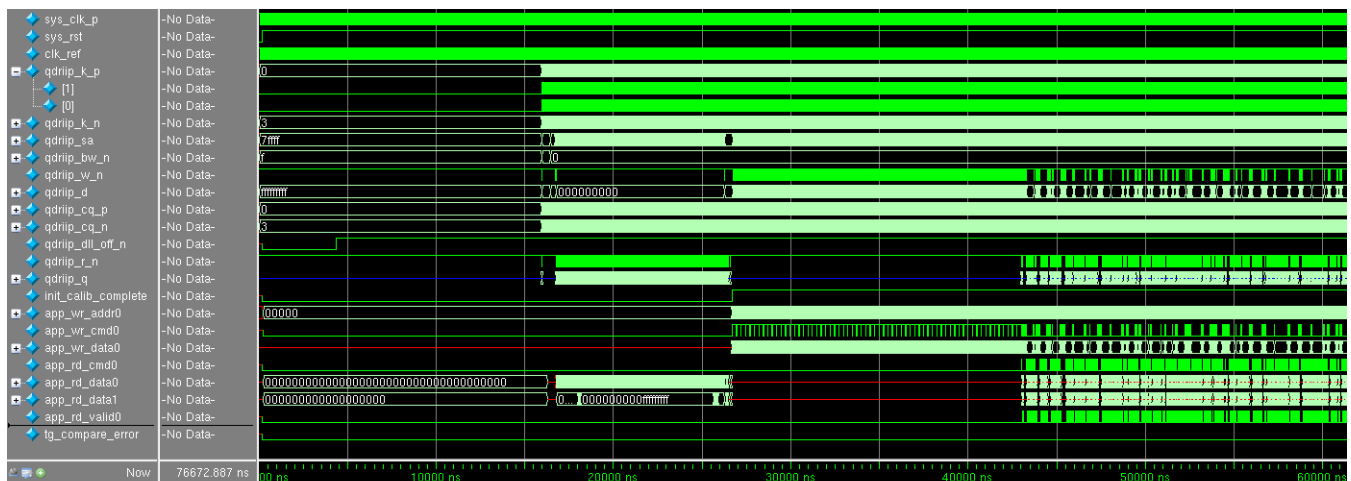
Figure 2-59: Test Bench Operation After Completion of Calibration
