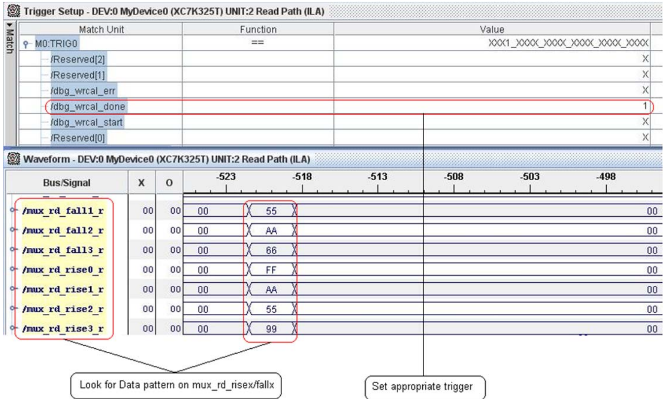
Figure 1-102: Trigger = dbg_wrcal_done
