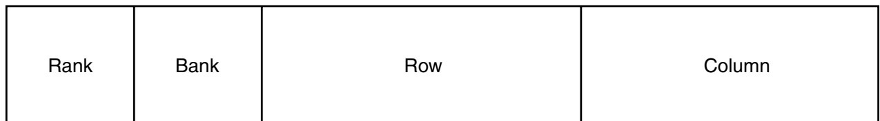
Figure 1-72: Memory Address Mapping for Bank-Row-Column Mode in UI Module
