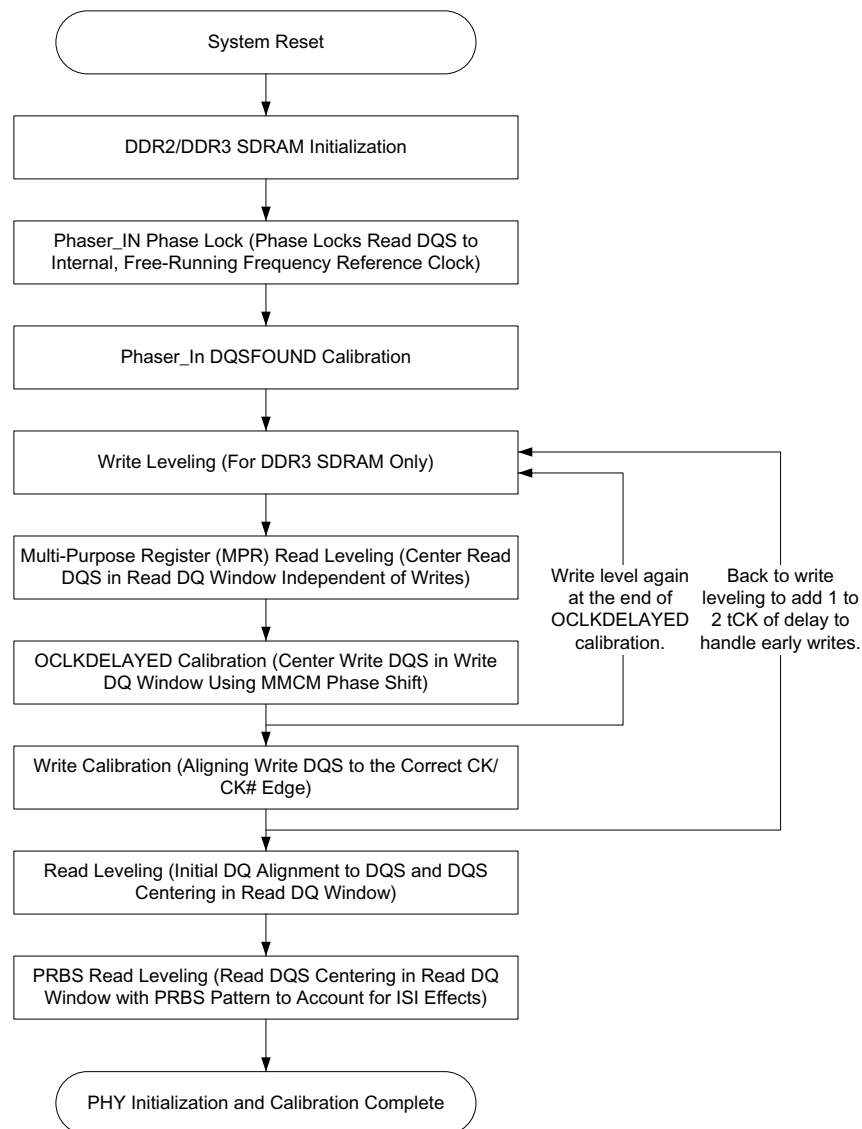
Figure 1-96: Calibration Stages
