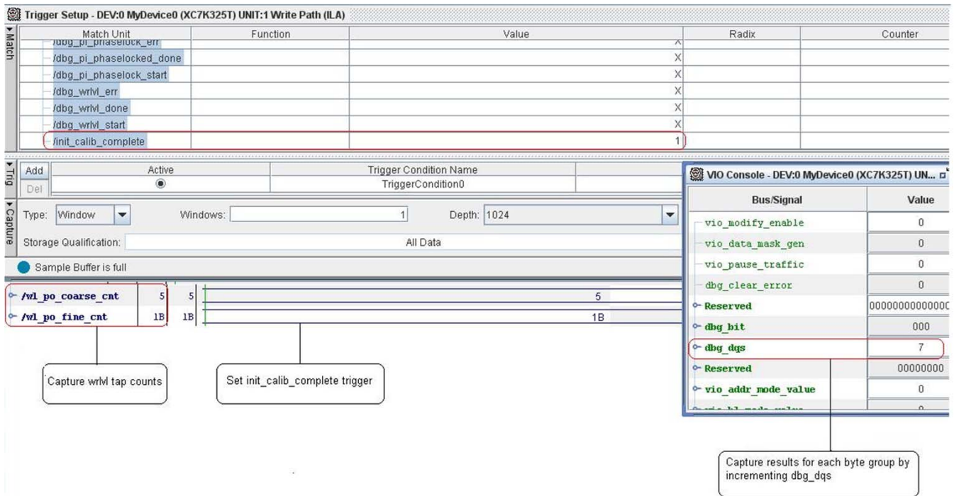
Figure 1-100: Trigger = init_calib_complete
