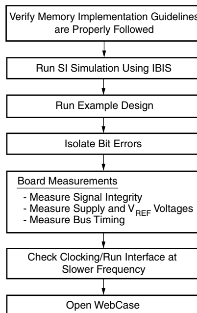
Figure 2-64: Hardware Debug Flowchart
