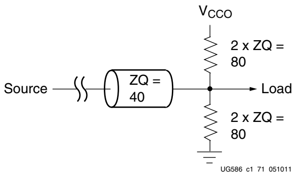
Figure 1-92: 80Ω Split Termination to V CCO and GND
