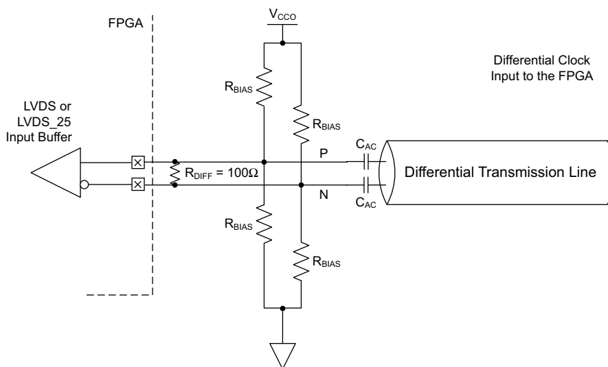
Figure 2-48: Example Circuit for AC-Coupled and DC-Biased Differential Clock Input
