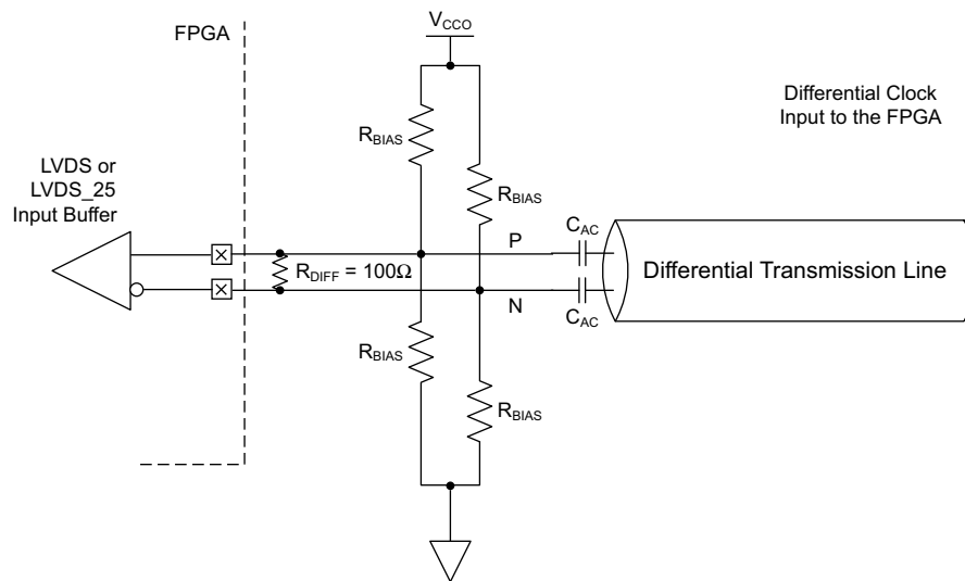
Figure 1-94: Example Circuit for AC-Coupled and DC-Biased Differential Clock Input
