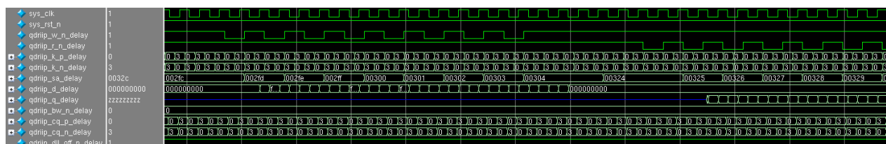
Figure 2-62: QDR II+ Interface Write and Read
