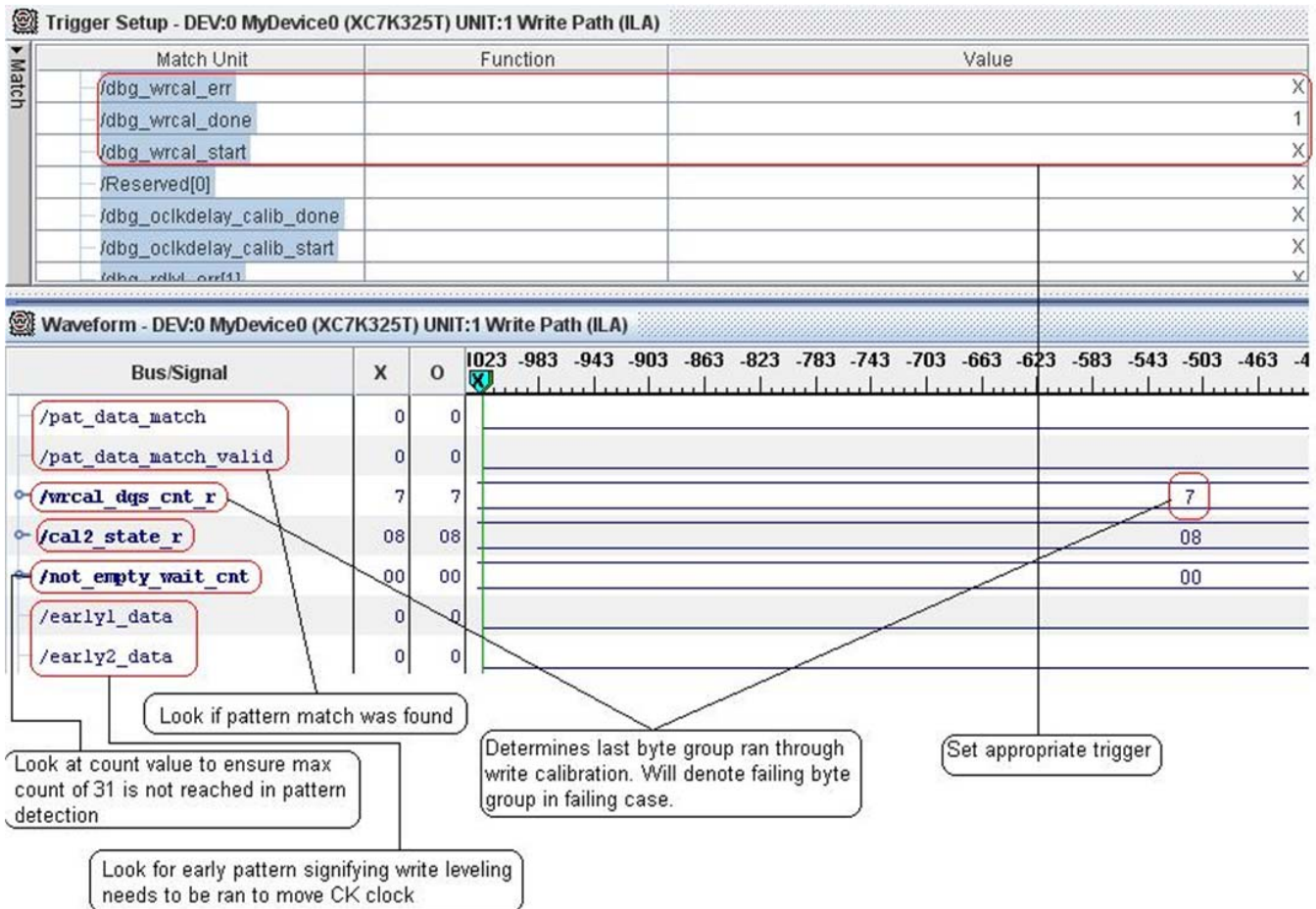
Figure 1-103: Trigger = dbg_wrcal_done
