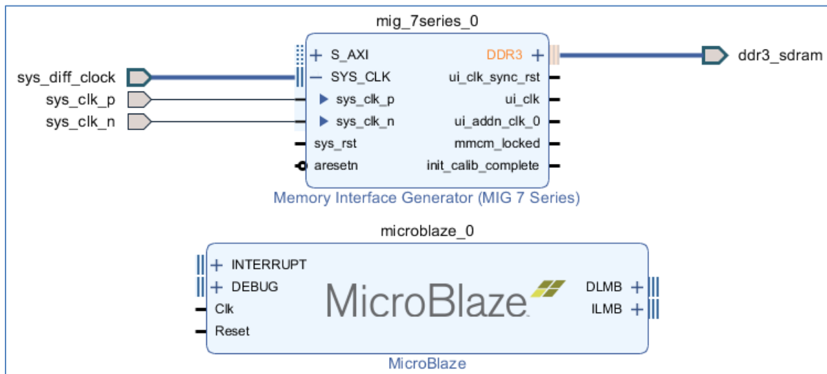
Figure 88: Block Design After Instantiating the Memory IP Core
