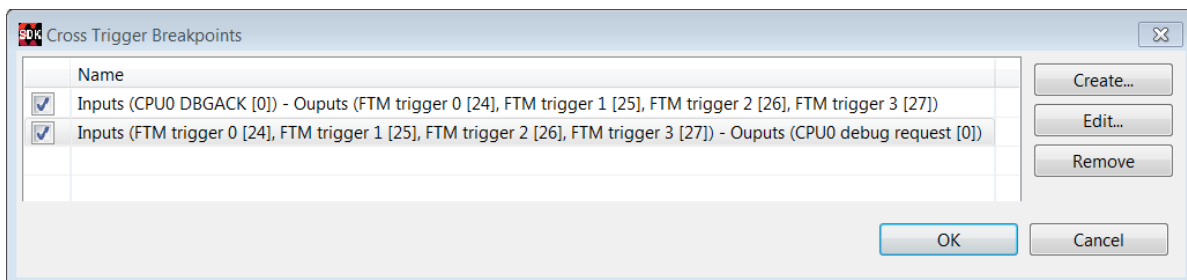
Figure 67: Cross Trigger Breakpoints dialog box showing the selection for breakpoint
