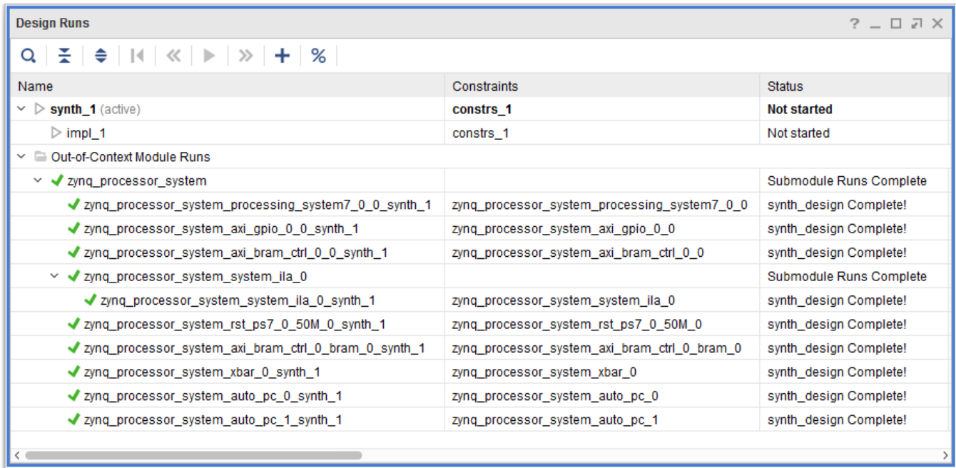
Figure 54: Design Runs window showing the status of Out-of-Context Module Runs
