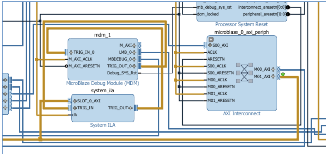
Figure 99: ILA connections to the Cross-Trigger Interface
