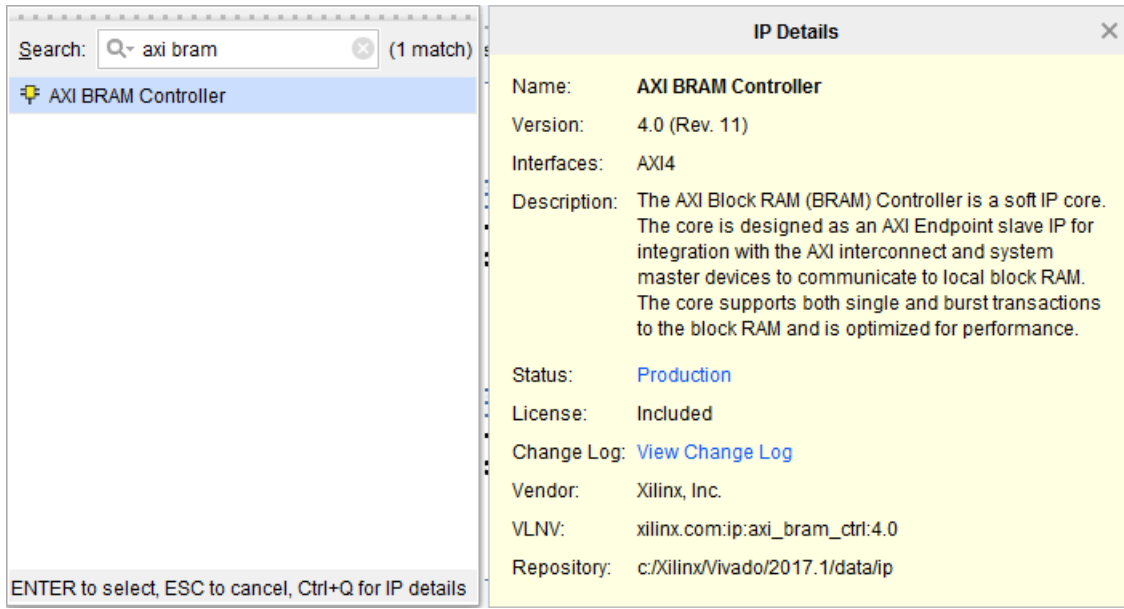
Figure 91: Add BRAM Controller
