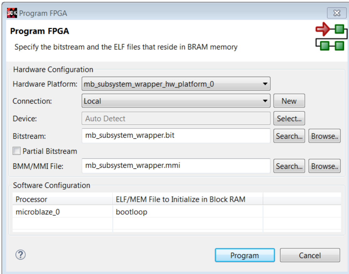
Figure 115: Program FPGA Dialog Box
