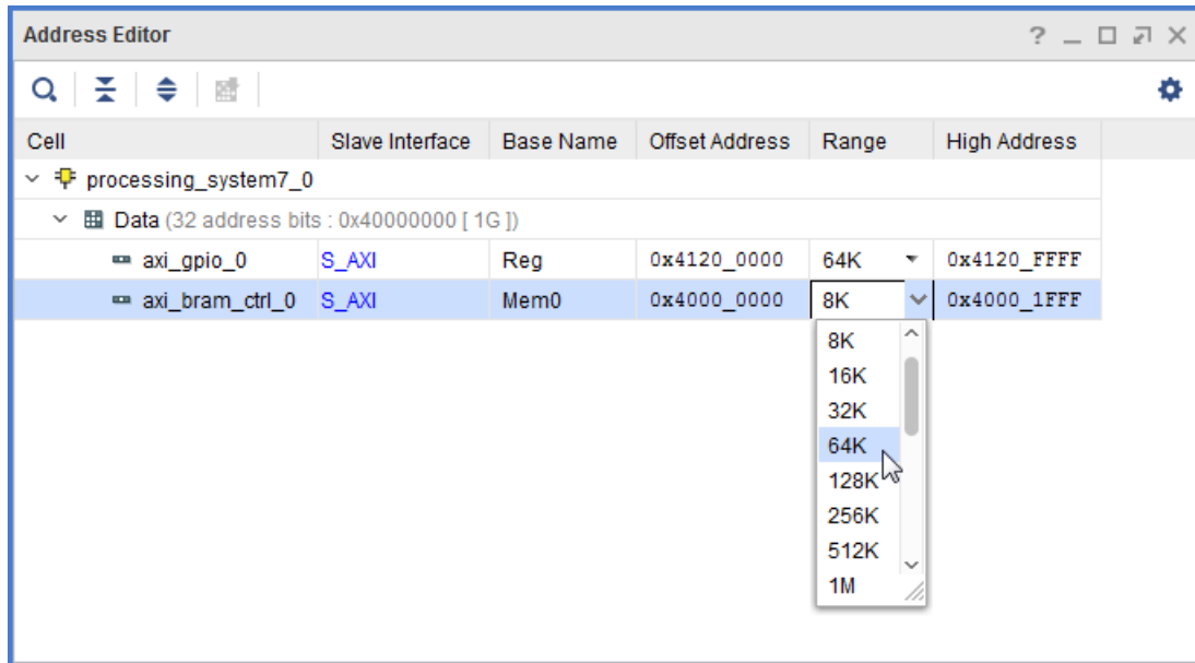
Figure 16: Change Range of axi_bram_ctrl to 64K
