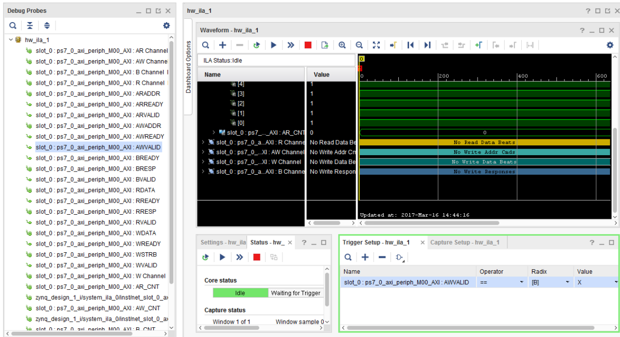
Figure 38: The ILA Properties window
