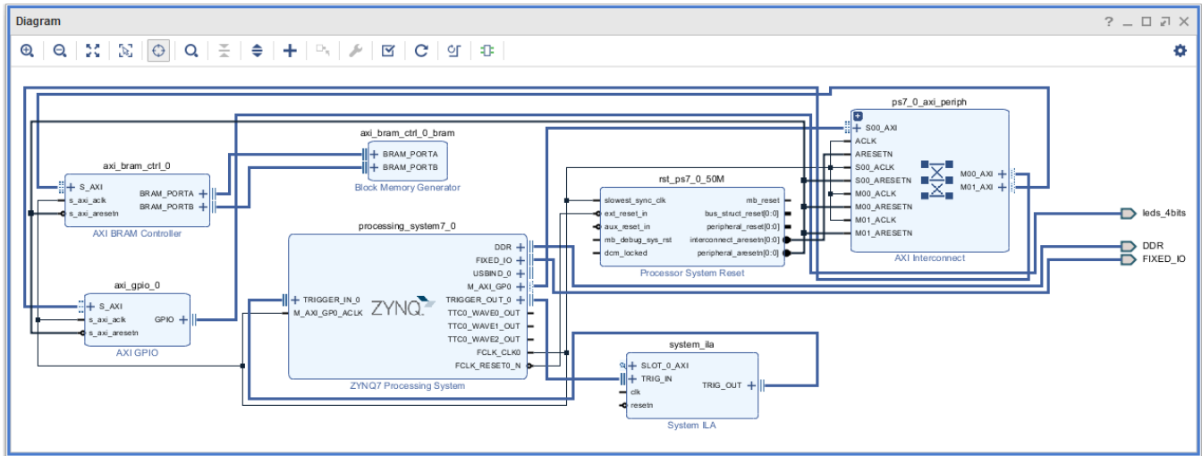
Figure 49: Design after Running Connection Automation
