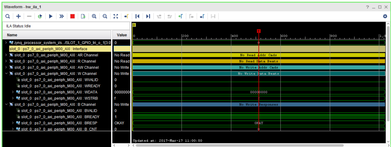
Figure 81: PS to PL Cross Trigger Waveform in hw_ila_1
