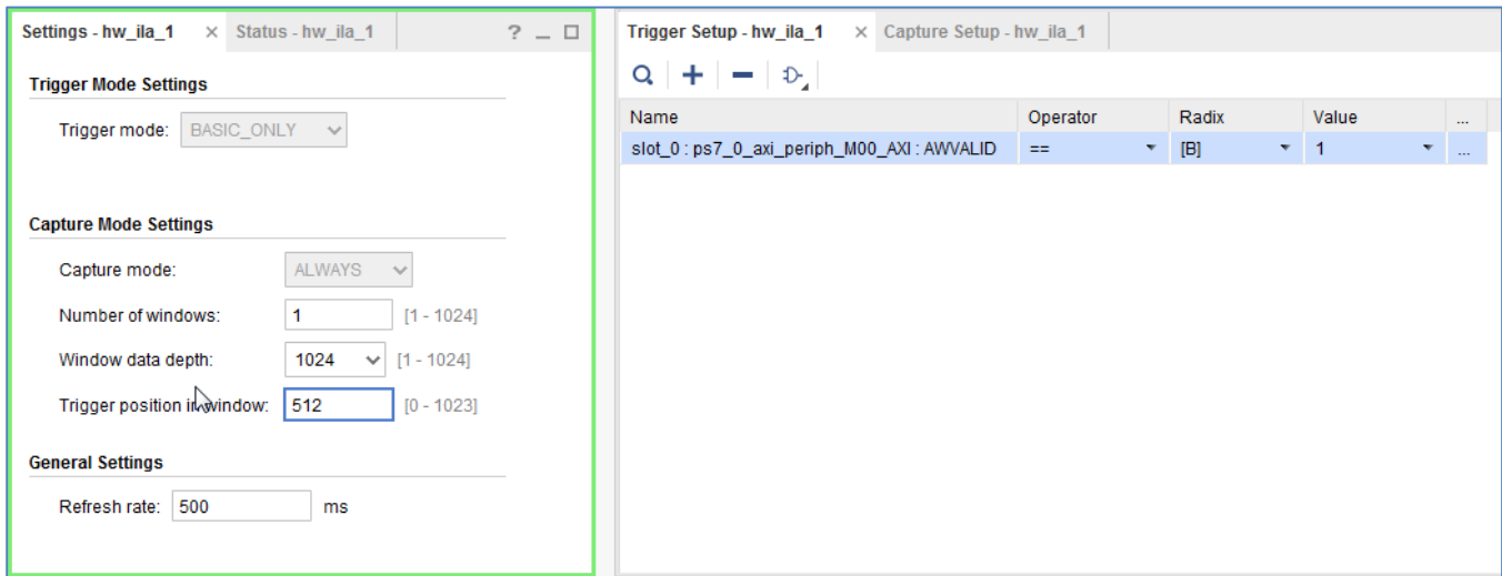
Figure 40: Change Capture Mode Settings
