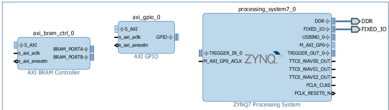
Figure 48: Diagram after Instantiating IP for This Design
