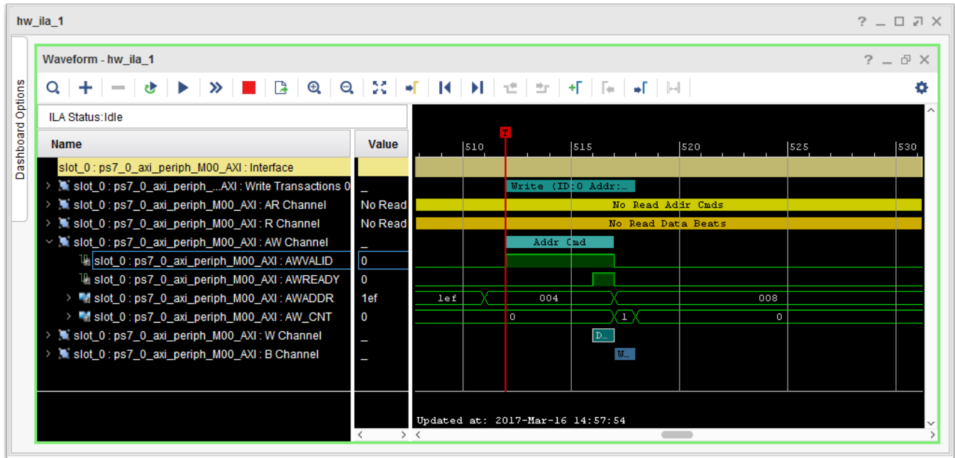
Figure 42: Trigger Mark Goes to 1
