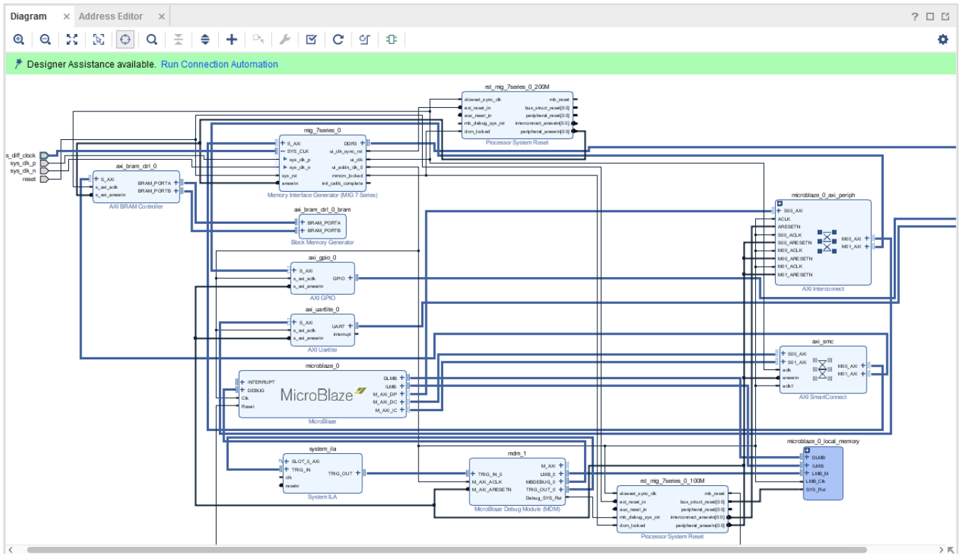
Figure 97: MicroBlaze Connected to UART, GPIO and AXI Timer
