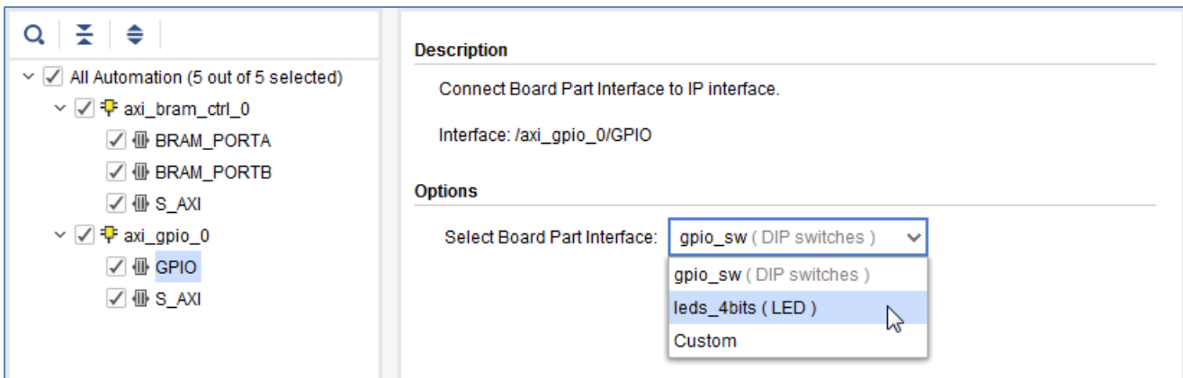
Figure 13: Select leds_4bits as for GPIO interface of axi_gpio_0
