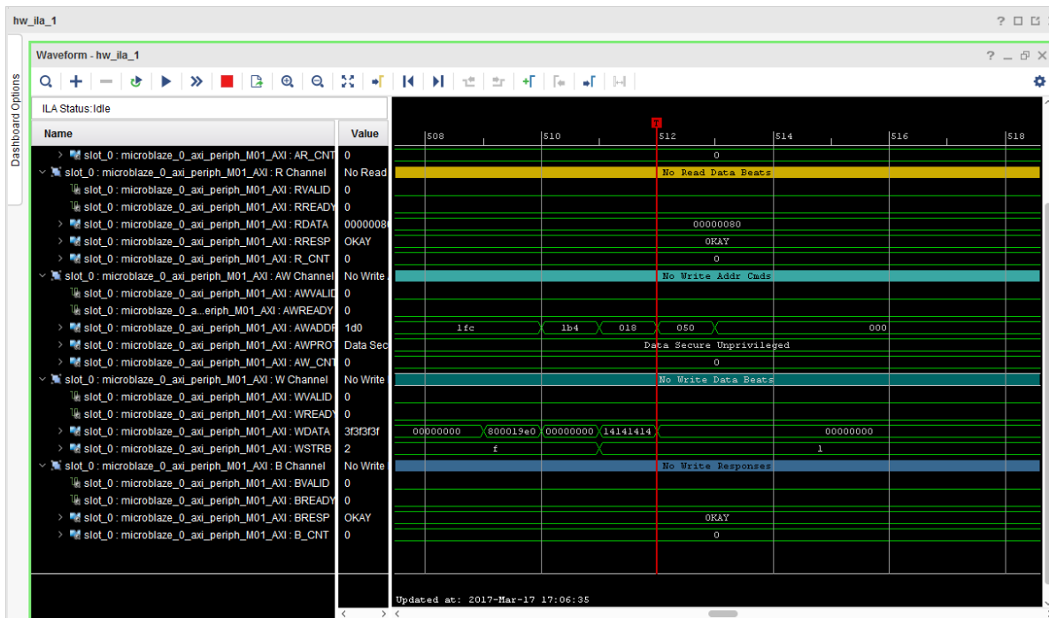
Figure 130: MicroBlaze to Logic Cross Trigger Waveform in hw_ila_1
