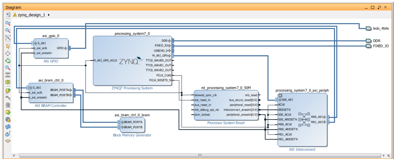
Figure 16: Zynq-7000 AP SoC Processor System
