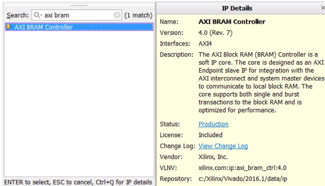
Figure 107: Add BRAM Controller
