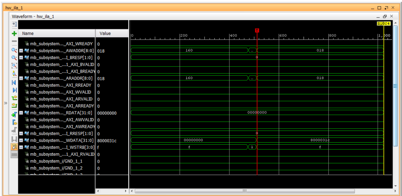
Figure 163: MicroBlaze to Logic Cross Trigger Waveform in hw_ila_1
