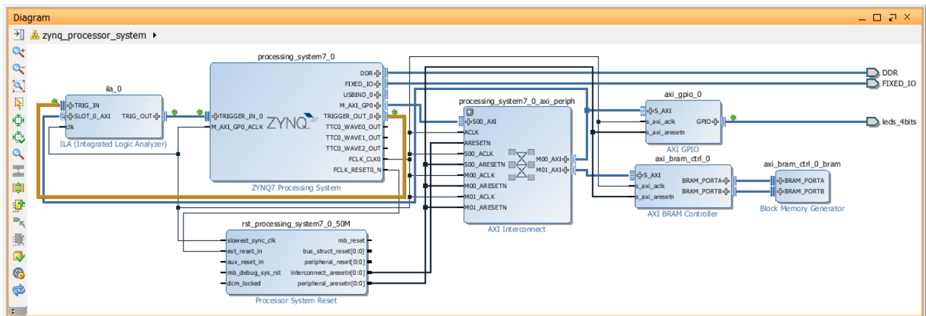
Figure 59: Block Design after Running Regenerate Layout
