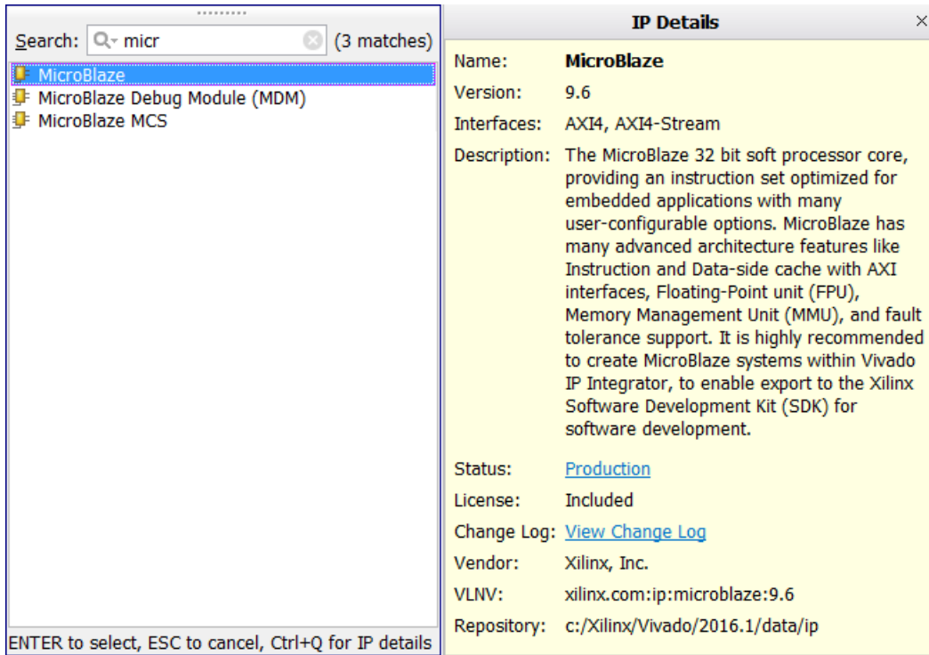
Figure 101: Search Field
