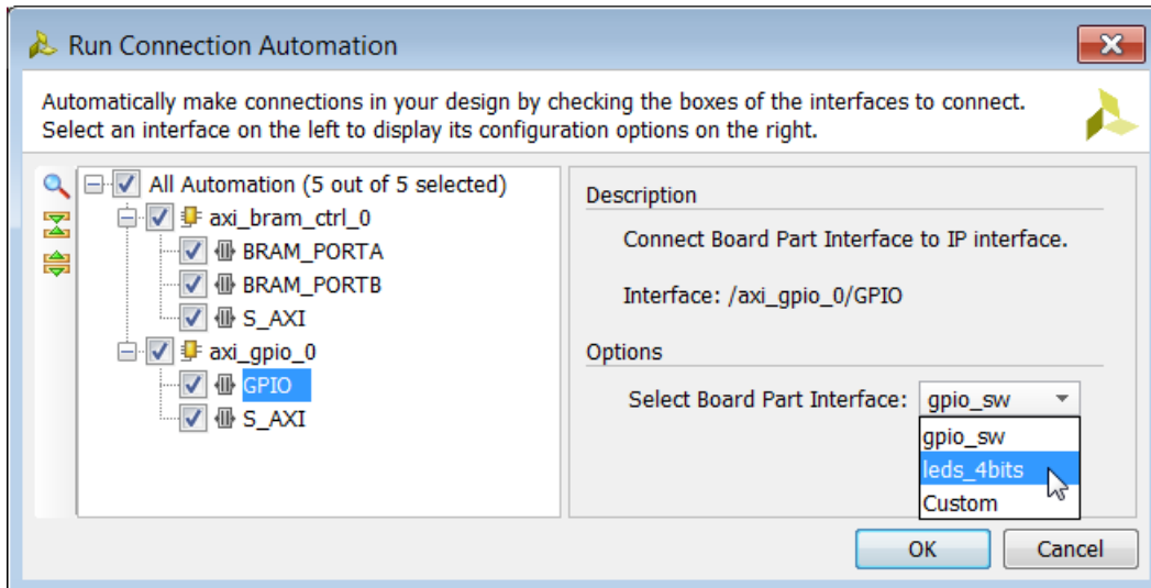
Figure 14: Run Connection Automation Dialog Box for GPIO Interface of axi_gpio_0
