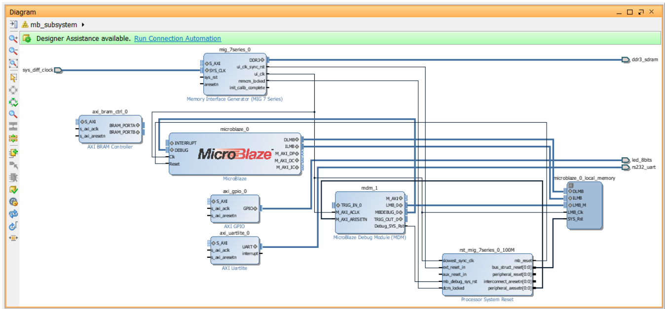
Figure 110: MicroBlaze System
