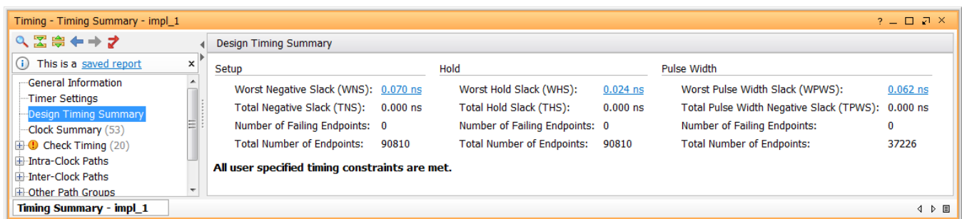
Figure 135: Timing Summary
