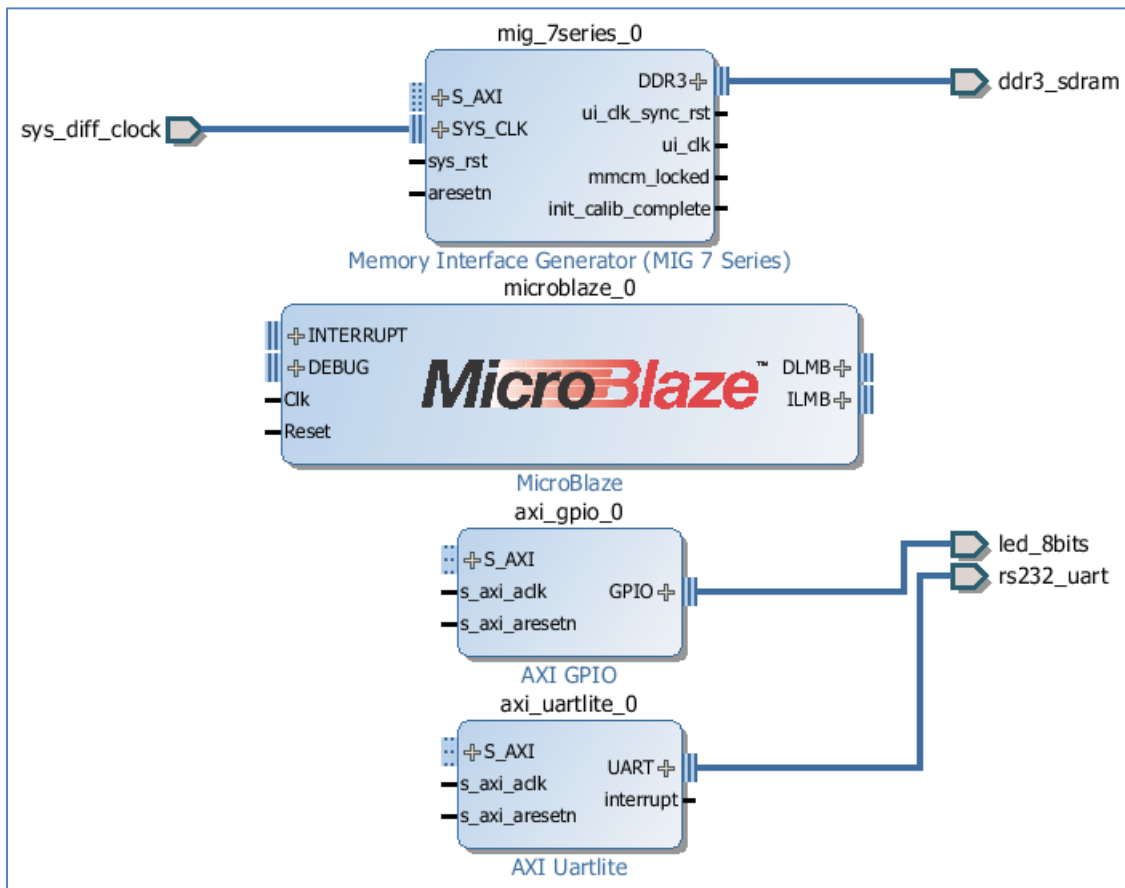
Figure 106: Block Design After Connecting the rs232_uart and the led_8bits Interfaces
