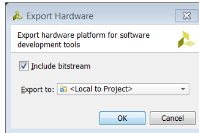
Figure 32: Export Hardware for SDK
