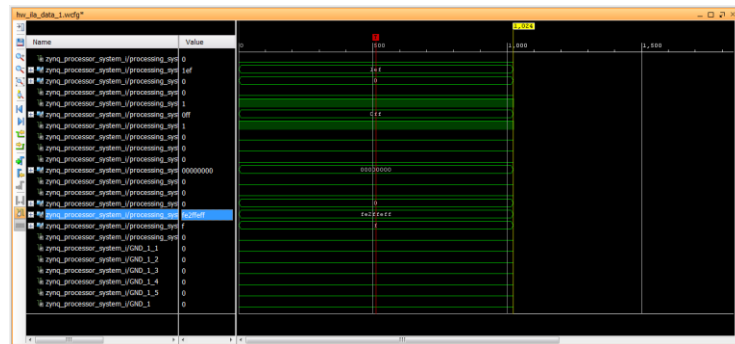
Figure 95: PS to PL Cross Trigger Waveform in hw_ila_1
