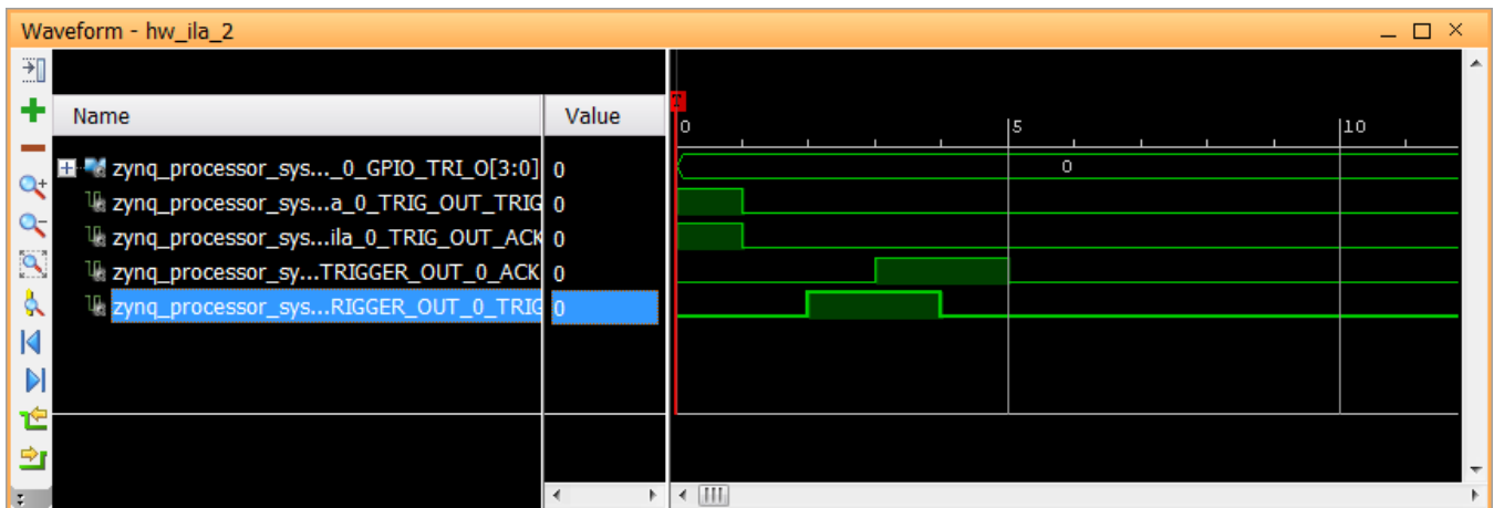
Figure 96: Waveform Demonstrating PS to PL Trigger
