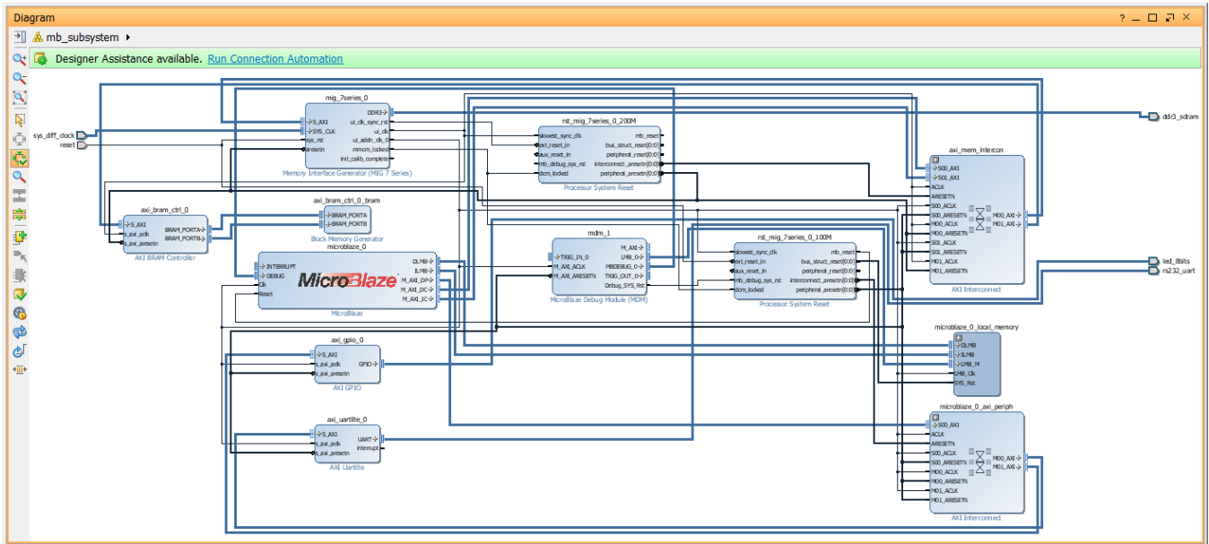
Figure 113: MicroBlaze Connected to UART, GPIO and AXI Timer
