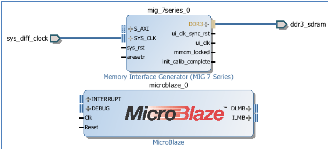
Figure 104: Block Design After Instantiating the Memory IP Core
