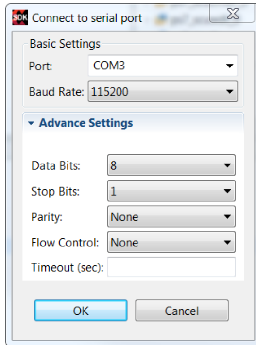
Figure 79: Terminal Settings
