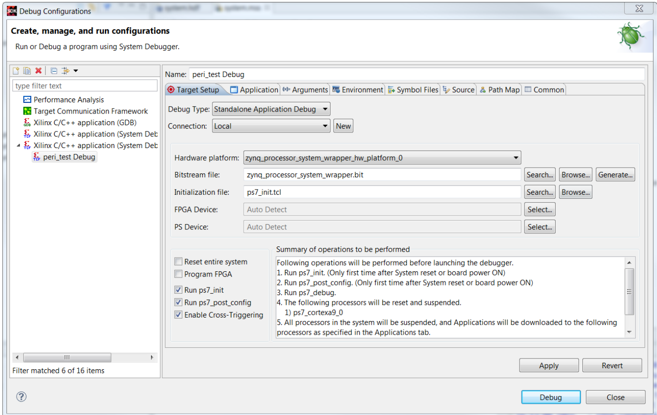
Figure 78: Enable Cross-Triggering
