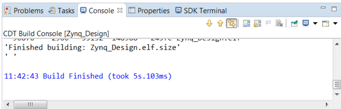
Figure 36: SDK Message
