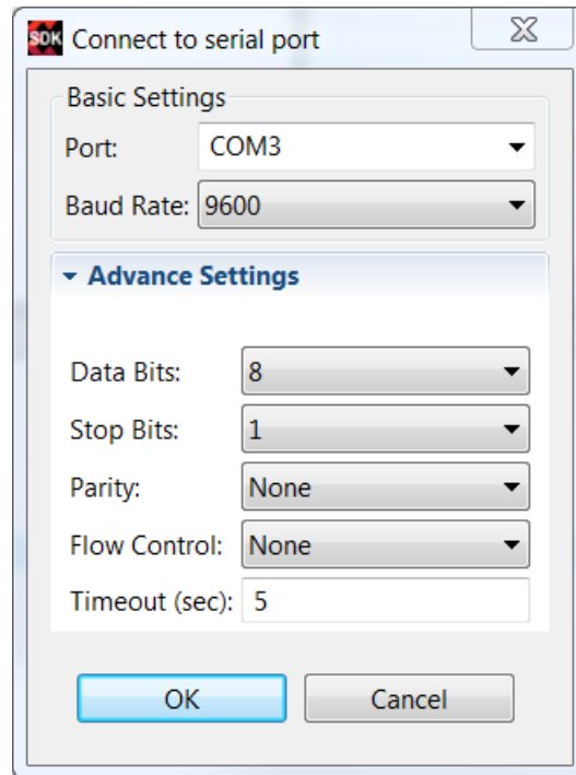
Figure 147: Terminal Settings
