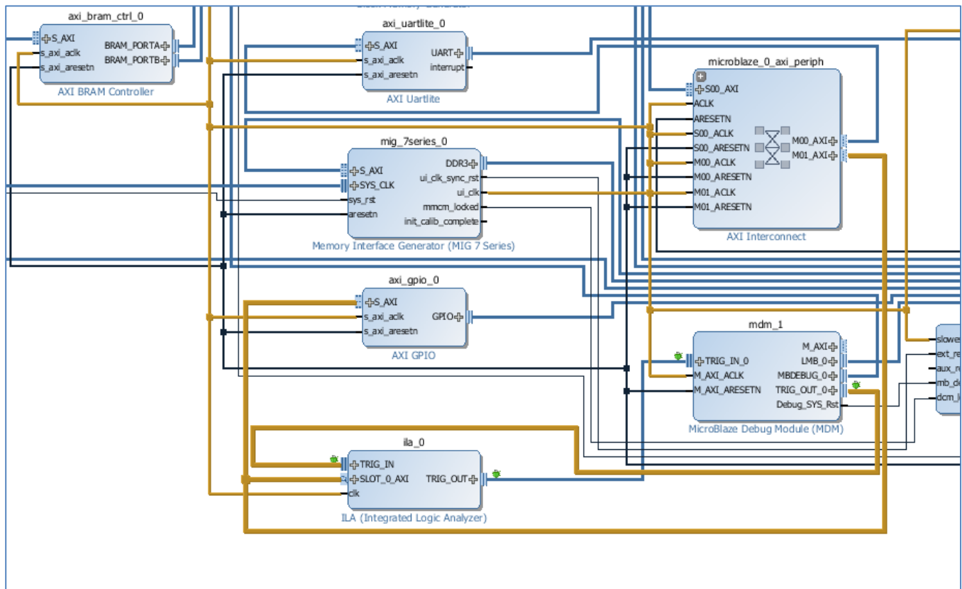
Figure 117: ILA connections to the Cross-Trigger Interface
