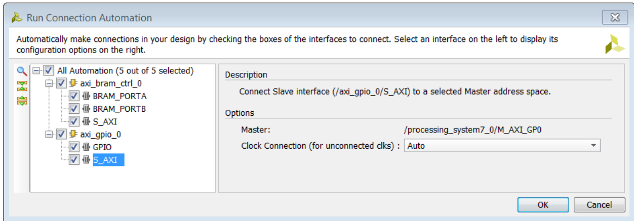
Figure 15: S_AXI Interface Options for axi_gpio_0
