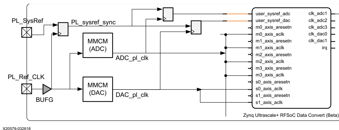
Figure 3-19: PL SYSREF Capture
