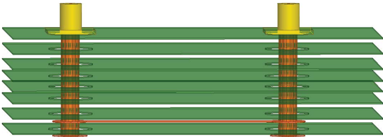
Figure 2-2: Layer 14 Routing Example
