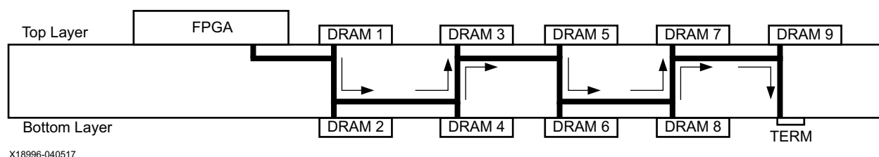
Figure 2-22: Address/Command/Control Topology for DDR4 SDRAM Clamshell
