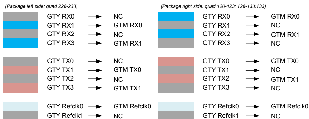
Figure 9-7: VU13P/VU29P D2104 GTY/GTM TX/RX Channel/Clock Mapping
