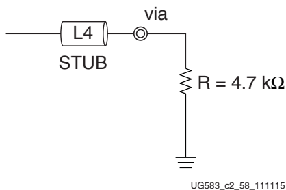
Figure 2-27: Termination for reset_n in DDR3 DRAM
