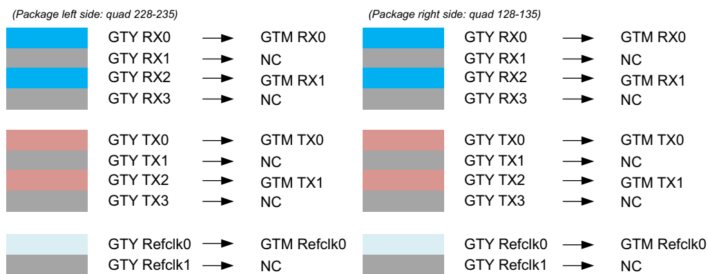
Figure 9-8: VU13P/VU27P A2577 GTY/GTM TX/RX Channel/Clock Mapping
