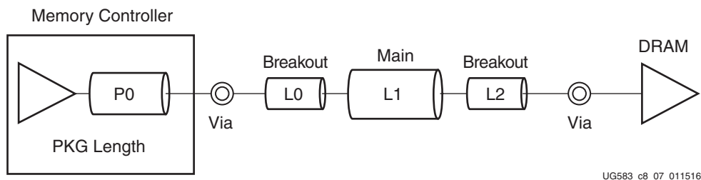
Figure 2-40: DQ and DM Routing for LPDDR4 without ECC
