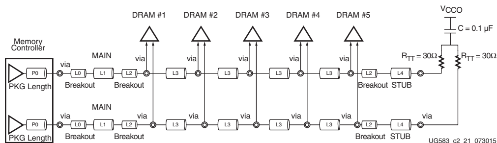
Figure 2-28: Clock Fly-by Termination for DDR3 SDRAM
