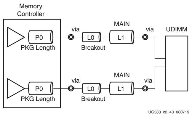
Figure 2-30: CK Point-to-Point Routing for DDR3/DDR4 DIMM Topology
