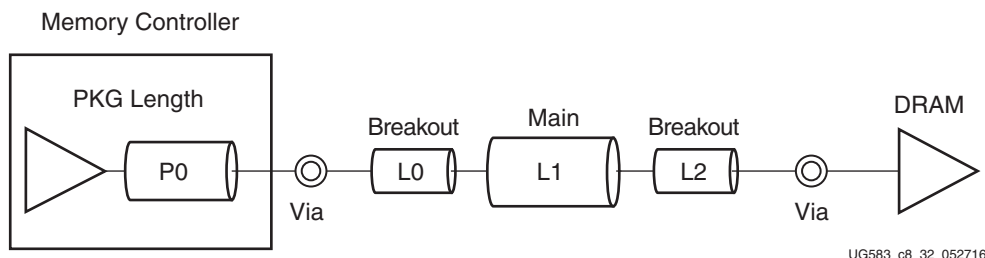
Figure 2-54: Data Signals Point-to-Point for LPDDR3 SDRAM
