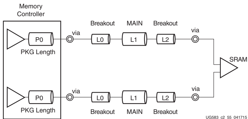
Figure 2-75: DK and CK Routing for QDR-IV SRAM
