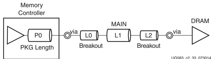
Figure 2-64: Data Signals Point-to-Point Routing
