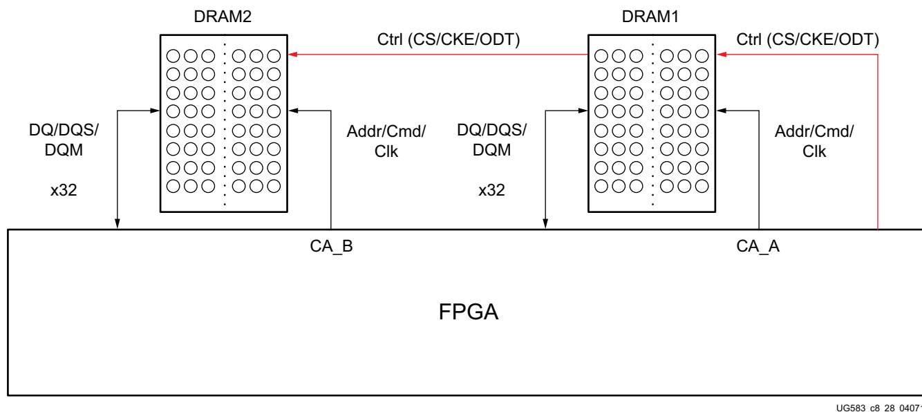
Figure 2-50: Design Example for Two-Component x64 LPDDR3 SDRAM
