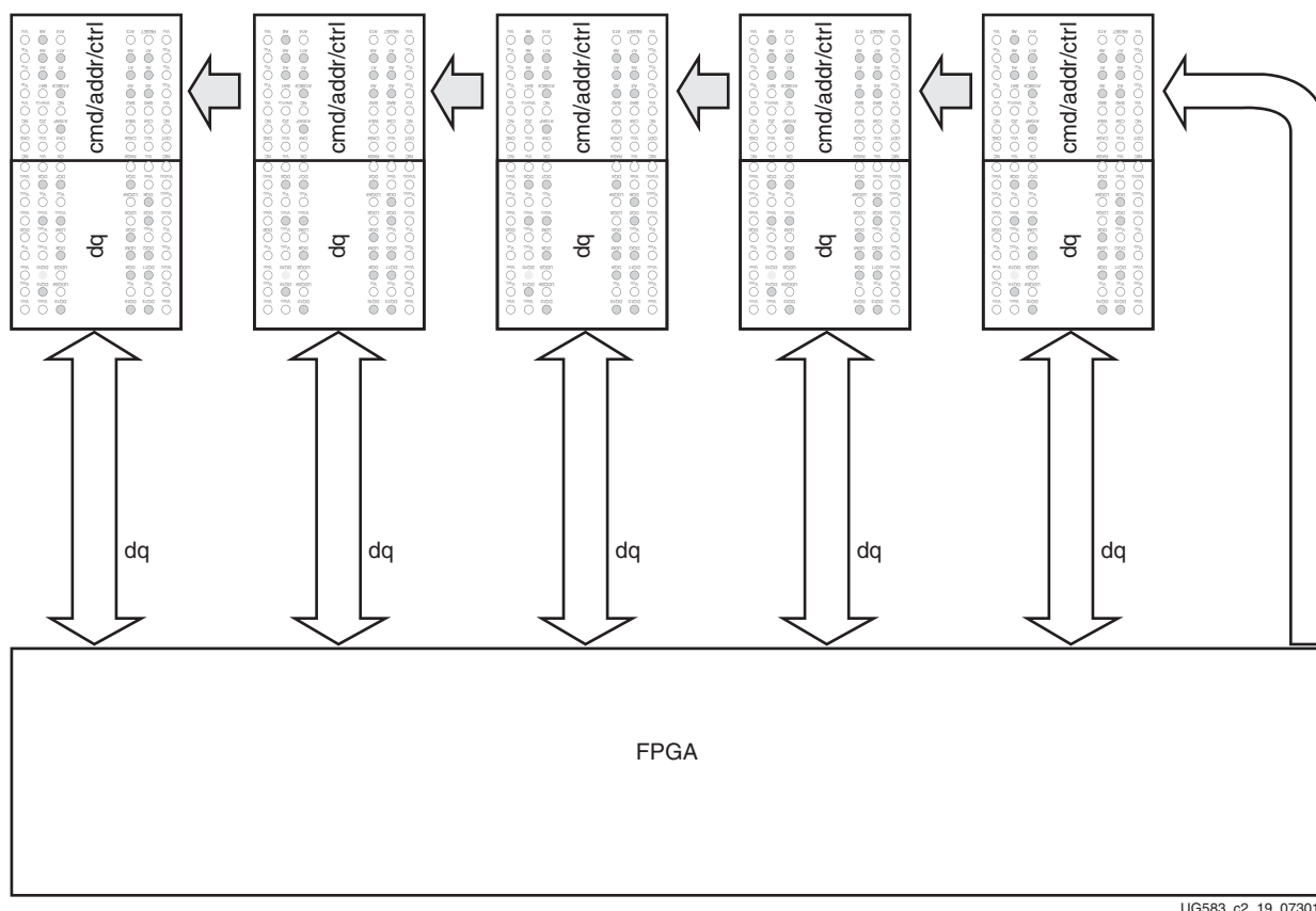
Figure 2-17: Component Placement Recommendations for Five Components
