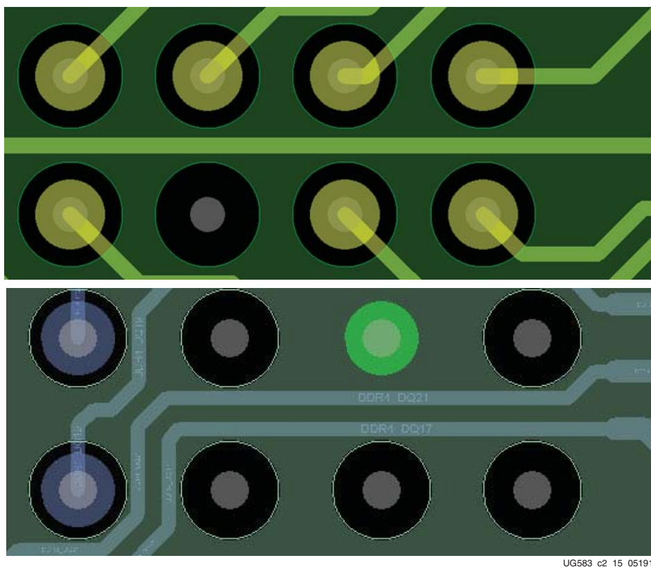
Figure 2-10: Breakout Region Routing
