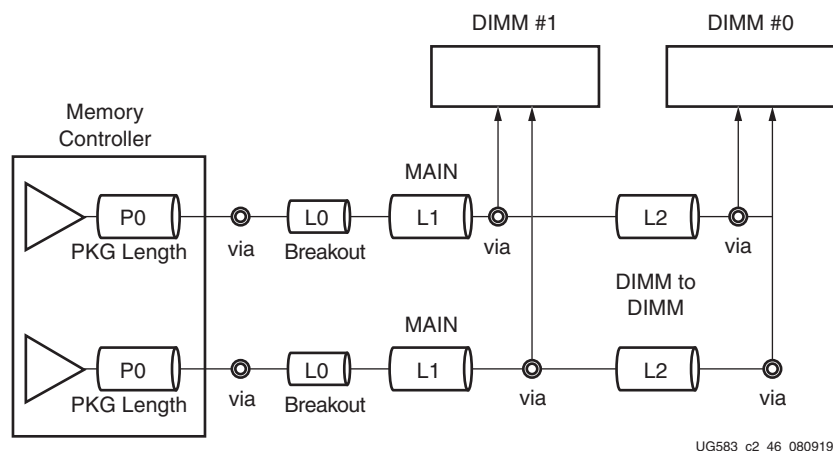
Figure 2-34: DQS Fly-by Routing for DDR3/DDR4 DIMM Topology
