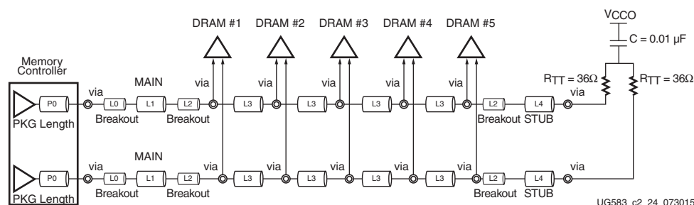
Figure 2-23: Clock Fly-by Termination for DDR4 SDRAM
