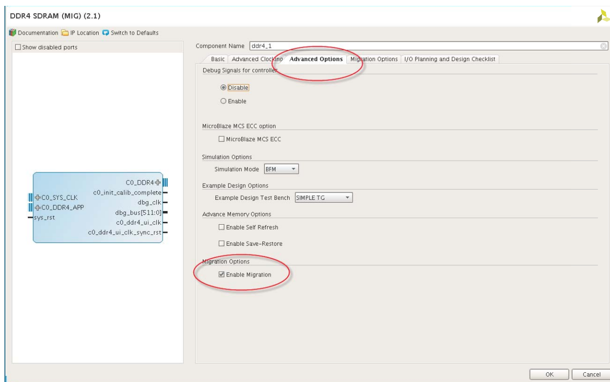
Figure 8-9: Selecting the Enable Migration Feature for DDR4 Designs
