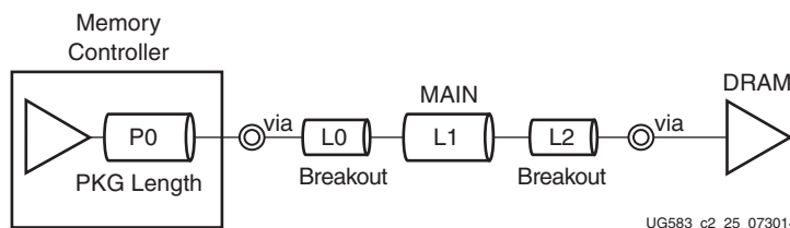
Figure 2-25: Data Signals Point-to-Point for DDR4 SDRAM
