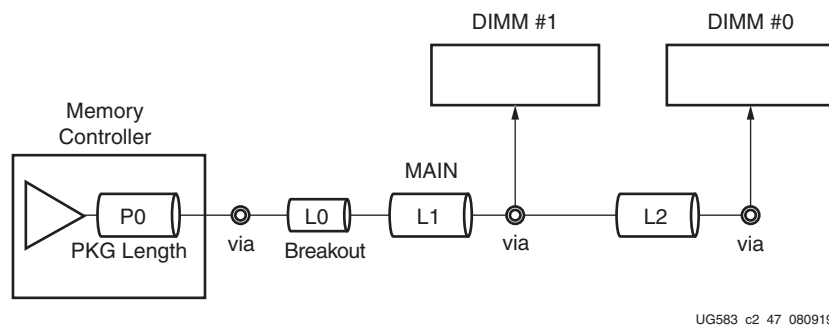
Figure 2-35: DQ Fly-by Routing for DDR3/DDR4 DIMM Topology
