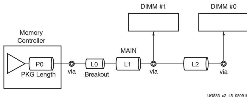
Figure 2-32: CMD/ADDR Fly-by Routing for DDR3/DDR4 DIMM Topology
