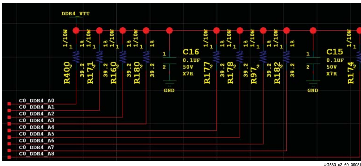
Figure 2-15: Schematic Example of VTT Resistor and Capacitor Connections
