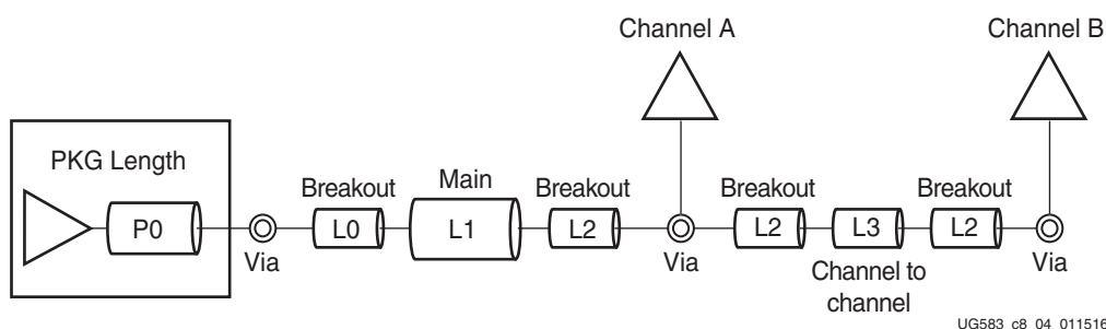
Figure 2-37: Chip Select Routing for LPDDR4 without ECC
