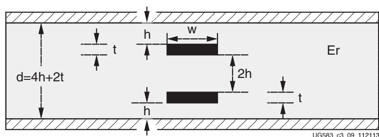
Figure 11-9: Centered Broadside-Coupled Stripline
