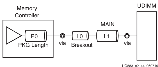
Figure 2-31: CTRL Point-to-Point Routing for DDR3/DDR4 DIMM Topology
