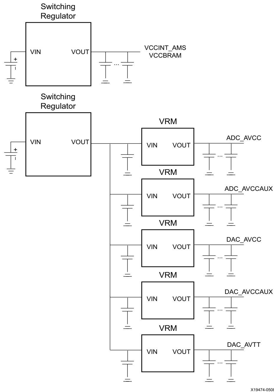
Figure 3-32: Power Regulation for Analog Supplies
