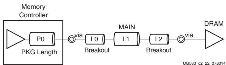
Figure 2-29: Data Signals Point-to-Point for DDR3 SDRAM
