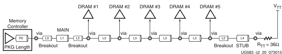
Figure 2-26: Address Fly-by Termination for DDR3 SDRAM
