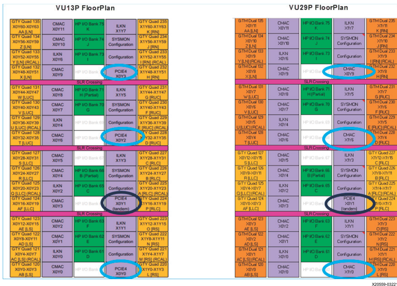
Figure 9-5: VU13P Floorplan with PCIe/GTY versus VU29P Floorplan with CMAC/GTM
