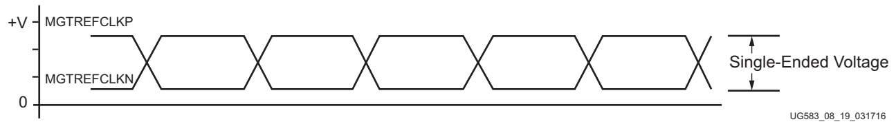
Figure 4-2: Single-Ended Clock Input Voltage Swing, Peak-to-Peak
