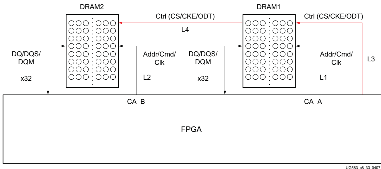
Figure 2-55: LPDDR3 x64 Two-SDRAM System
