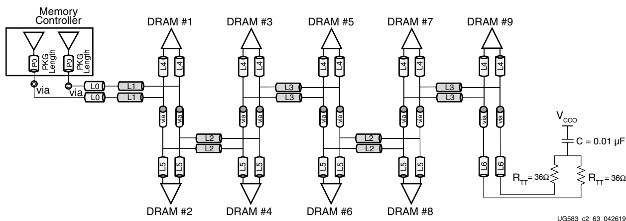
Figure 2-24: Clock Topology for DDR4 SDRAM Clamshell
