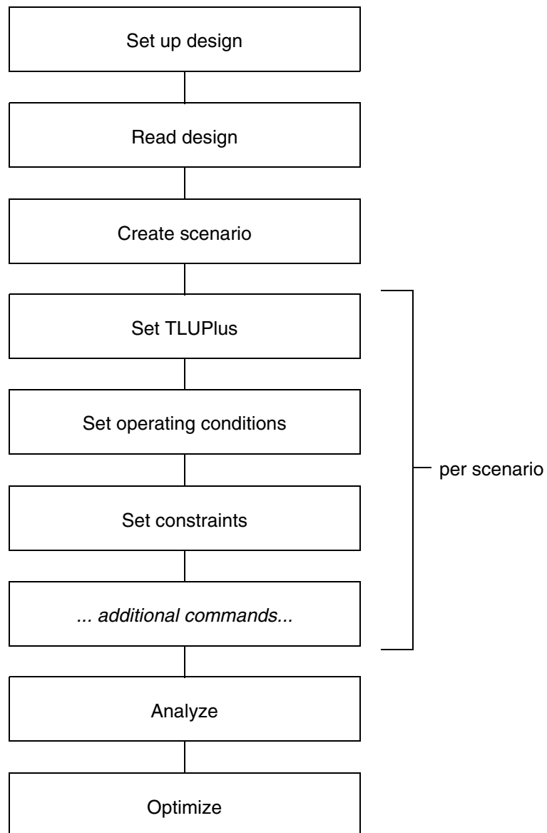
Figure 10-24 Basic Multimode Flow
