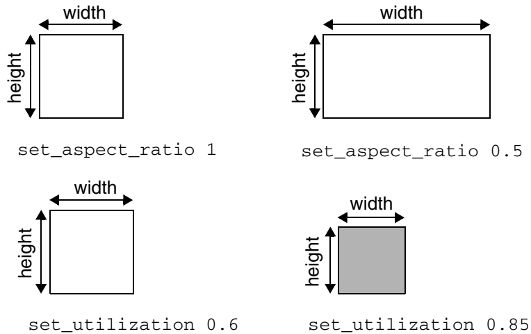
Figure 10-3 Defining Relative Core Area and Shape
