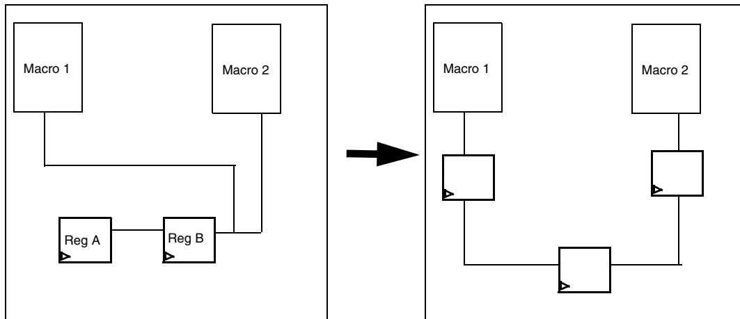
Figure 12-1 Register Replication Example
