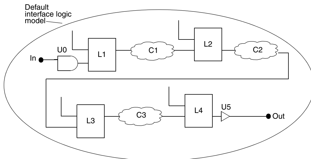
Figure 9-2 Interface Logic Model Default Model and Latch Levels
