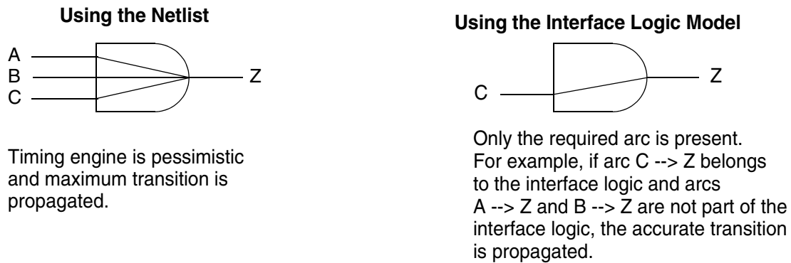
Figure 9-5 Comparison of Timing Propagation Between Netlist and Model
