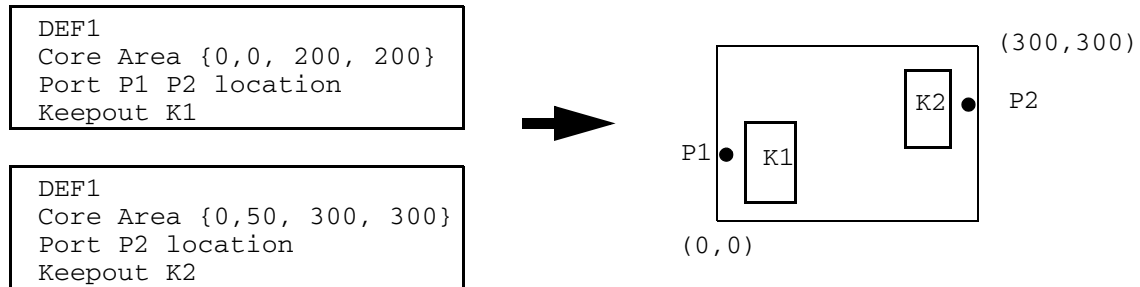
Figure 10-18 Incremental Extraction with the extract_physical_constraints command
