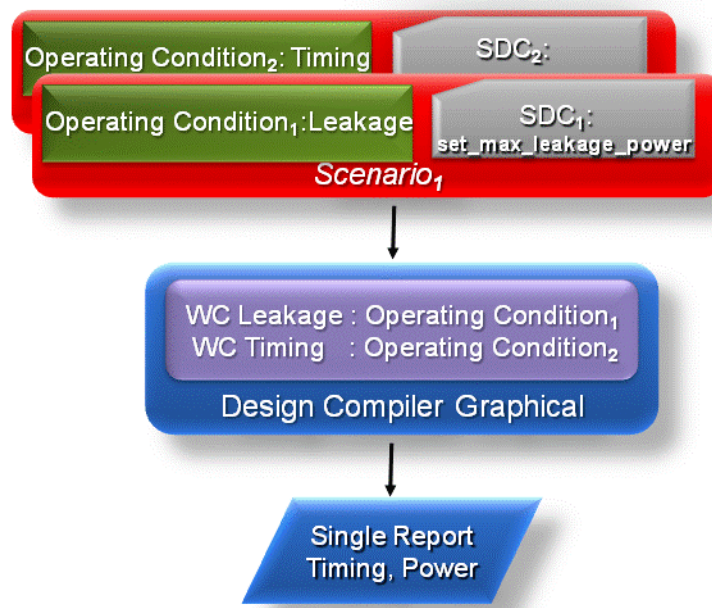
Figure 10-25 Setting Different Constraints on Different Scenarios
