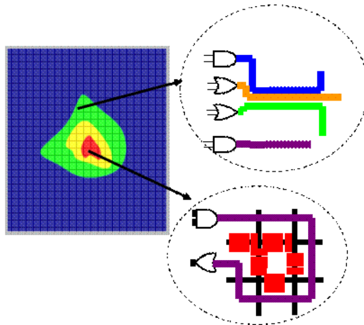
Figure 10-21 Predicting Congestion Using Virtual Grid Route
