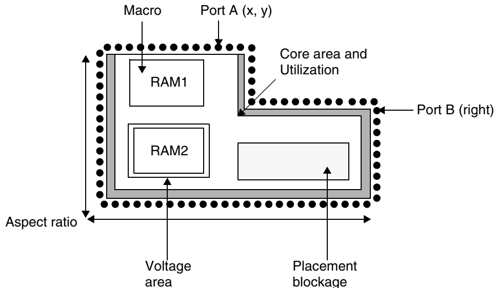
Figure 10-2 Supported Physical Constraints
