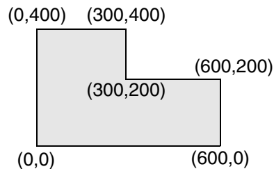
Figure 10-5 Defining Exact Rectilinear Core Area And Shape
