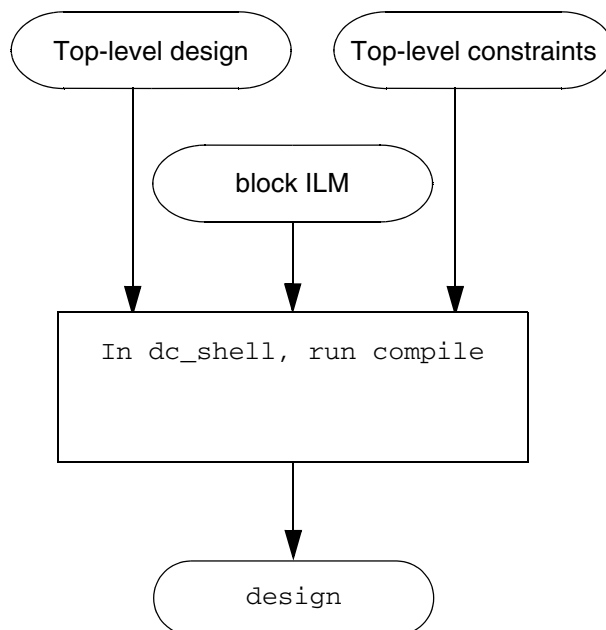
Figure 9-6 Flow for Instantiating and Using Interface Logic Models
