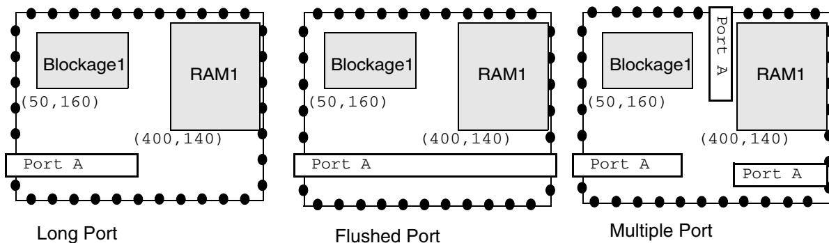
Figure 10-9 Types of Port Dimension Specifications
