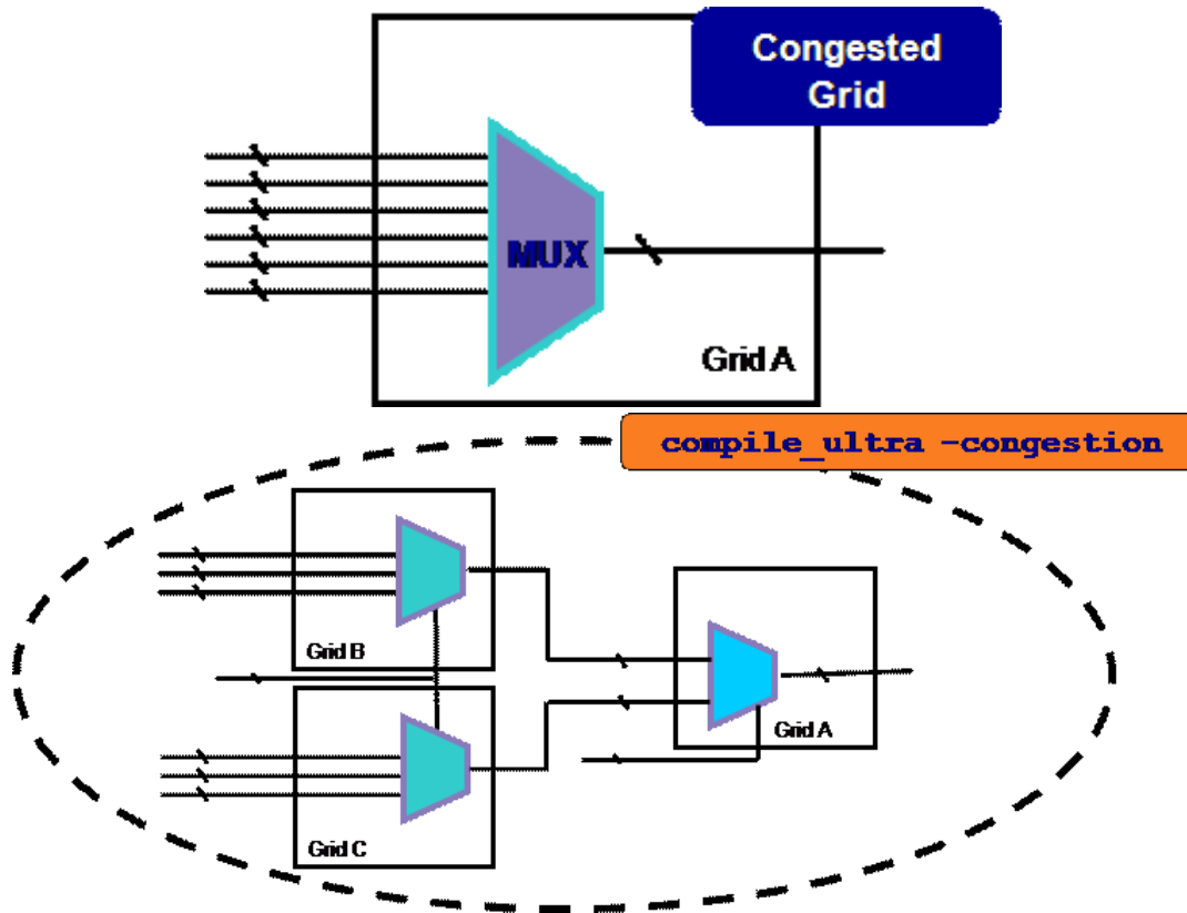
Figure 10-23 Optimizing RTL Structures to Minimize Congestion
