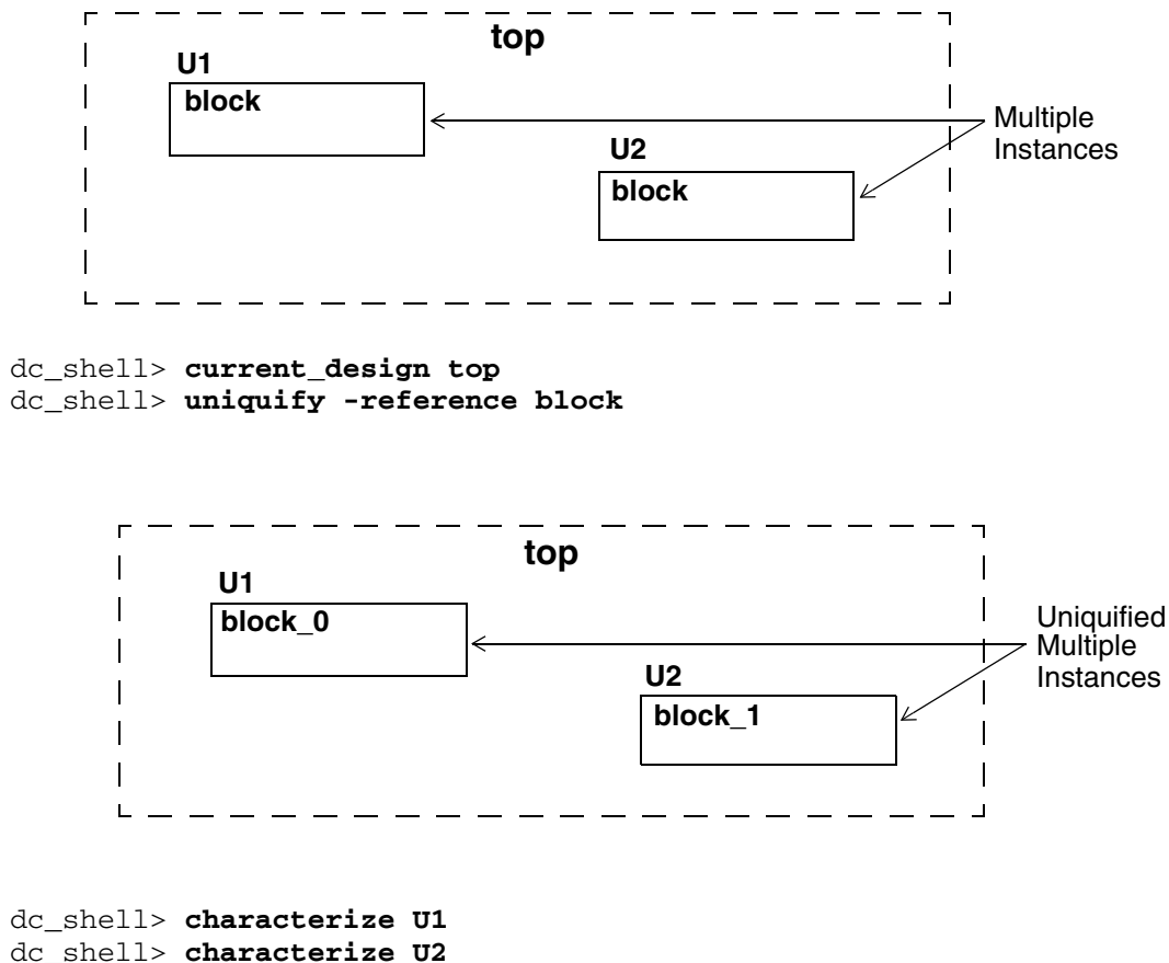
Figure 7-15 Characterizing a Subdesign Referenced Multiple Times
