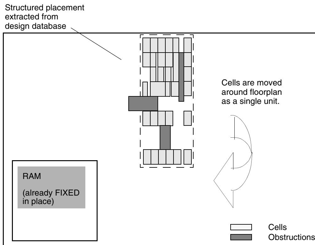
Figure 10-12 Relative Placement in a Floorplan
