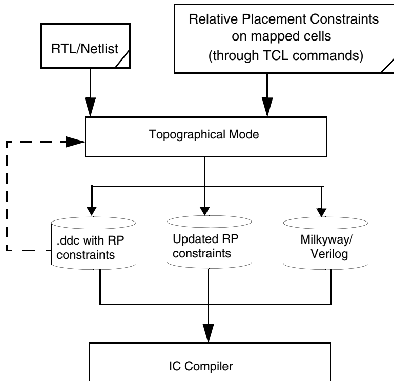
Figure 10-13 Relative Placement Flow
