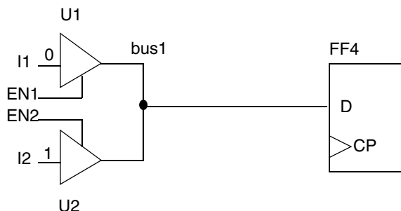
Figure 5-16 Circuit Example
