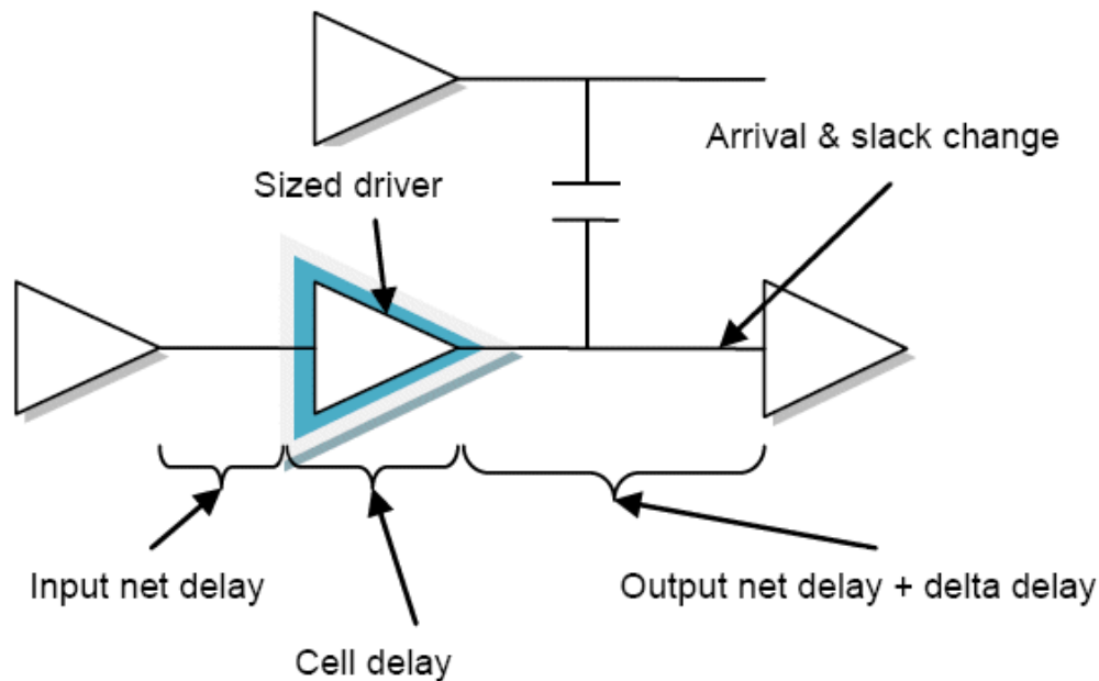
Figure 3-1 Timing Breakdowns
