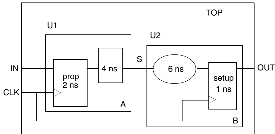
Figure 4-7 50-MHz Design
