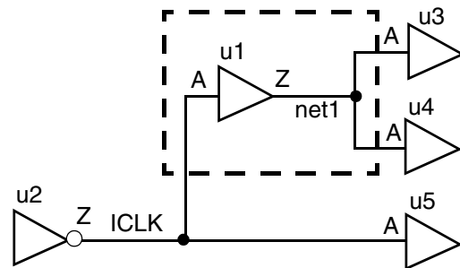
Figure 3-3 New Circuit
