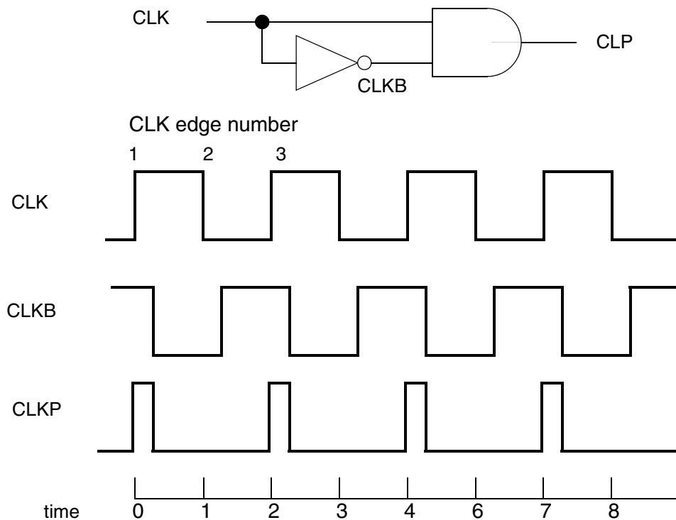
Figure 6-19 Pulse Clock Specified as a Generated Clock
