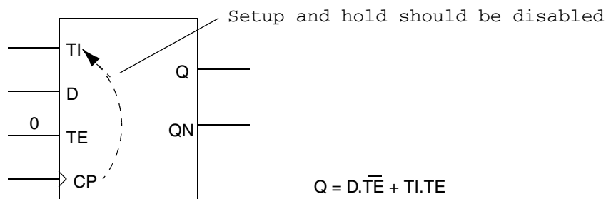
Figure 9-3 Case Analysis Disabling Timing Checks
