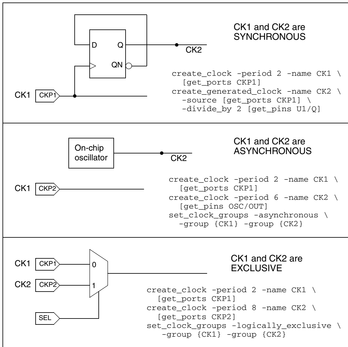
Figure 6-8 Synchronous, Asynchronous, and Exclusive Clocks
