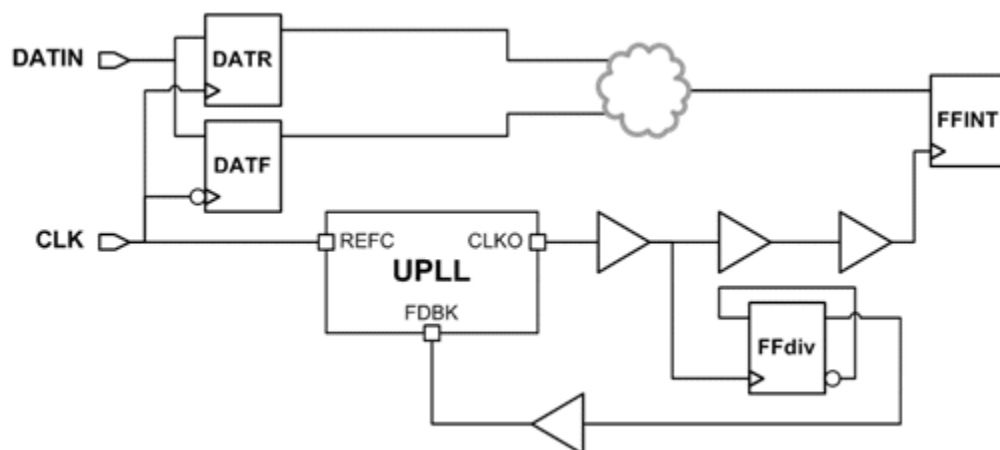
Figure 6-21 Example Circuit
