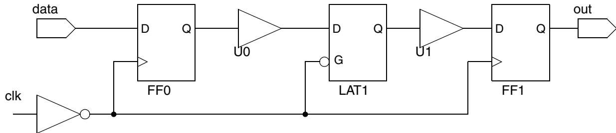
Figure 5-5 Circuit for Path Specification Example 7
