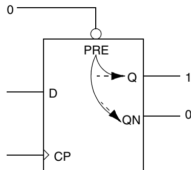
Figure 9-2 Constant Propagation Through an Asynchronous Input
