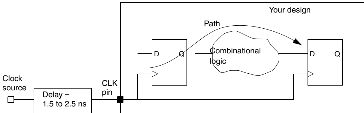
Figure 6-3 External Source Latency
