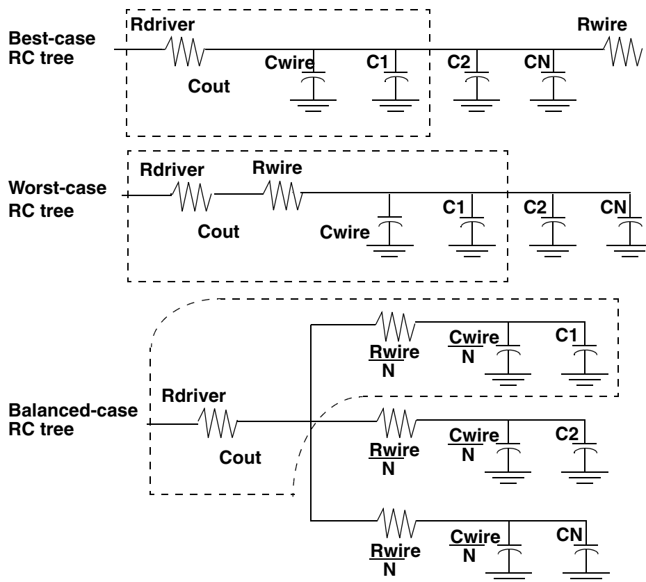
Figure 7-3 RC Interconnect Topologies for Fanout of N
