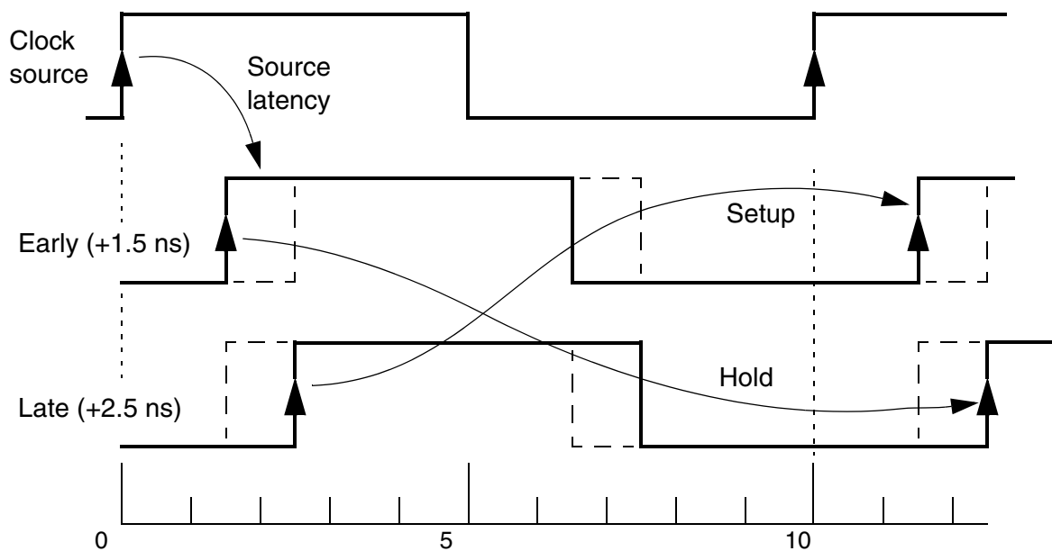
Figure 6-4 Early/Late Source Latency Waveforms
