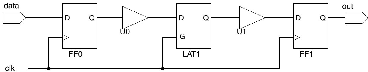
Figure 5-2 Circuit for Path Specification Example 4
