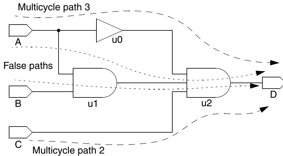
Figure 8-13 Design to Demonstrate Transformed Exceptions
