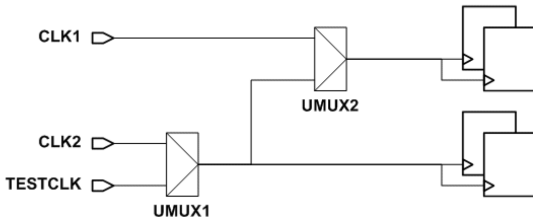
Figure 6-17 Physical Clock Stopping
