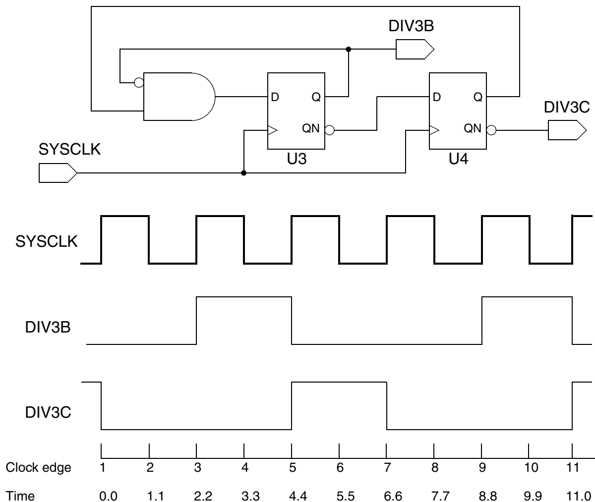
Figure 6-29 Generated Divide-by-3 Clock With Shifted Edges
