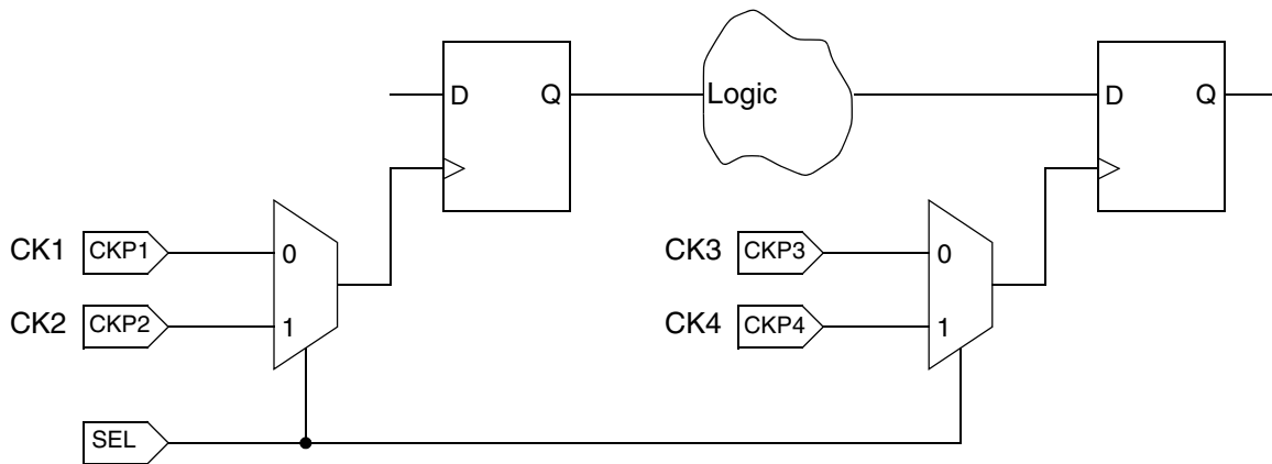
Figure 6-11 Four Clocks and One Selection Signal
