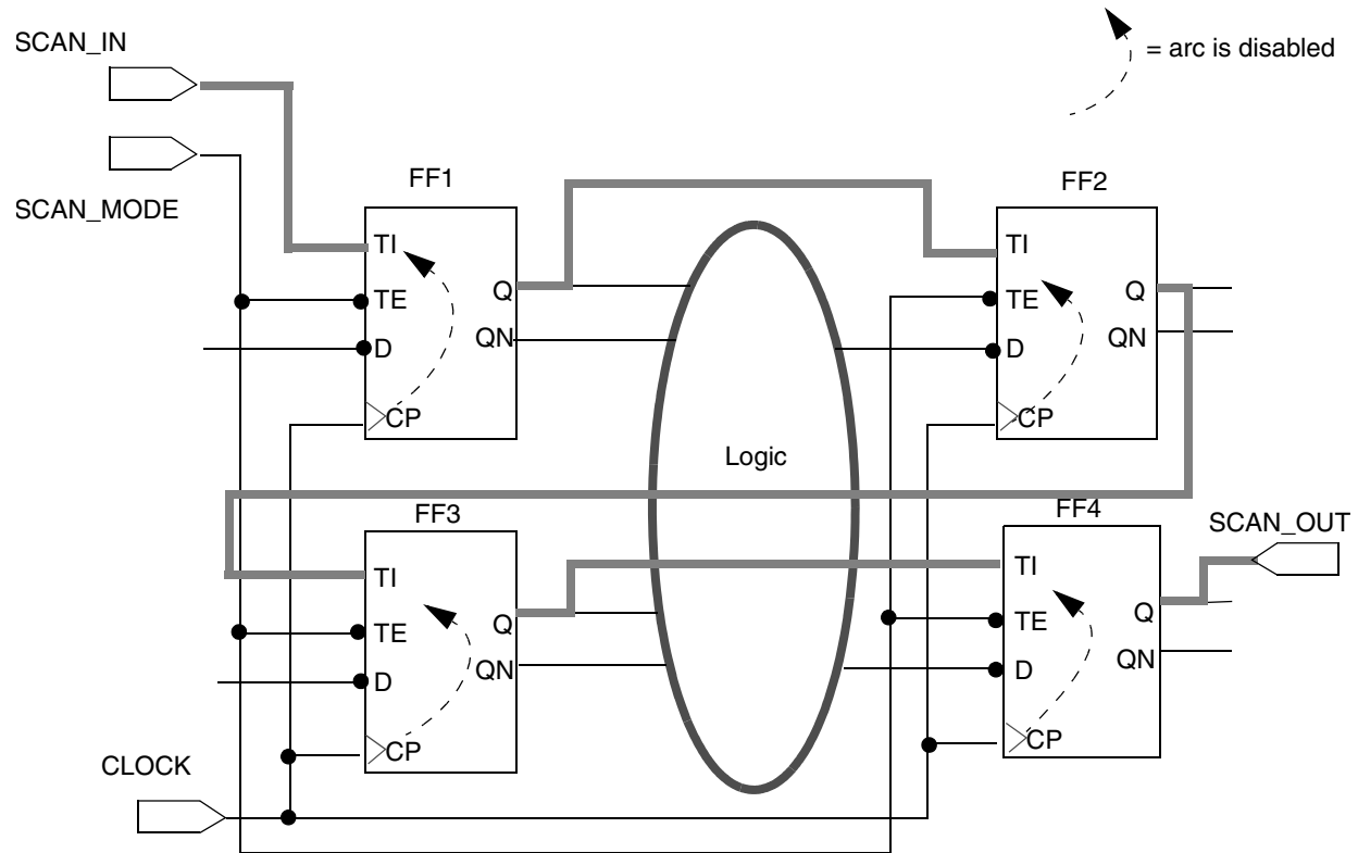
Figure 9-4 Using Case Analysis to Disable a Scan Chain
