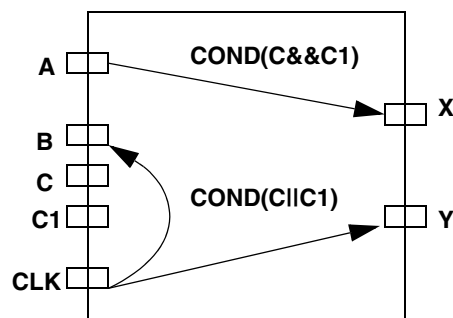
Figure 9-8 Conditional and Nonconditional Arcs
