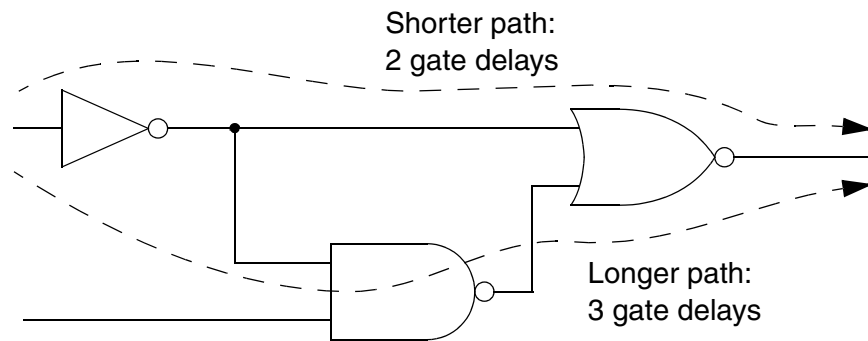
Figure 1-5 Multiple Paths Through Combinational Logic
