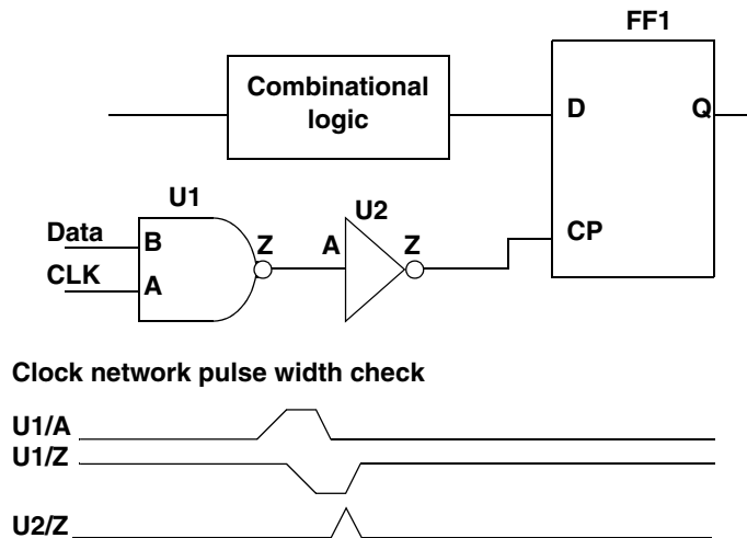
Figure 6-7 Clock Network Pulse Width Check
