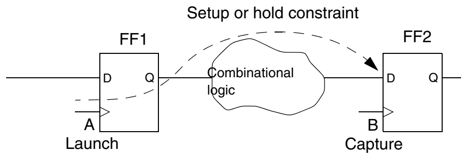
Figure 12-6 Clock Skew Calculation
