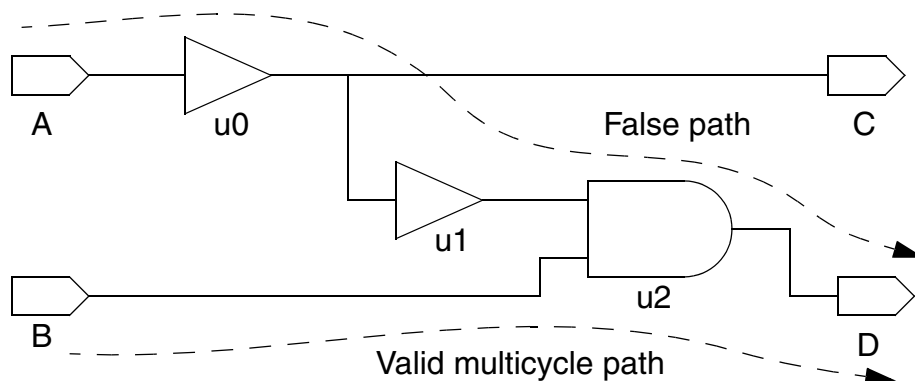
Figure 8-12 Design to Demonstrate Ignored Exceptions
