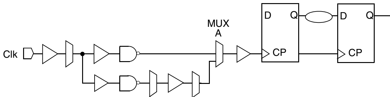
Figure 11-11 Reconvergent Logic in a Clock Network
