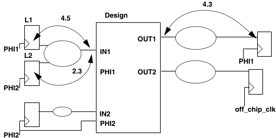
Figure 7-1 Two-Phase Clocking Example for Setting Port Delays
