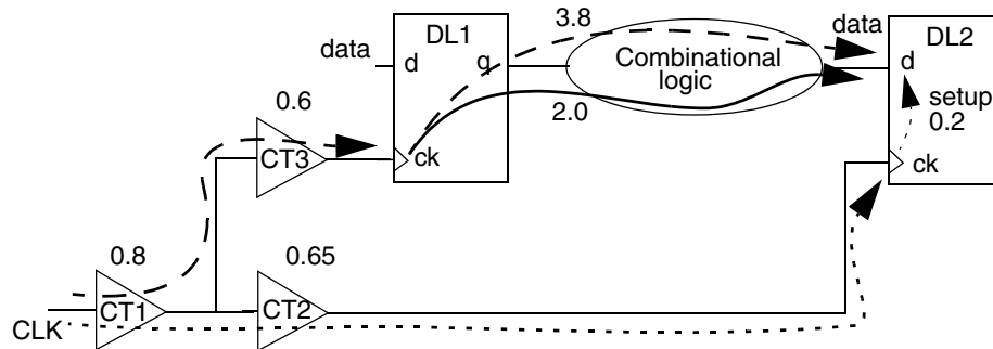
Figure 11-2 Setup Check Using Worst-Case Conditions
