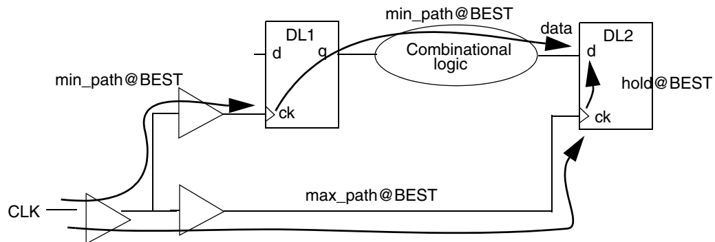
Figure 11-5 Timing Path for One Operating Condition—Best Case
