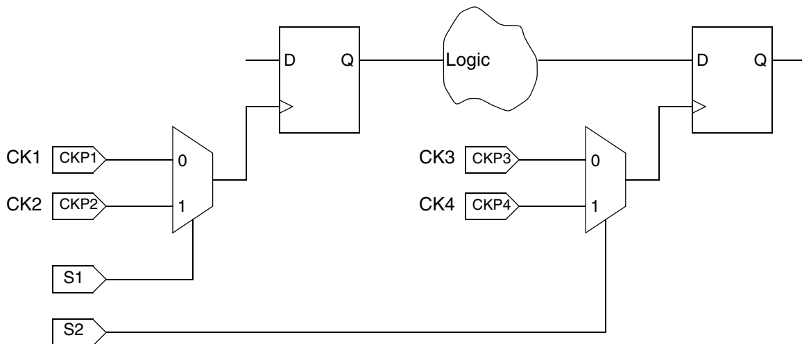
Figure 6-12 Four Clocks and Two Selection Signals
