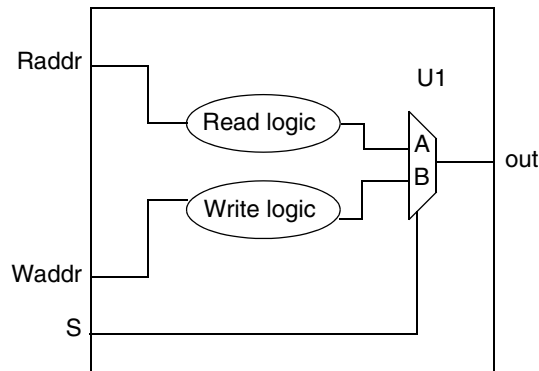
Figure 10-6 Extracting Modes Using the -through Option
