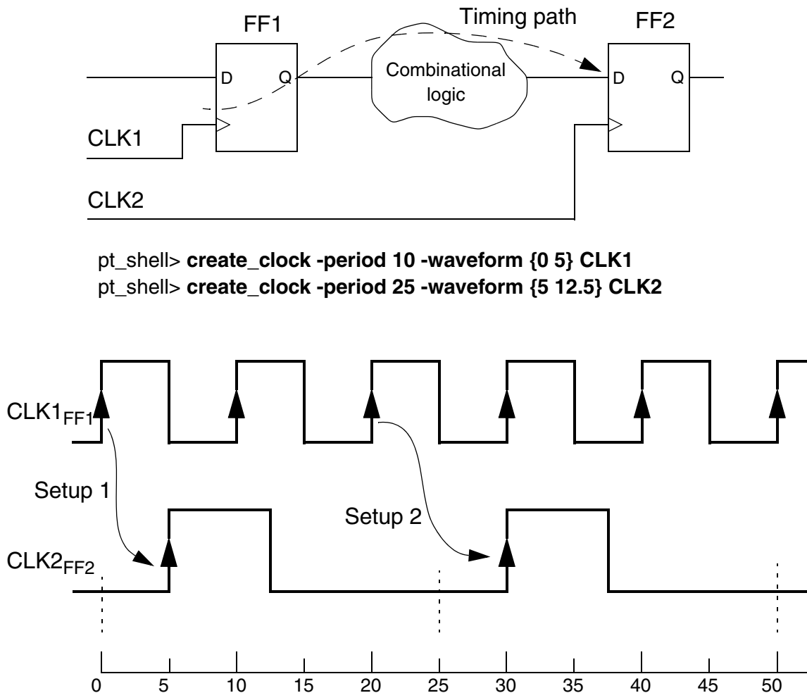
Figure 8-2 Setup Constraints for Flip-Flops With Different Clocks
