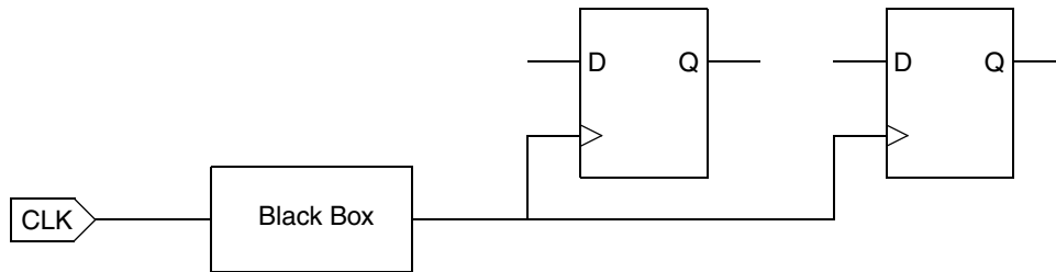
Figure 6-6 Internal Black Box in Clock Network
