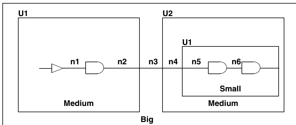
Figure 7-2 Example Design for Wire Load Mode Settings Design
