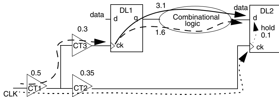
Figure 11-3 Hold Check Using Best-Case Conditions
