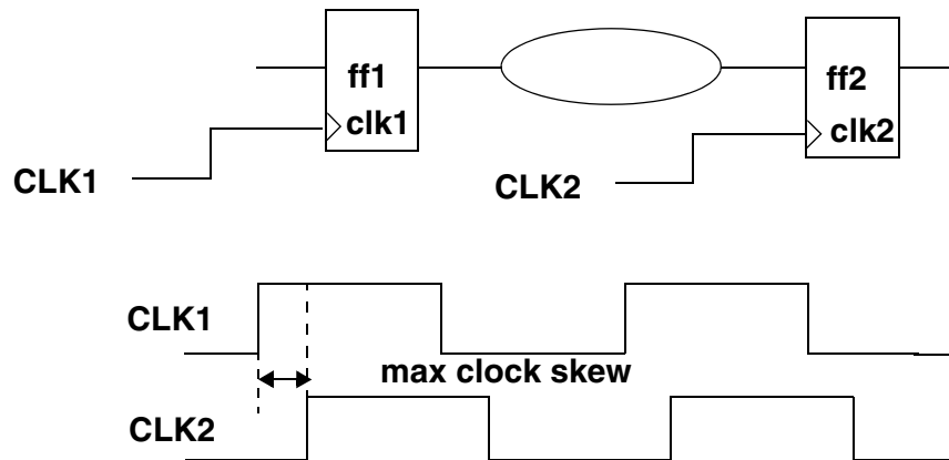
Figure 6-5 Example of Interlock Uncertainty
