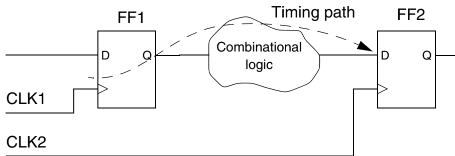
Figure 8-4 Delay Requirements With 20ns/10ns Clocks
