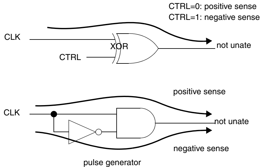
Figure 6-15 Non-Unate Clock Signals
