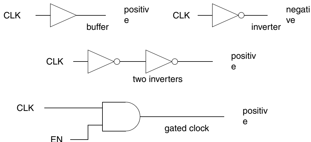
Figure 6-14 Unate Clock Signals
