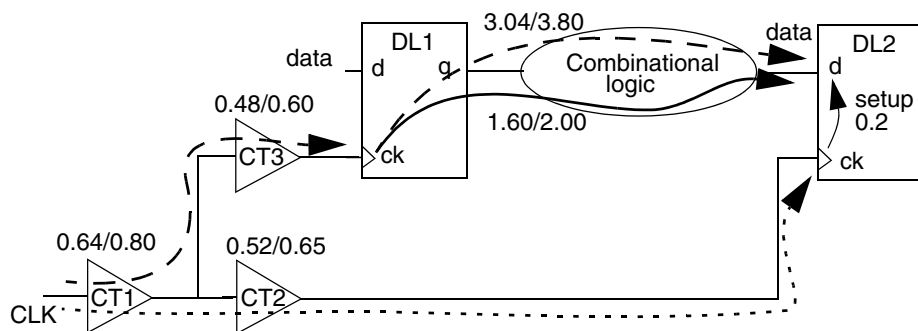
Figure 11-4 On-Chip Variation for Worst-Case Conditions
