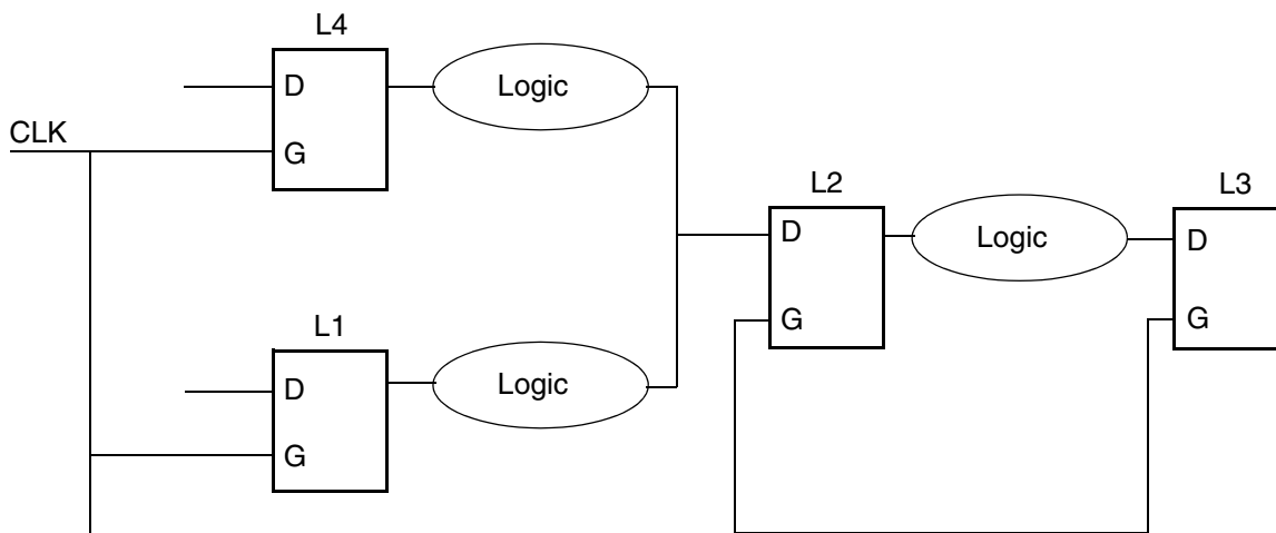
Figure 12-5 Using -exclude with -trace_latch_borrow
