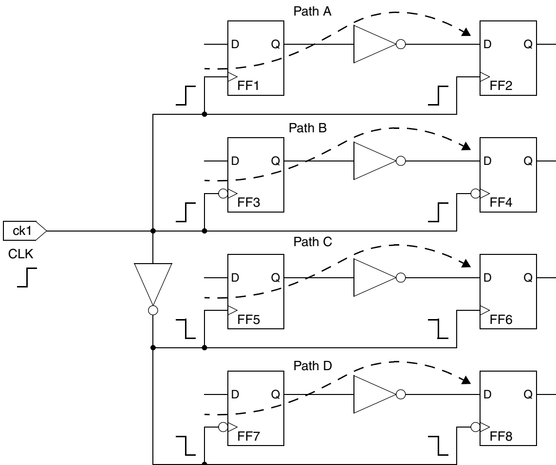
Figure 5-1 Circuit for Path Specification Examples 1 Through 3
