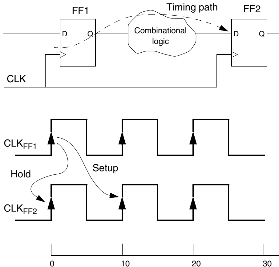
Figure 8-1 Single-Cycle Setup and Hold for Flip-Flops
