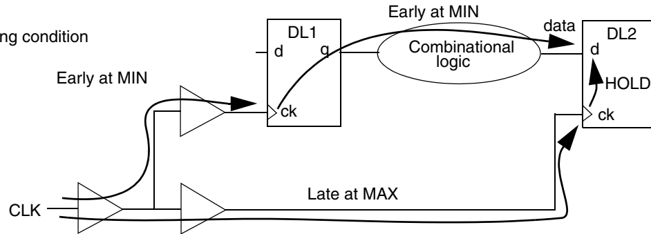
Figure 11-8 Timing Path Reported During On-Chip Variation Analysis
