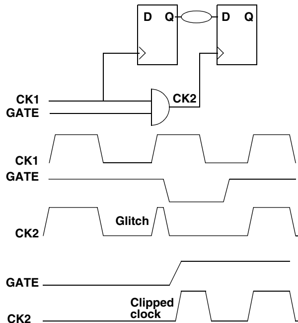
Figure 6-22 Clock-Gating Setup Violations
