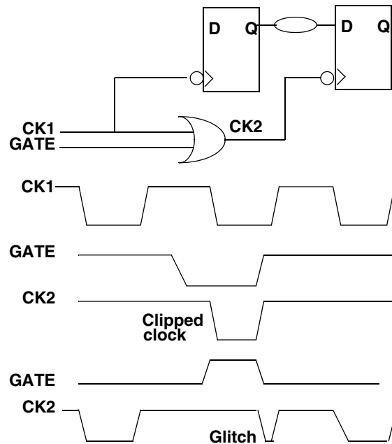
Figure 6-23 Clock-Gating Hold Violations
