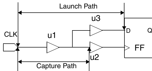
Figure 11-13 Timing Path Fanout from Clock Source to Data Pin
