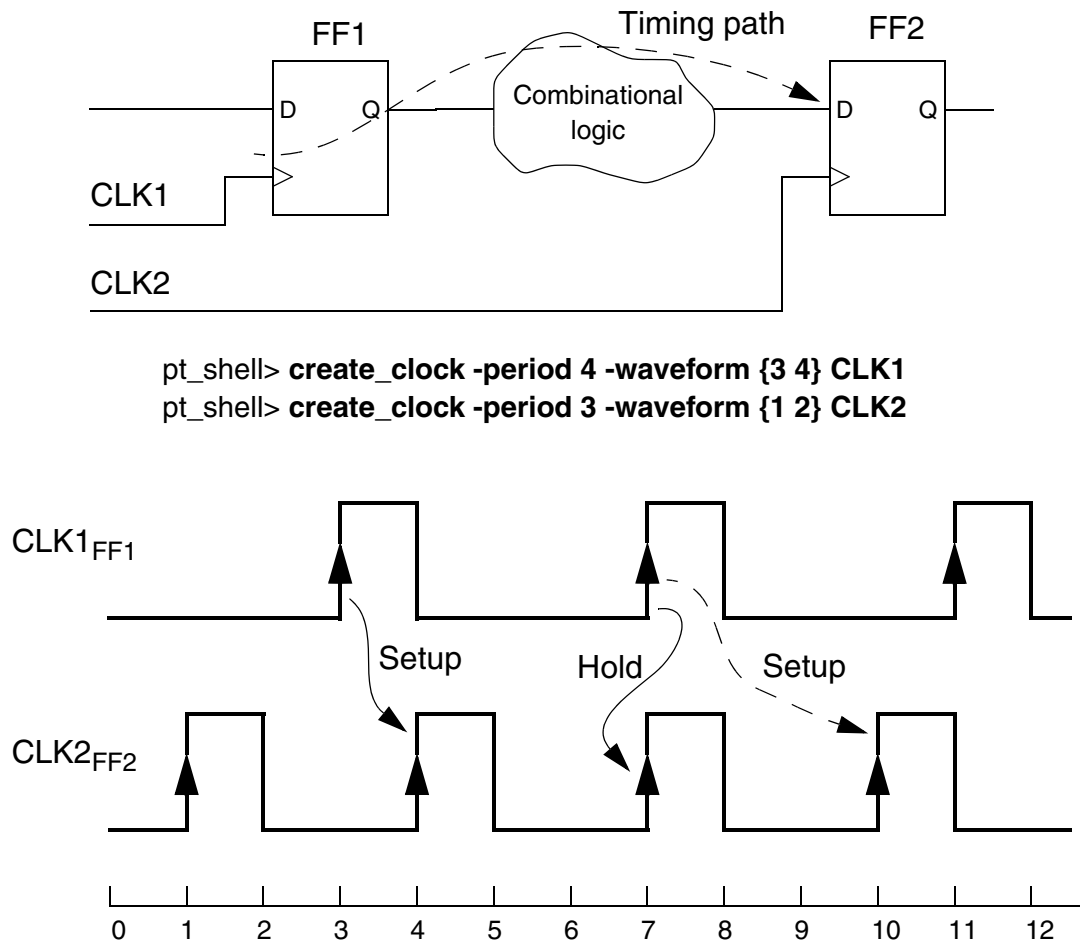
Figure 8-5 Delay Requirements With 4ns/3ns Clocks
