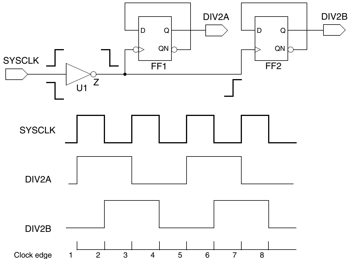
Figure 6-28 Generated Divide-by-2 Clocks Based on Different Edges
