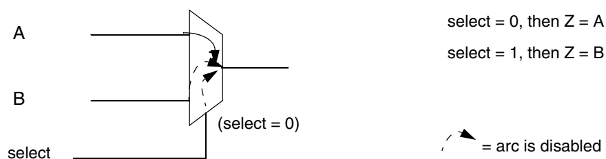
Figure 9-1 Constant Blocking of Data
