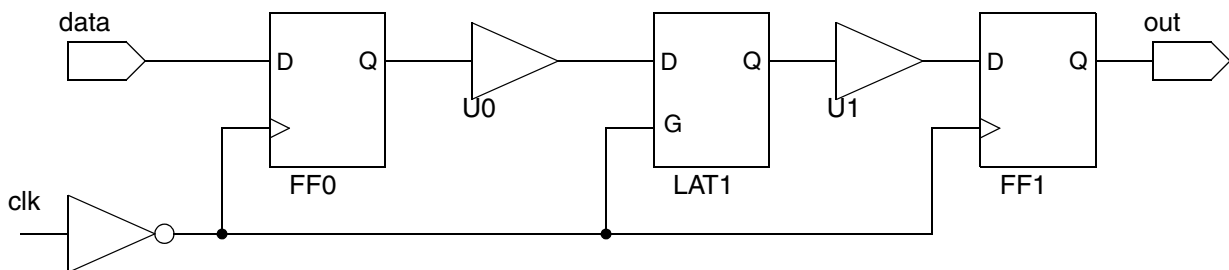
Figure 5-4 Circuit for Path Specification Example 6
