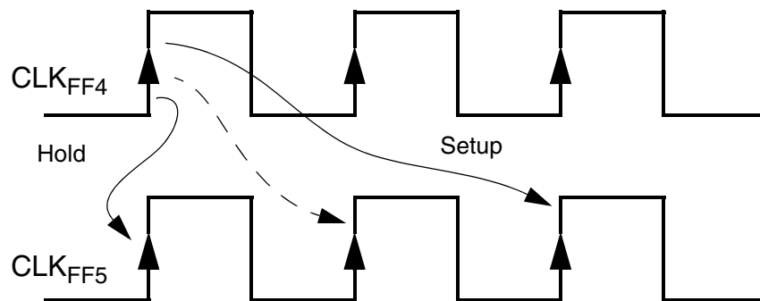
Figure 8-9 Multicycle Path Hold Set Correctly
