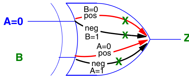
Figure 9-6 Disabled Arcs Using the when Statement
