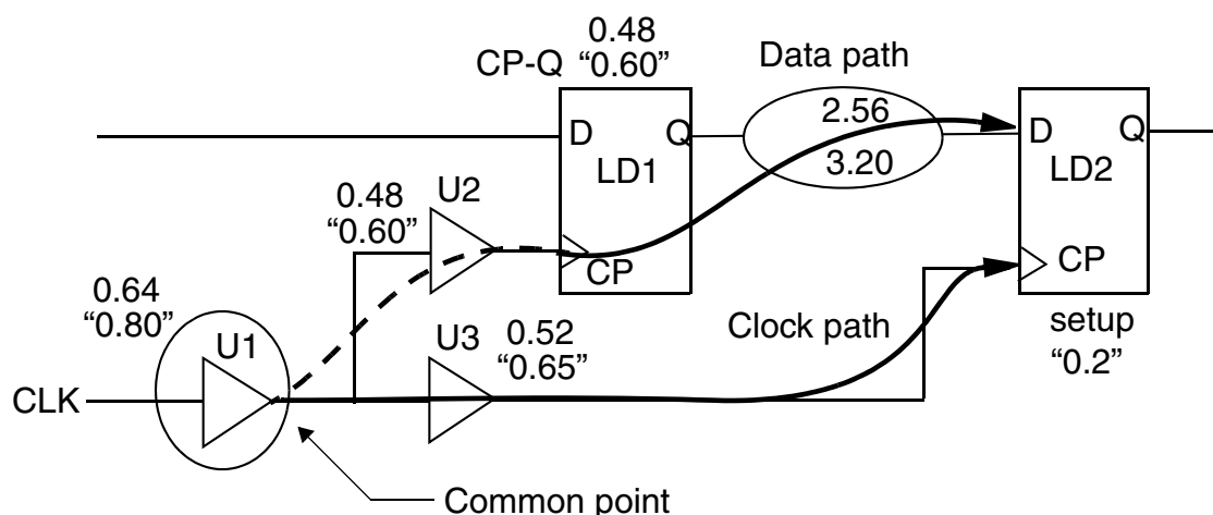
Figure 11-10 Clock Reconvergence Pessimism Example
