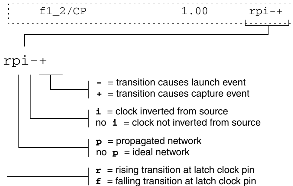
Figure 12-8 Latency, Transition Time, and Skew Condition Codes
