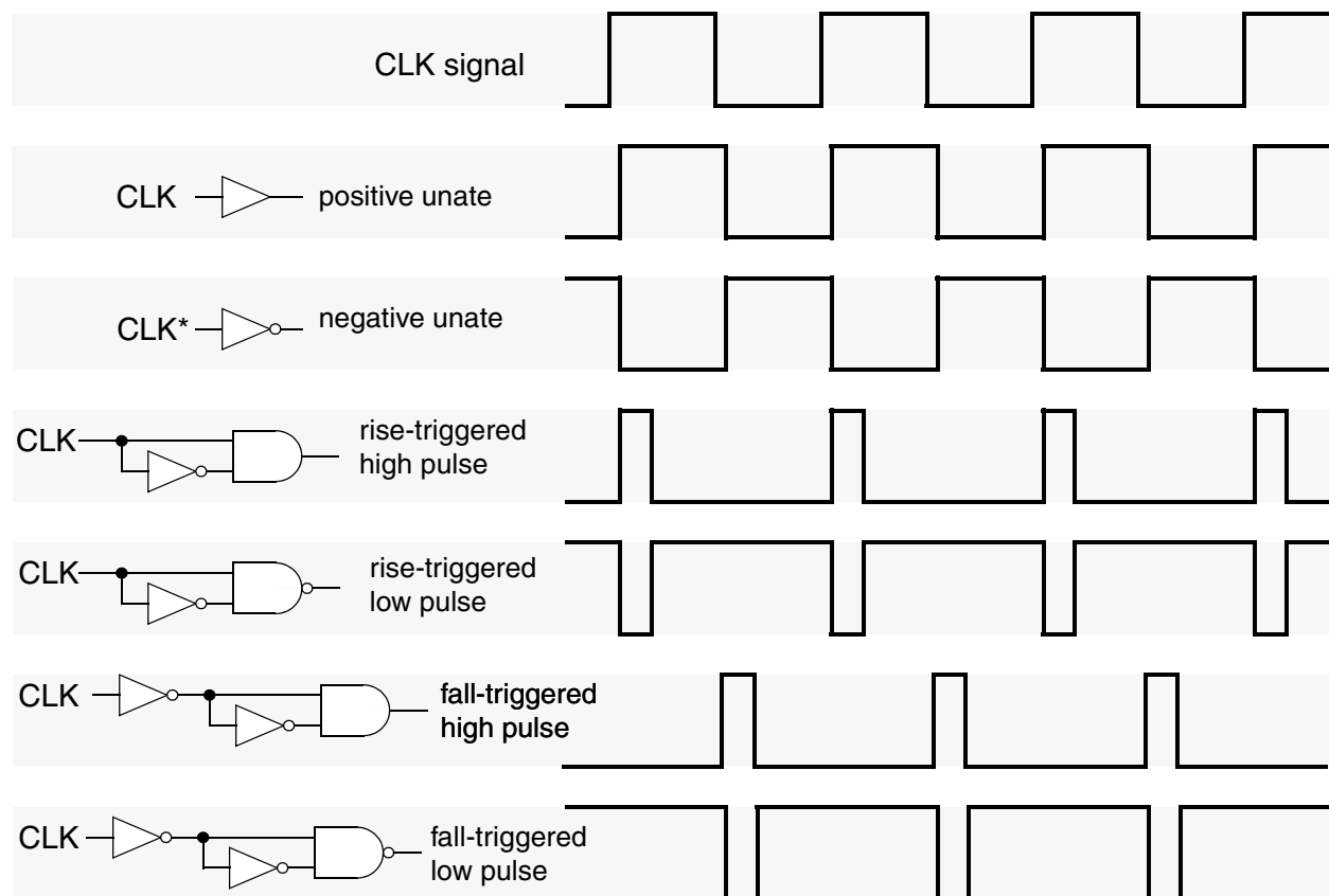
Figure 6-16 Clock Sense Examples
