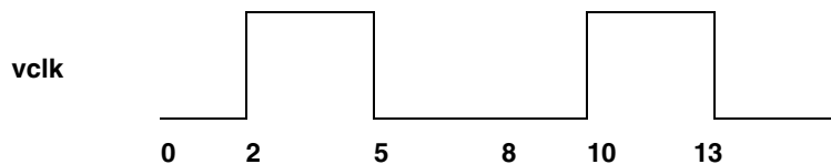
Figure 6-2 vclk Clock Waveform
