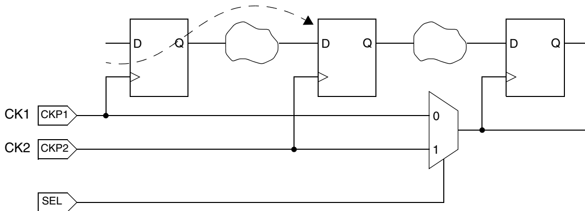
Figure 6-13 Multiplexed Clocks Specified With Case Analysis
