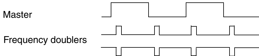
Figure 6-27 Pulse Clock Types That Change Frequency
