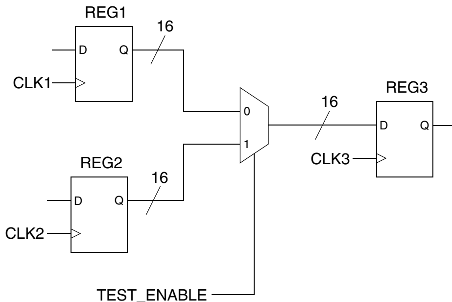
Figure 8-11 Multiplexed Register Paths
