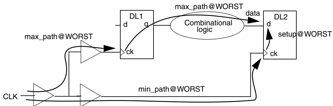
Figure 11-6 Timing Path for One Operating Condition—Worst Case
