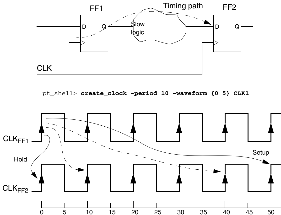
Figure 8-10 Multicycle Path Taking Five Clock Cycles
