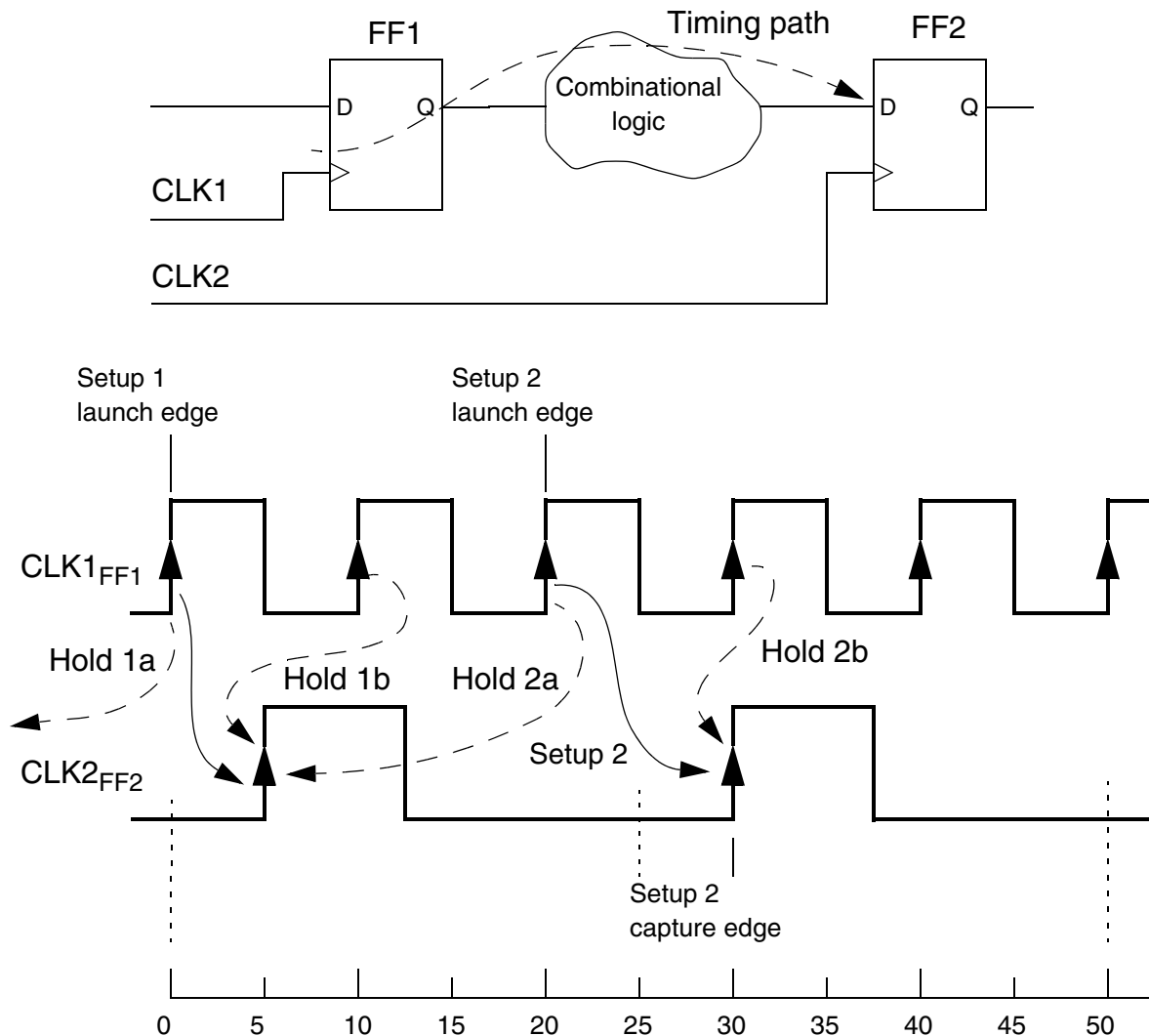
Figure 8-3 Hold Constraints for Flip-Flops With Different Clocks
