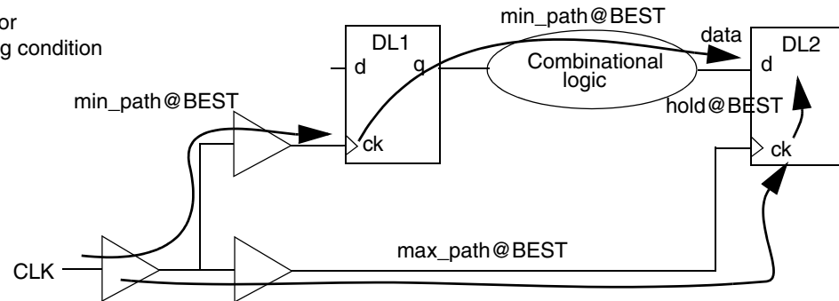
Figure 11-7 Timing Paths for Best-Case/Worst-Case Operating Conditions
