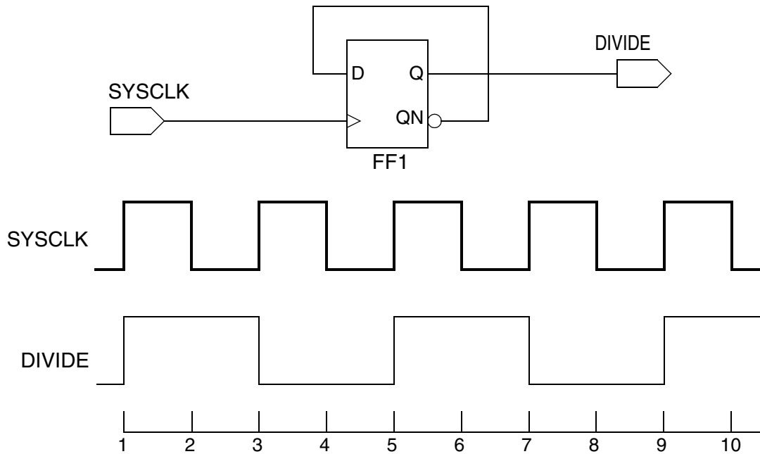
Figure 6-24 Divide-by-2 Clock Generator
