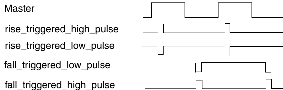
Figure 6-26 Pulse Clock Types That Do Not Change Frequency
