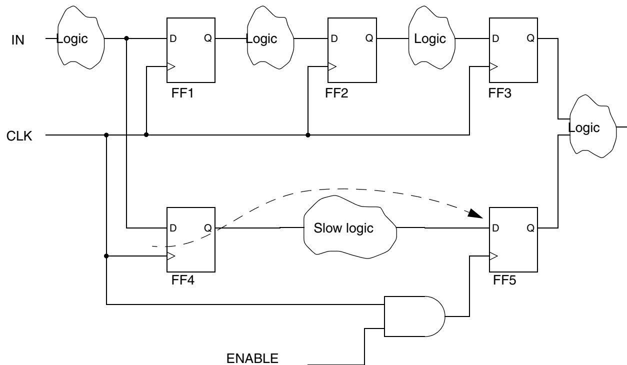
Figure 8-6 Multicycle Path Example
