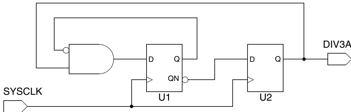
Figure 6-25 Divide-by-3 Clock Generator
