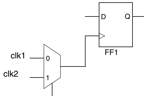
Figure 5-6 Circuit for Path Specification Example 8
