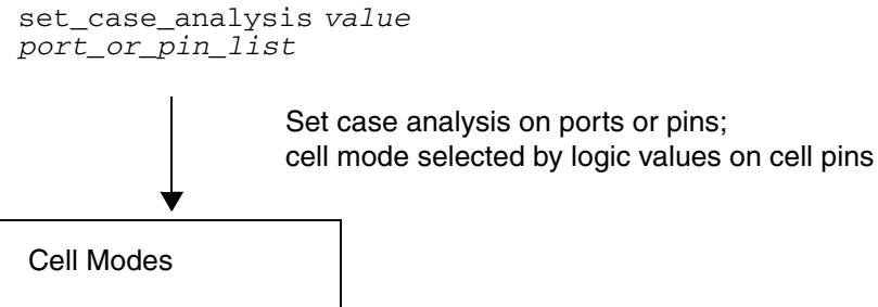
Figure 10-3 Selecting Modes Using Case Analysis
