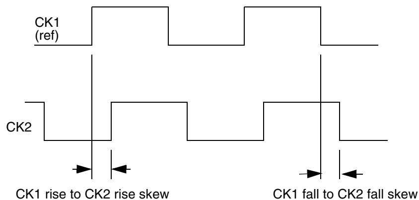
Figure 12-9 Timing Diagram for Skew Constraint
