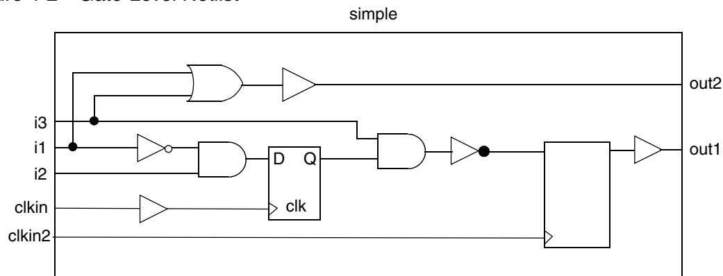
Figure 4-2 Gate-Level Netlist
