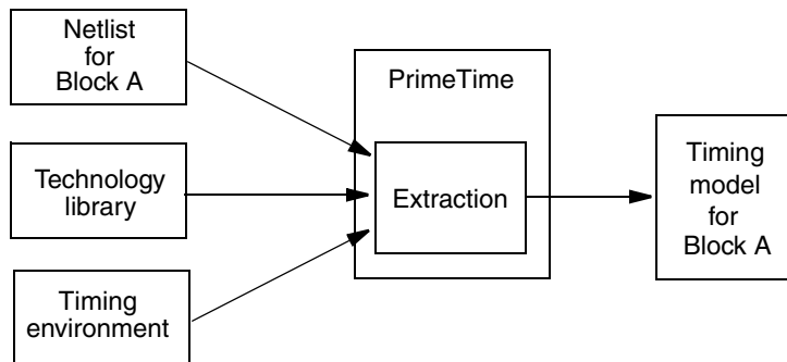
Figure 4-1 Extraction Process
