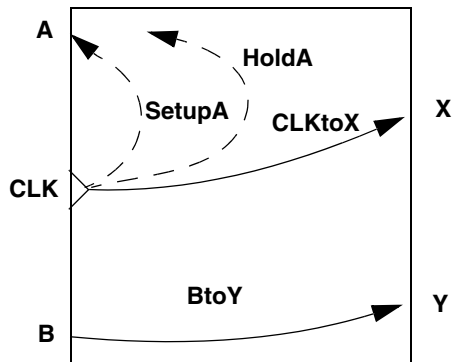
Figure 2-3 Quick Timing Model Representation of a Block
