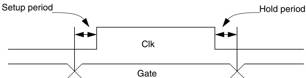
Figure 4-15 No-Change Arc
