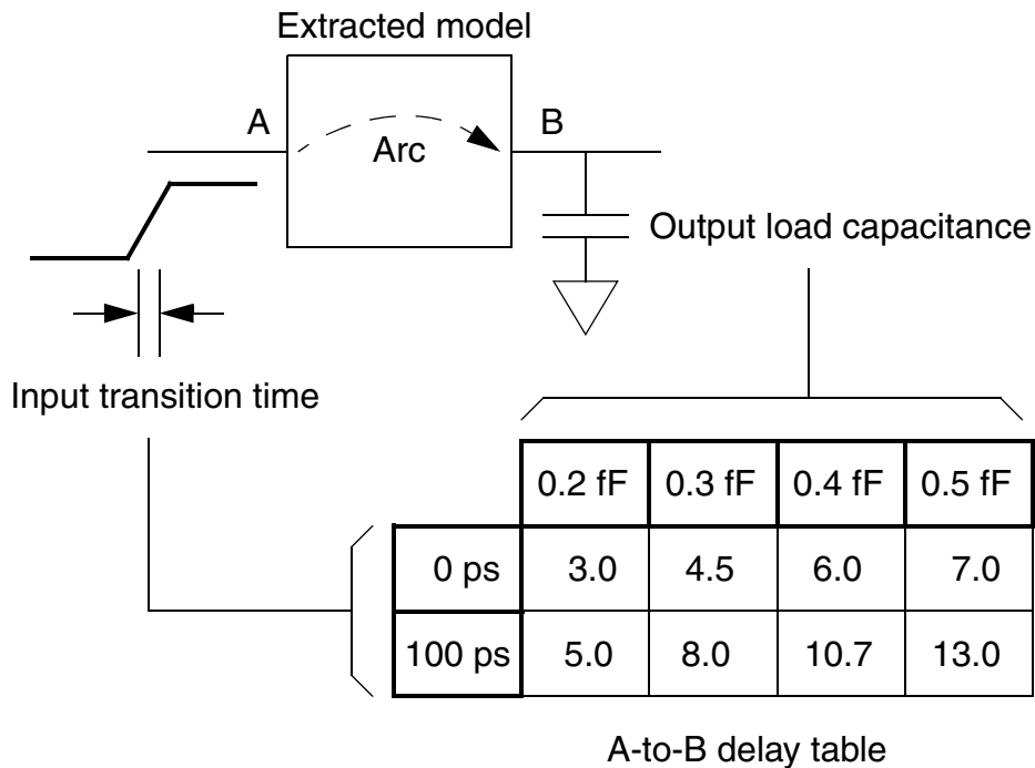
Figure 4-8 Delay Table Example
