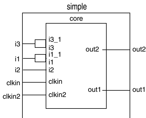
Figure 4-3 Netlist of Extracted Model
