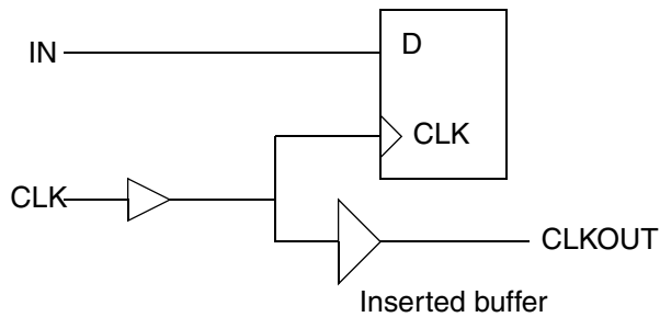
Figure 4-7 Isolating the Delay of the Clock Network
