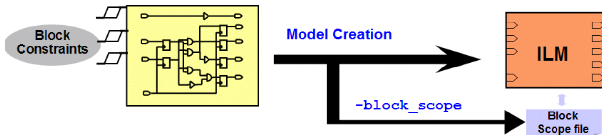
Figure 3-3 Checking the Block Level Scope
