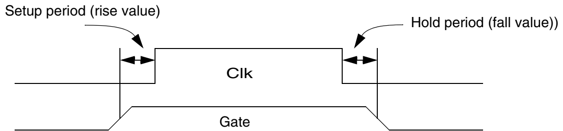
Figure 4-16 NOCHANGE_HIGH_HIGH Arc
