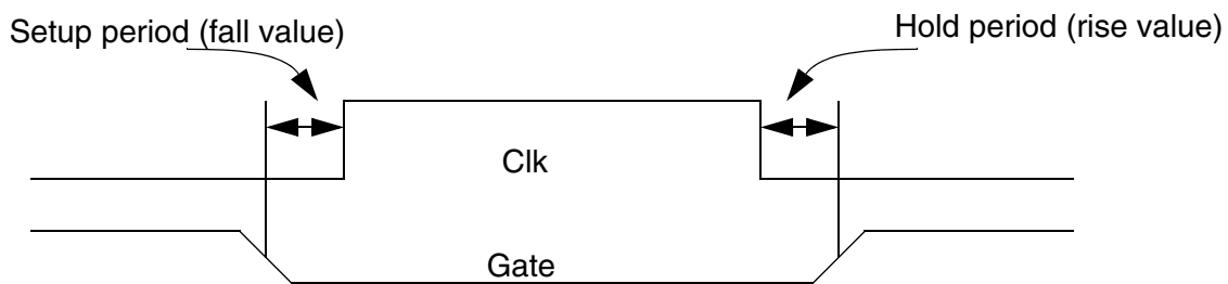
Figure 4-17 NOCHANGE_LOW_HIGH Arc
