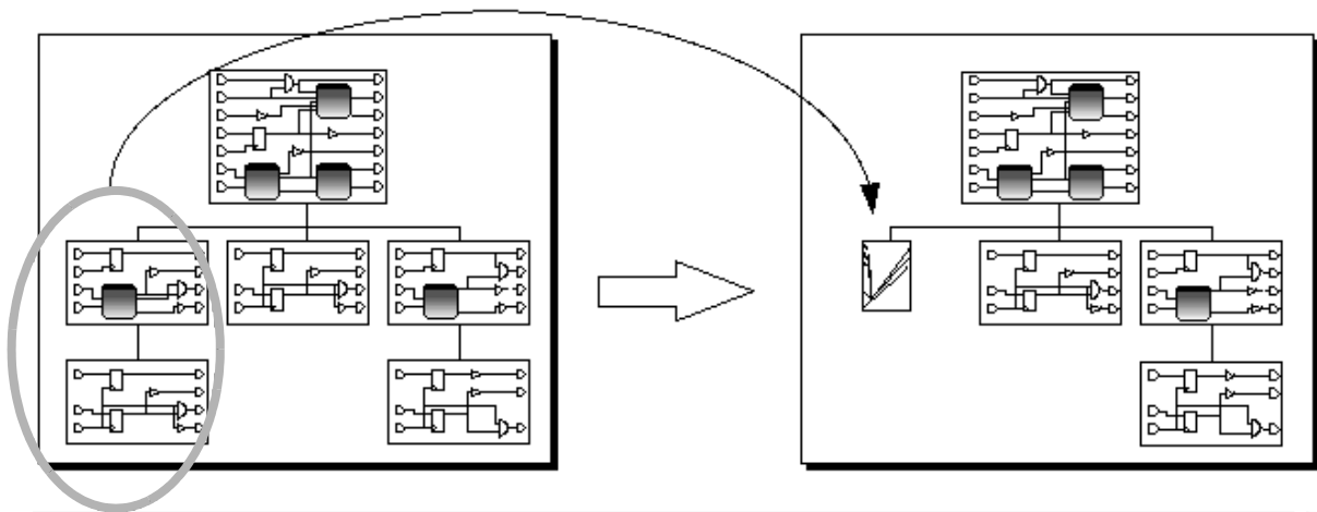
Figure 1-5 Extracted Model of a Bottom-Up Design
