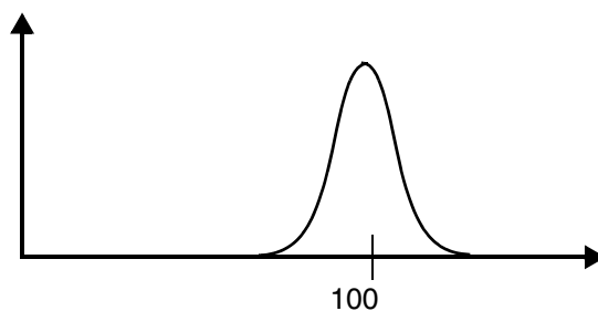
Figure 3-1 PDF Plot of Normal Distribution
