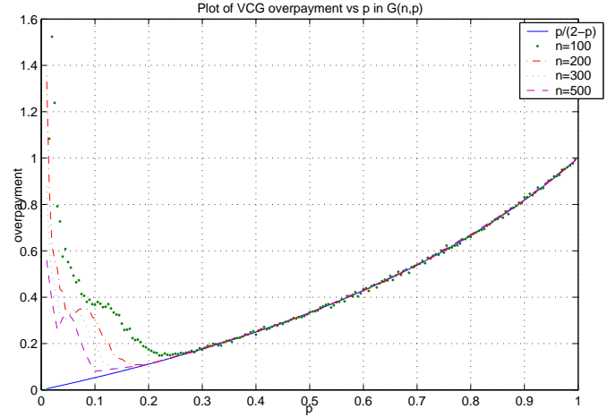
Fig. 1. Average overpayment in G(n, p) .
