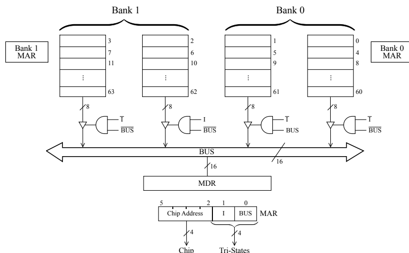
Figure 6.6: Two-way Interleaving
