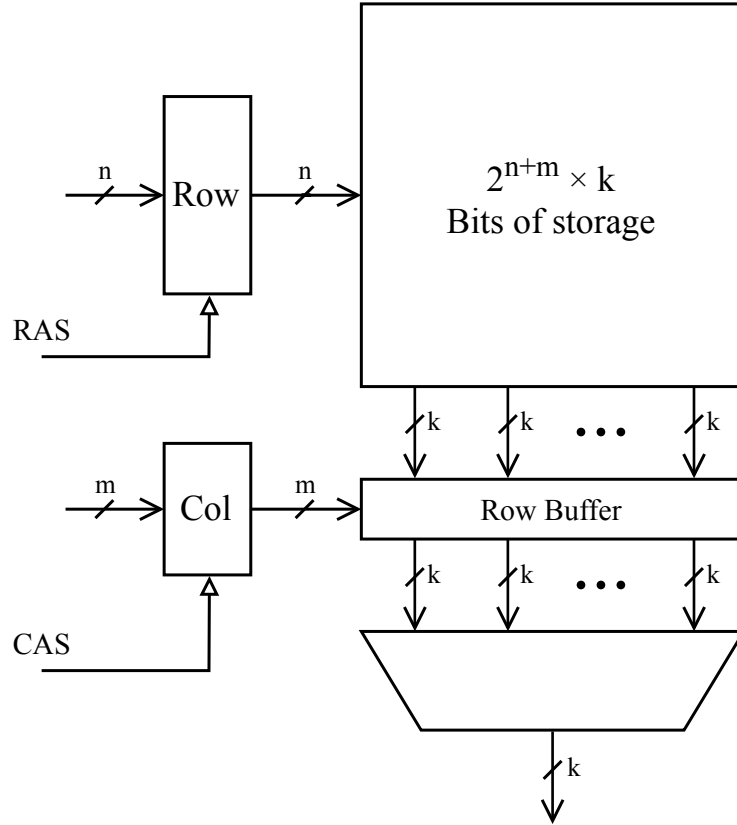
Figure 6.11: The DRAM Array
